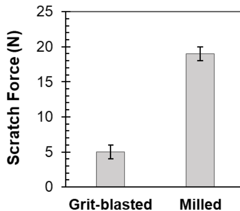
Fig. 5. Scratch resistance in the grit-blasted and milled surfaces after anodizing.
