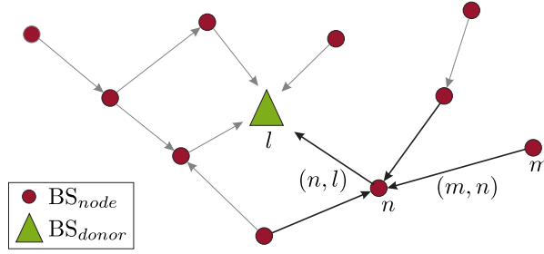
Figure 3.11: Example of a graph \mathcal{G}_i
