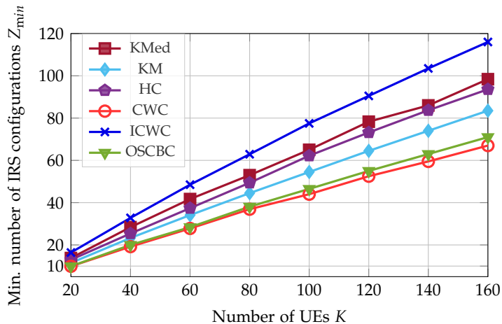
Figure 4.12: Minimum number of IRS configurations (clusters) Z_{min} to achieve 80% of the maximum achievable sum capacity, for an unquantized 40H \times 80V IRS, and considering a pLoS channel for the IRS-UEs links.
