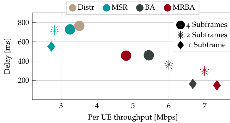
(a) Combined per UE end-to-end throughput first quartile and delay third quartile, as a function of the semi-centralized allocation period T_{alloc} .
