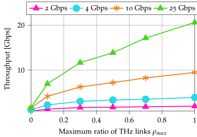
Figure 3.29: System throughput for different source rate and ratio of THz links.
