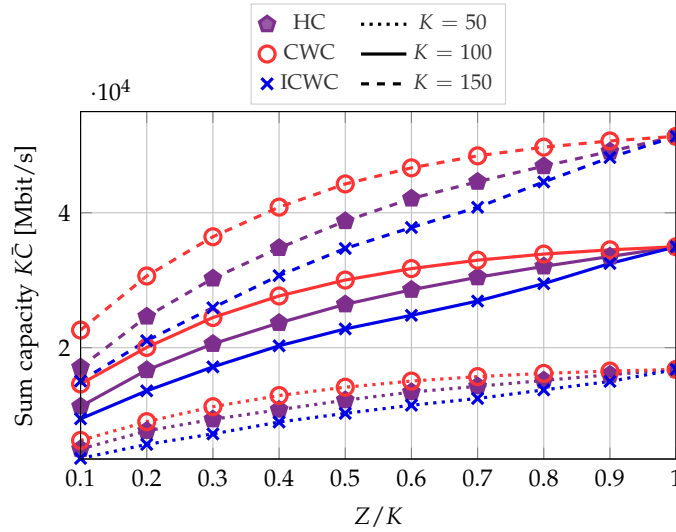
Figure 4.10: Sum capacity as a function of the maximum number of clusters over the number of UEs Z/K , for different values of K , for an unquantized 40\text{H}\times 80\text{V} IRS, K = \{50, 100, 150\} , and considering a pLoS channel for the IRS-UEs links. For readability, the results are shown without averaging over the TDMA frame length.
