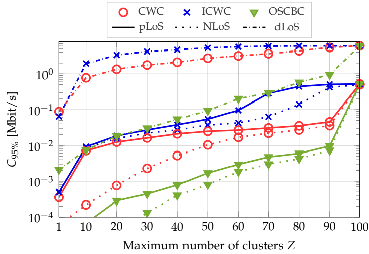
Figure 4.5: 95% percentile of the user capacity as a function of the maximum number of clusters Z , for N_I = 3200 , unquantized phase shifts, and for different channel conditions.
