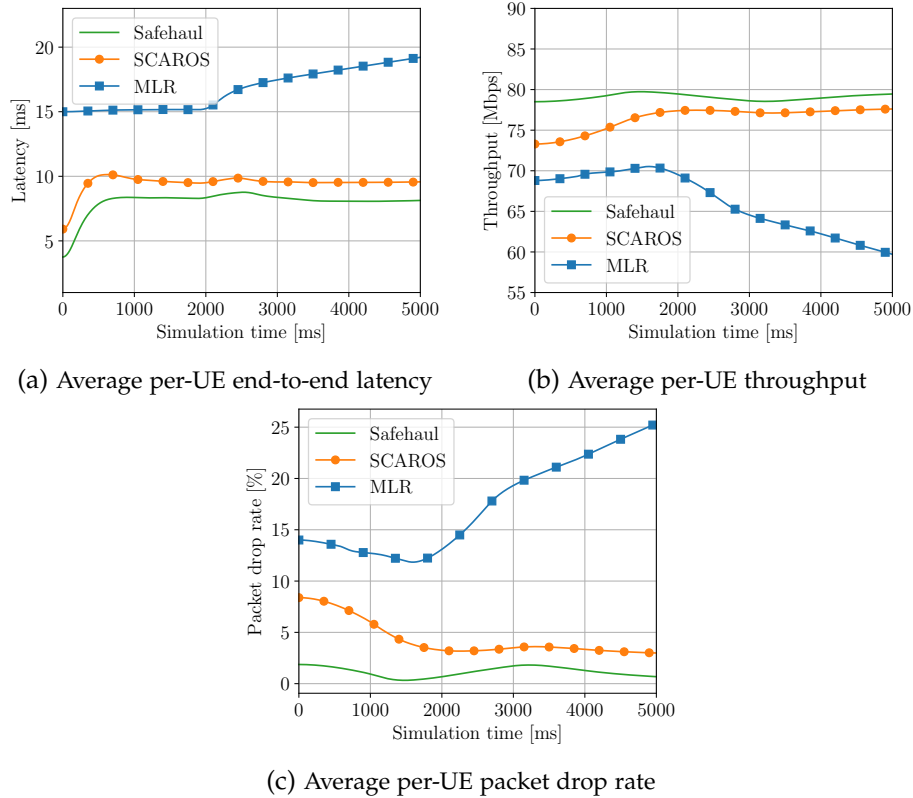
Figure 3.22: Average network performance for 50 UEs and 80 Mbps per-UE source rate where 1 random BS-node is shut down.
