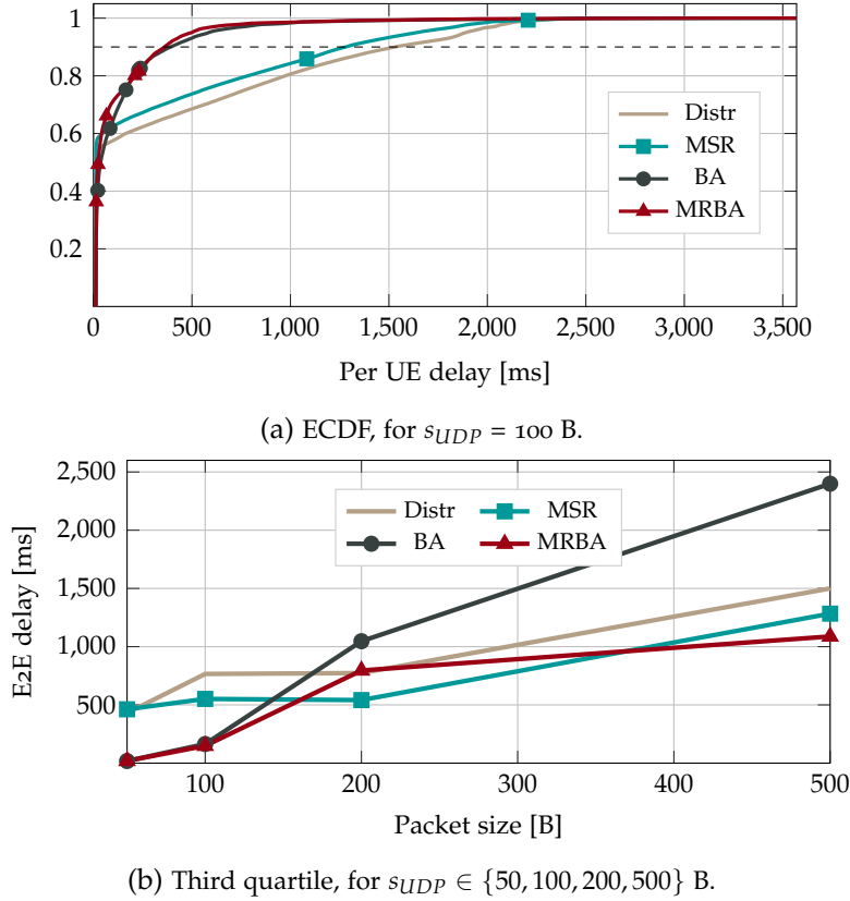
Figure 3.7: Per-UE end-to-end delay statistics.
