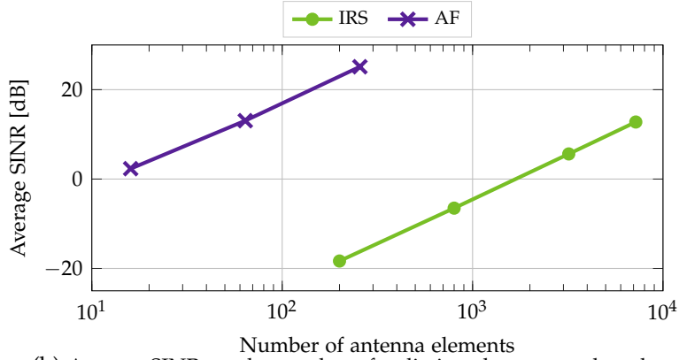
(b) Average SINR vs. the number of radiating elements at the relay.
