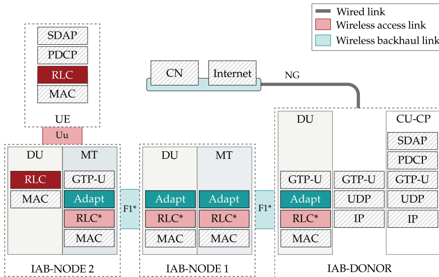
(a) IAB protocol stack and topology.
