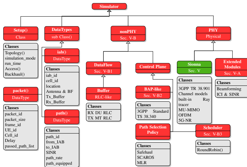
Figure 3.13: Overall design of our Sionna's extension. The red blocks represent our additions to the baseline simulator, i.e., Sionna [146].
