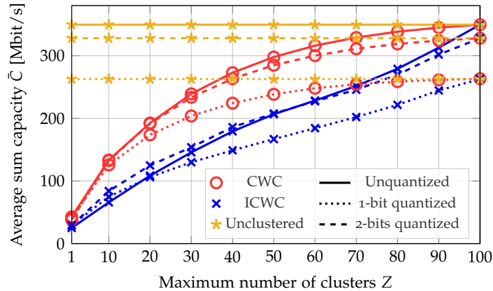
Figure 4.8: Average sum capacity as a function of the maximum number of clusters Z , for N_I = 3200 and for different degrees of quantization of the phase shifts, and considering a pLoS channel for the IRS-UEs links.
