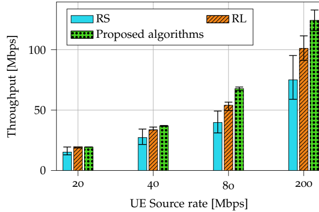
Figure 3.25: Throughput per UE for different schedulers and THz link selection policies, for THz bandwidth 32 GHz and \rho_{max} = 0.3 .
