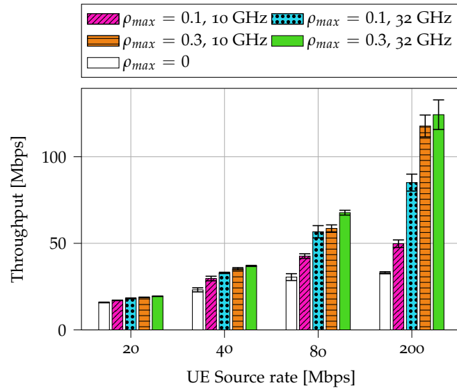
Figure 3.26: Throughput per UE for different configurations.
