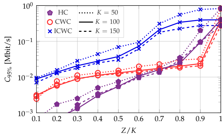
Figure 4.11: 95% of the user capacity as a function of the maximum number of clusters over the number of UEs Z/K , for different values of K , for an unquantized 40\text{H}\times 80\text{V} IRS, K = \{50, 100, 150\} UEs, and considering a pLoS channel for the IRS-UEs links.
