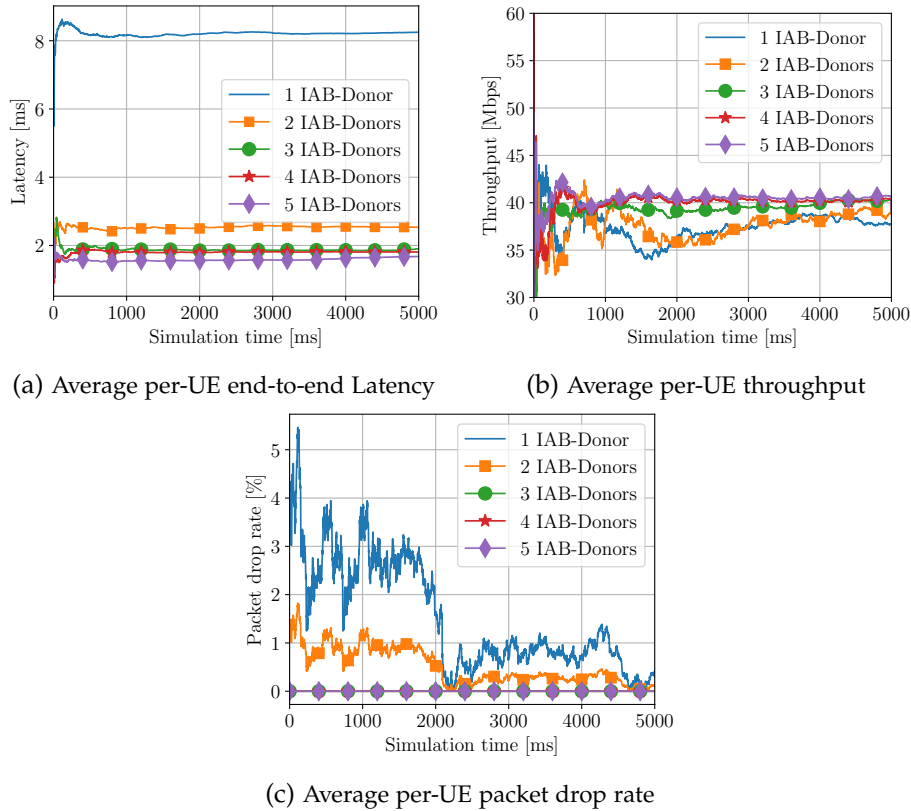
Figure 3.21: Network performance for 50 UEs and 40 Mbps per-UE source rate, versus the number of BS-donors in Padova (Scenario 3).
