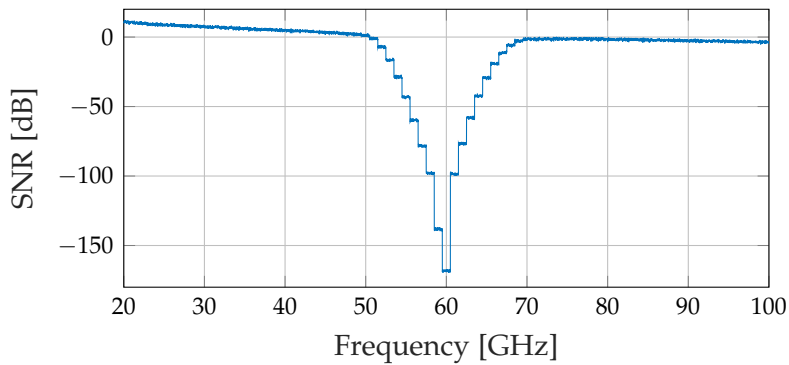
Figure 2.8: The SNR for different carrier frequencies. We consider a GEO satellite, with the parameters in Tab. 2.3.
