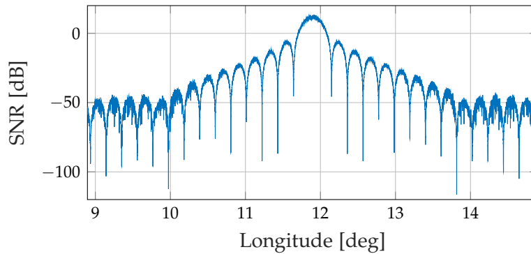
Figure 2.9: The SNR for different angular positions of a GEO satellite, with the parameters in Tab. 2.3.
