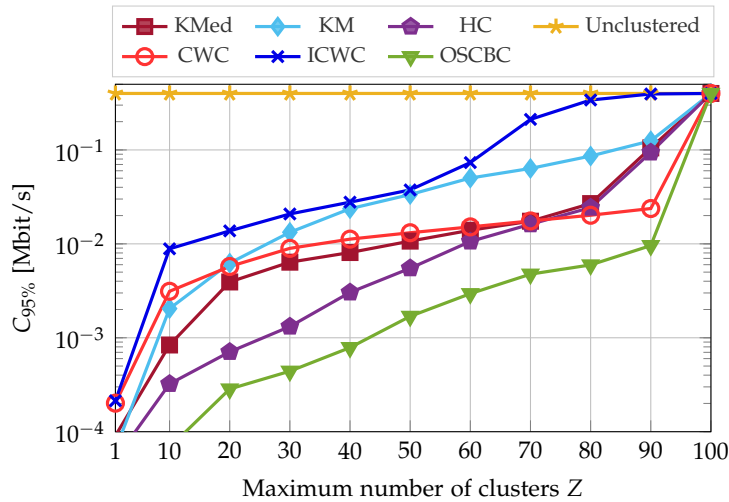
Figure 4.3: 95% percentile of the user capacity as a function of the maximum number of clusters Z , for an unquantized 40H \times 80V IRS, and considering a pLoS channel for the IRS-UEs links.
