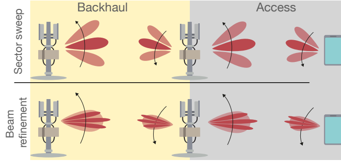
Figure 3.12: Schematic of the hierarchical beam management procedure. First, the general direction is estimated using wide beams (top). Then, the search is refined using the narrow beams codebook.
