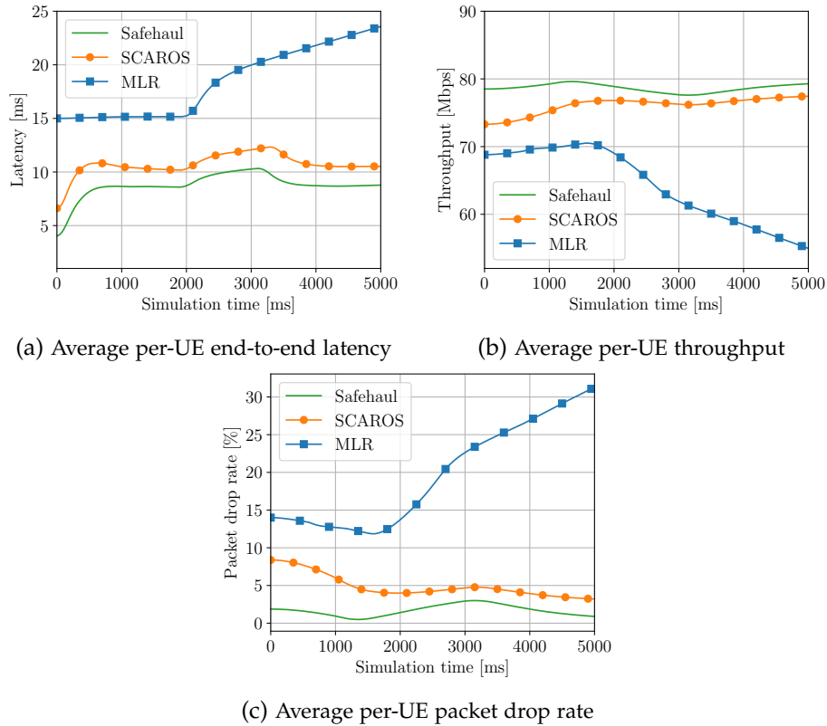
Figure 3.23: Average network performance for 50 UEs and 80 Mbps per-UE source rate where 3 random BS-nodes are shut down.
