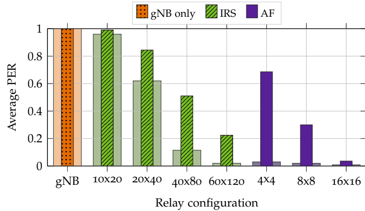
Figure 2.6: Average PER at the application layer in Scenario 1 (wide bars) and Scenario 2 (narrow bars) for different relay configurations.
