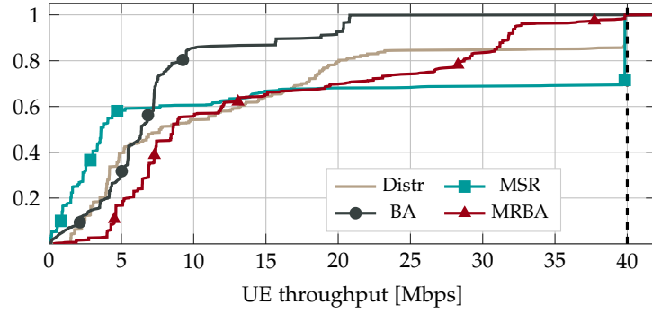
(b) s_{UDP} = 500 B, i.e., UDP rate of 40 Mbps.
