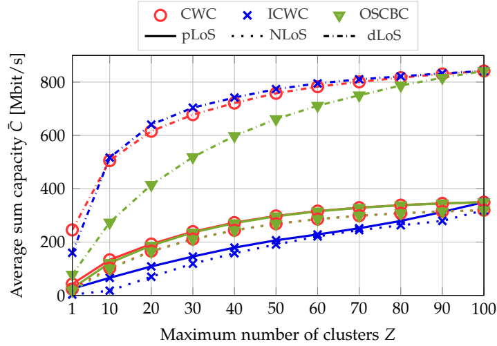
Figure 4.4: Average sum capacity as a function of the maximum number of clusters Z , for N_I = 3200 , unquantized phase shifts, and for different channel conditions.
