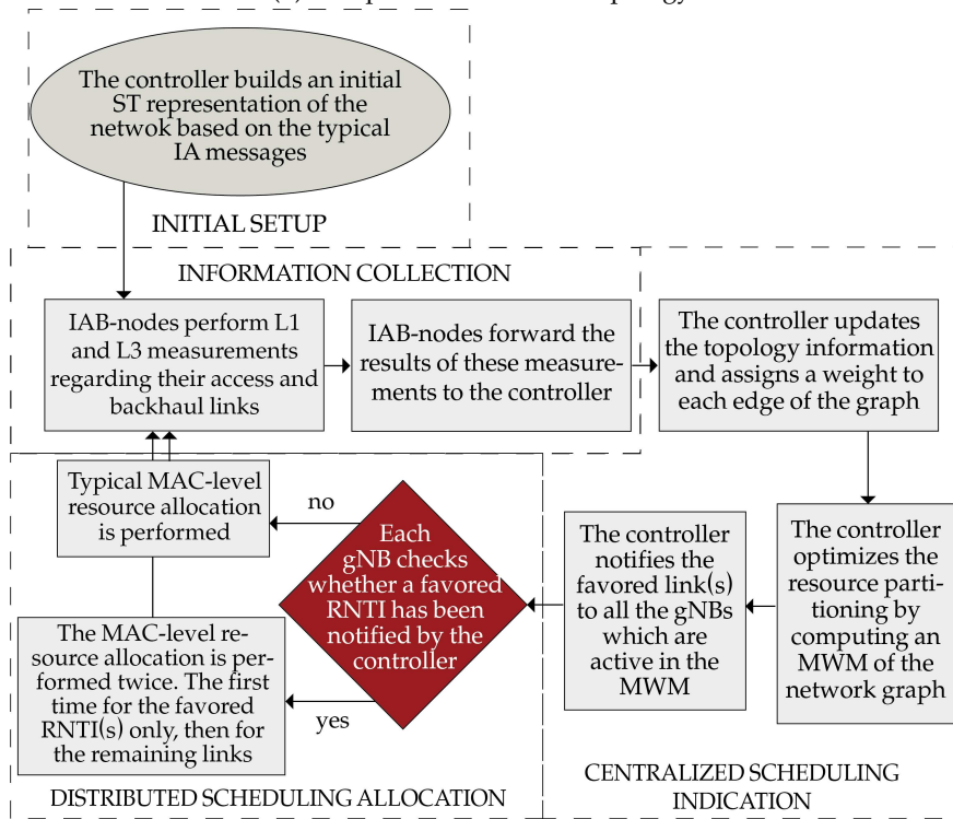
(b) High level diagram of the proposed MWM-based framework.
