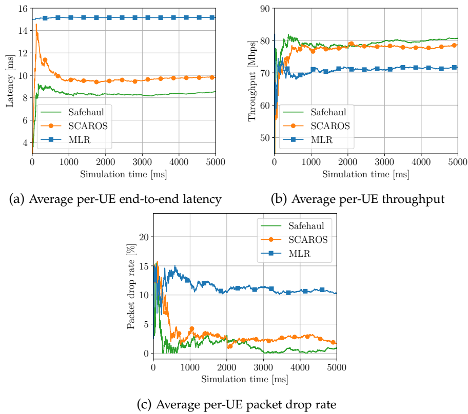
Figure 3.15: Average network performance for 50 UEs and 80 Mbps per-UE source rate (Scenario 1).
