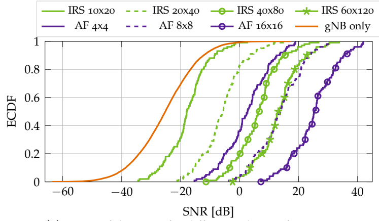
(a) ECDF of the SINR for different relay configurations.
