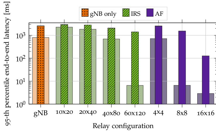
Figure 2.5: 95-th percentile of the end-to-end latency at the application layer in Scenario 1 (wide bars) and Scenario 2 (narrow bars) for different relay configurations.
