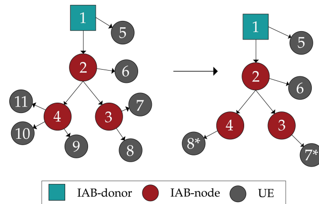
(a) The original topology, exhibiting the actual cell attachments, is depicted on the left. Conversely, the reduced one is shown on the right.
