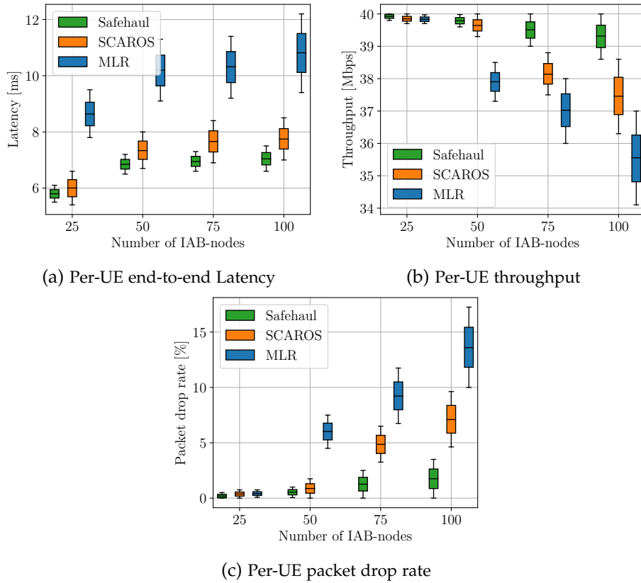
Figure 3.20: Network performance for \{25, 50, 75, 100\} BS-nodes, 2 UEs per BS-node on average, and 40 Mbps per-UE source rate (Scenario 2) in Padova.
