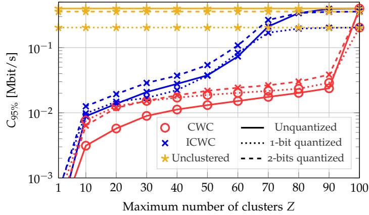
Figure 4.9: 95% percentile of the user capacity as a function of the maximum number of clusters Z , for N_I = 3200 and for different degrees of quantization of the phase shifts, and considering a pLoS channel for the IRS-UEs links.
