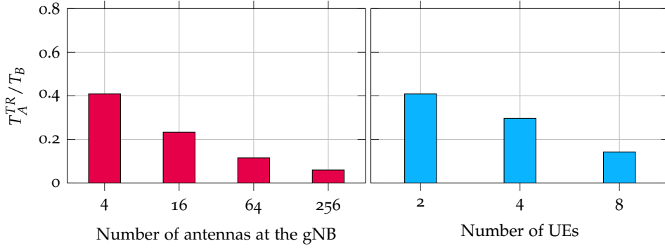
Figure 2.14: Ratio of the median simulation times using the performance-oriented channel model presented in this work ( T_A^{TR} ) and the 3GPP channel model of [46] after the merge of this work. In this case, Eigen is disabled.
