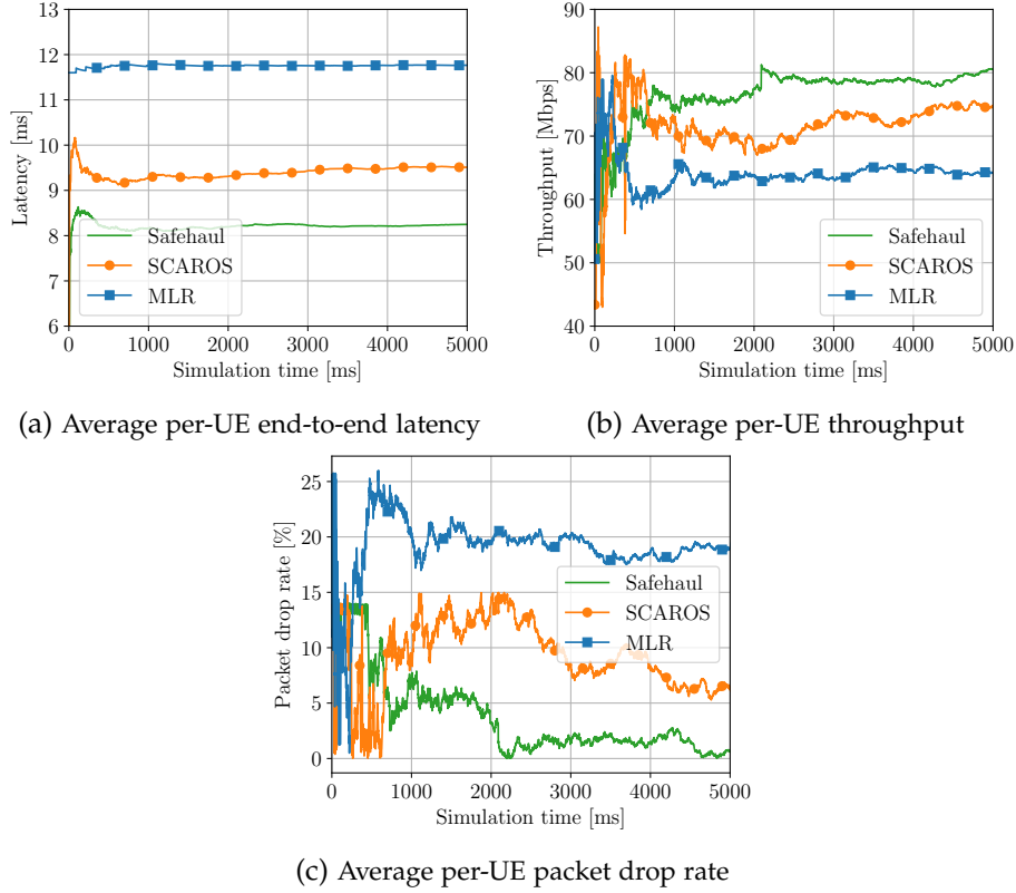
Figure 3.19: Average network performance for 50 UEs and 80 Mbps per-UE source rate (Scenario 1) in Padova.
