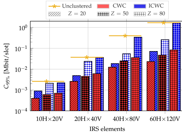
Figure 4.7: 95% percentile of the user capacity for CWC and ICWC as a function of the number of reflecting elements at the IRS, for unquantized phase shifts, and considering a pLoS channel for the IRS-UEs links.
