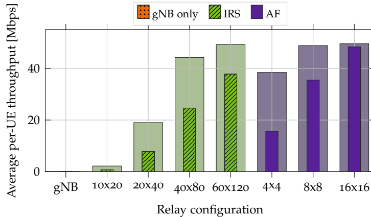
Figure 2.4: End-to-end per-UE throughput at the application layer in Scenario 1 (wide bars) and Scenario 2 (narrow bars) for different relay configurations.
