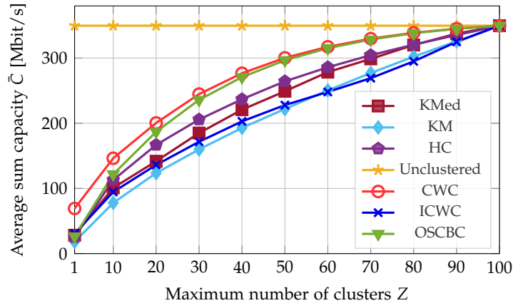
Figure 4.2: Average sum capacity as a function of the maximum number of clusters Z , for an unquantized 40\text{H} \times 80\text{V} IRS, and considering a pLoS channel for the IRS-UEs links.
