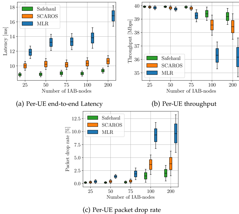
Figure 3.16: Network performance for \{25, 50, 75, 100, 200\} BS-nodes, 2 UEs per BS-nodes on average, and 40 Mbps per-UE source rate (Scenario 2).
