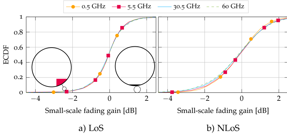
Figure 2.12: Small-scale fading gain statistics for the UMi propagation scenario versus the carrier frequency f_C , for both LoS and NLoS channel conditions.
