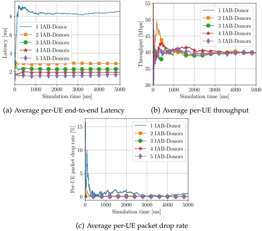
Figure 3.17: Network performance for 50 UEs and 40 Mbps per-UE source rate, versus the number of BS-donors (Scenario 3).
