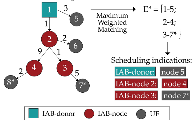
(b) Computation of the MWM and of the corresponding scheduling indications.
