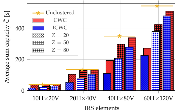
Figure 4.6: Average sum capacity for CWC and ICWC as a function of the number of reflecting elements at the IRS, for unquantized phase shifts, and considering a pLoS channel for the IRS-UEs links.
