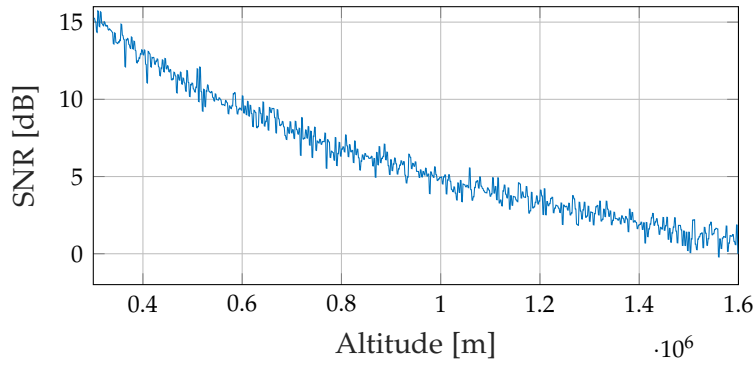
Figure 2.10: The SNR for different values of the altitude of a LEO satellite, with the parameters in Tab. 2.3.
