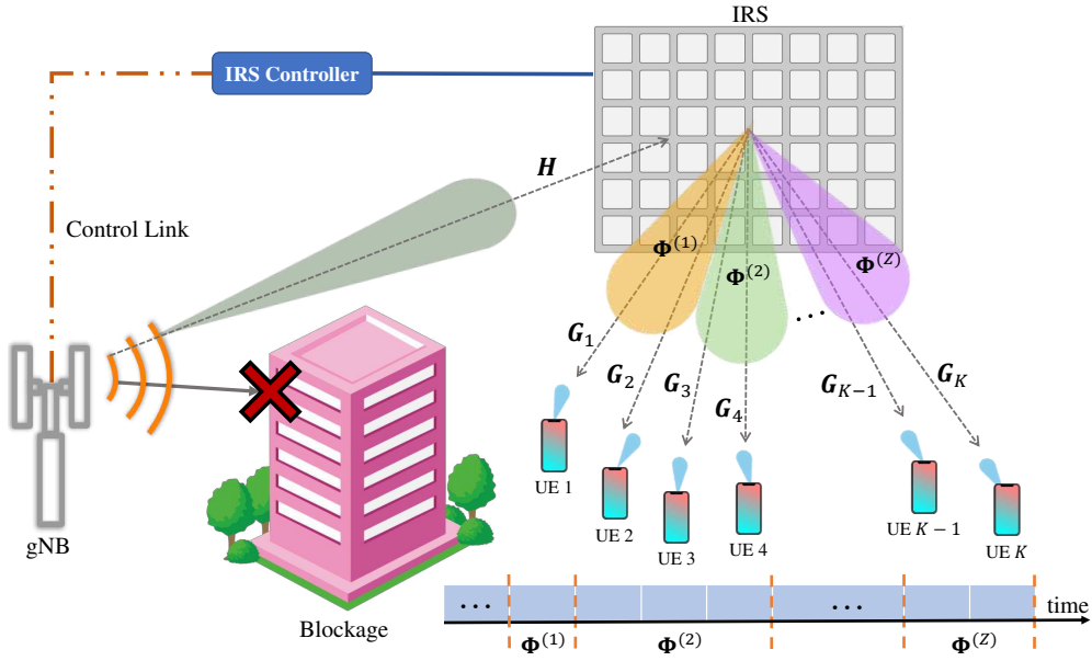
Figure 4.1: Downlink TDMA scheduling for multi-user IRS-aided systems.
