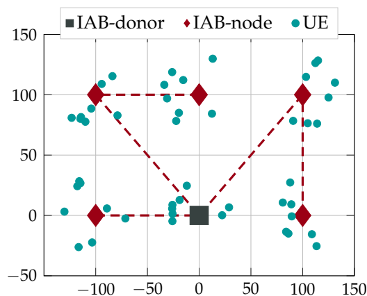
(a) A realization of the simulation scenario; the dotted lines represent the cell-attachments of the IAB-nodes.
