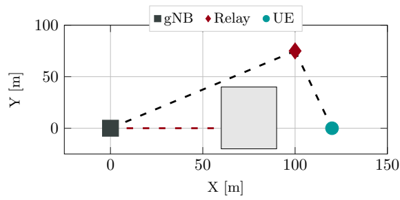
(a) Scenario 1, with N_U = 1 .
