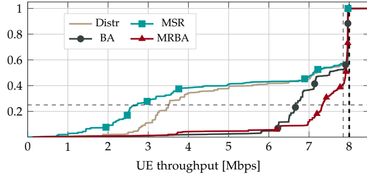
(a) s_{UDP} = 100 B, i.e., UDP rate of 8 Mbps.
