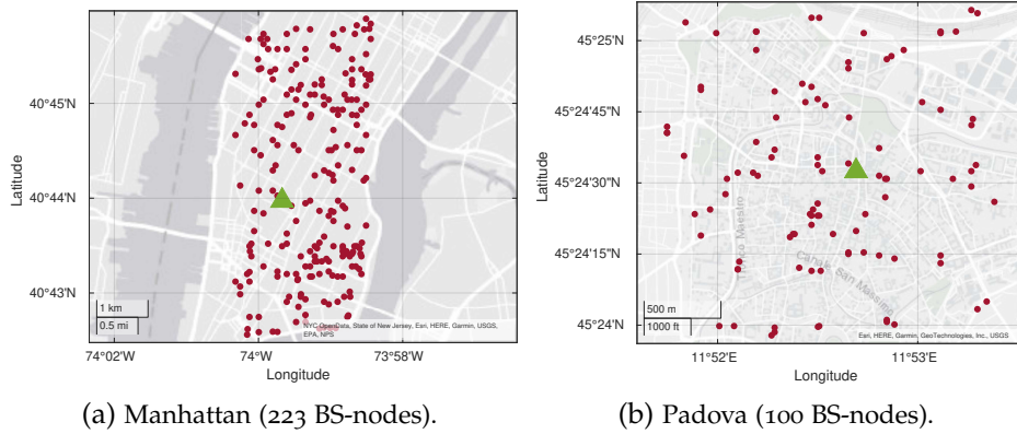
Figure 3.14: Locations of BS-nodes (red dots) and of the BS-donor (green triangle) in the Manhattan (left) and Padova (right) topologies.
