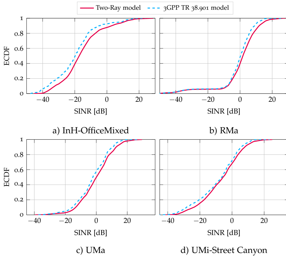
Figure 2.15: ECDF of the SINR obtained using the 3GPP channel model of [46], and the performance-oriented channel model presented in this work, for different propagation scenarios.
