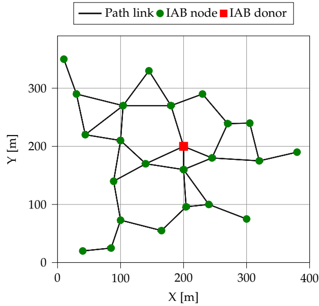
Figure 3.24: Simulation Scenario
