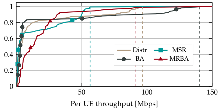
(b) Throughput ECDF.
