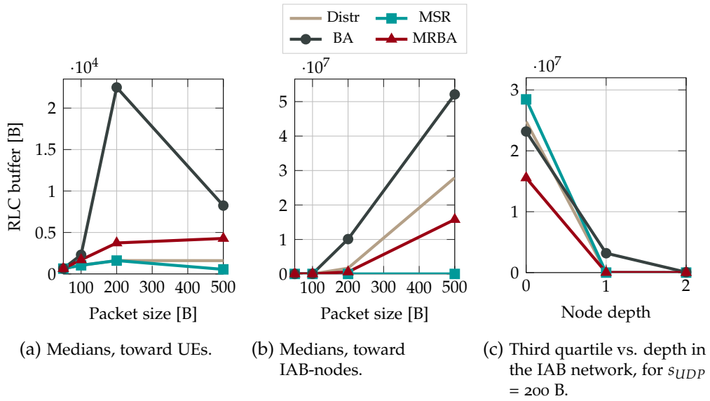
Figure 3.8: Buffer occupancy statistics, for s_{UDP} \in \{50, 100, 200, 500\} B.
