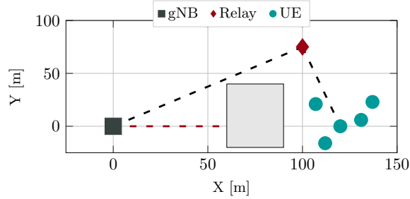
(b) Scenario 2, with N_U = 5 .
