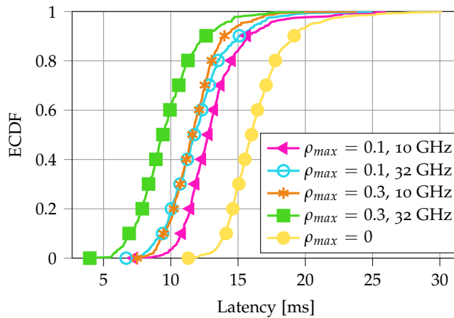
Figure 3.28: E2E latency ECDF for different configurations for 80 Mbps user rate.
