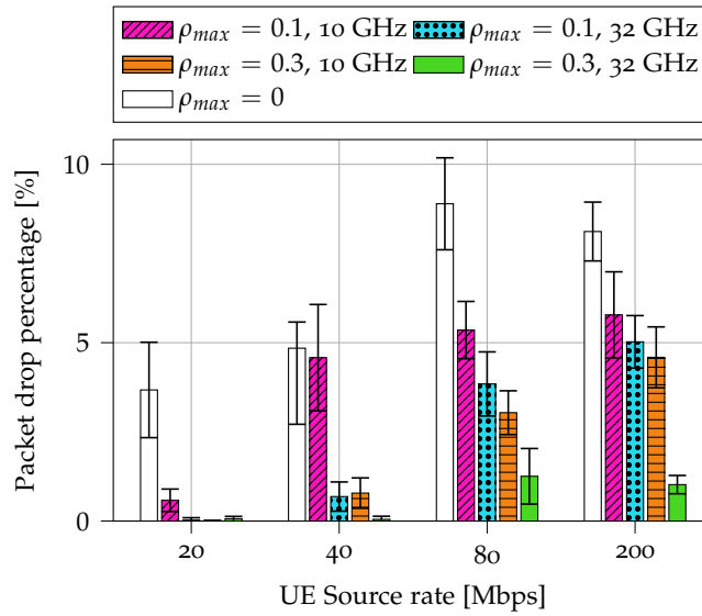
Figure 3.27: Backhaul packet drop percentage for different configurations.
