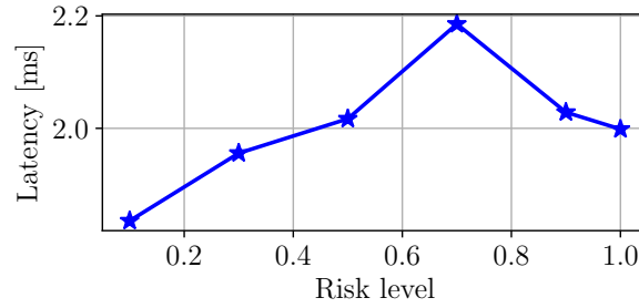
Figure 3.18: Average latency for 50 UEs and 20 Mbps per-UE source rate, versus the risk level \alpha (Scenario 4)
