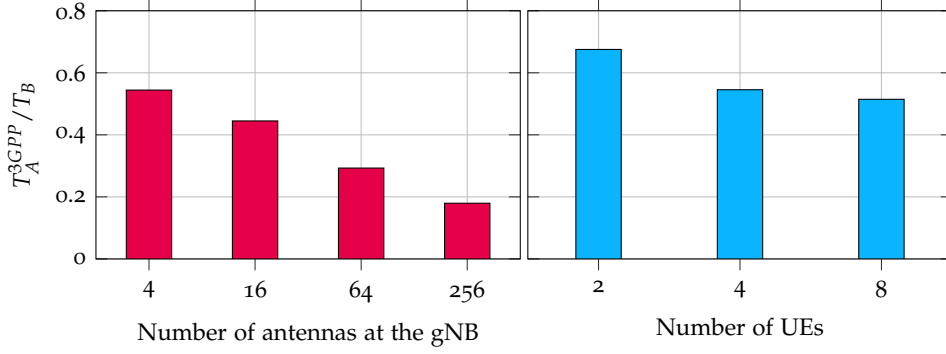
Figure 2.13: Ratio of the median simulation times after the merge of this work with the Eigen integration ( T_A^{3GPP} ) and as per ns-3.37 ( T_B ), when using the 3GPP channel model of [46].
