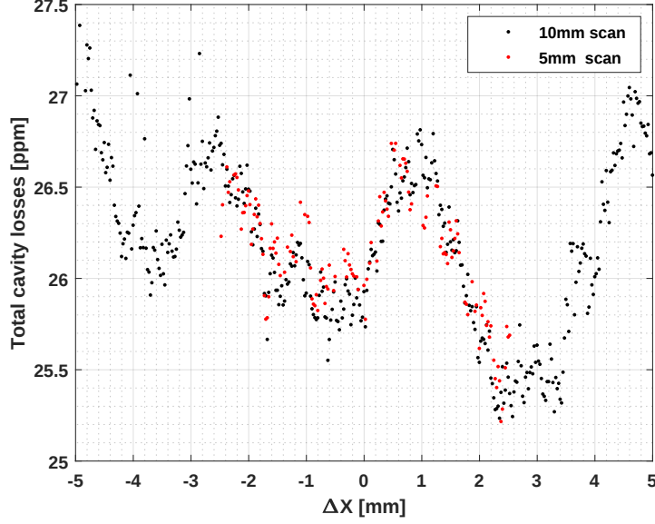
FIG. 9. Total cavity losses as a function of end mirror position along the cavity axis.
