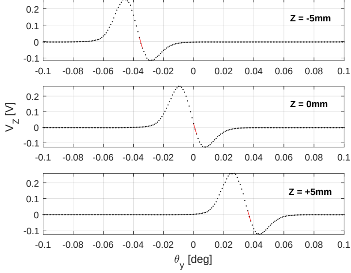
FIG. 4. Four quadrant photo-detector signal recorded as the mirror is tilted around the y axis of the hexapod (tilt of \theta_y ) for three different mirror positions \Delta_z = -5\text{ mm} ; \Delta_z = 0\text{ mm} \Delta_z = +5\text{ mm} .
