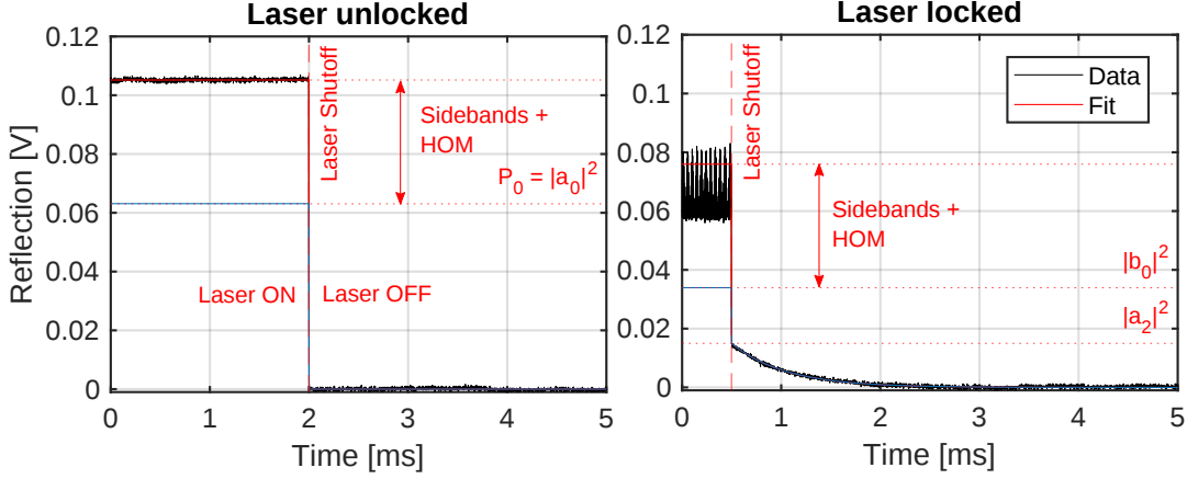
FIG. 12. PDH photodiode signal when the laser is on (right) and off (left) resonance. The recorded data is plotted in black lines and a least square fit is given in red. The blue lines represent the reflected optical power after subtraction of the sideband and HOM power that cannot be coupled into the cavity.
