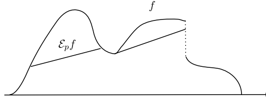
Fig. 4. The lower one-sided p -Lipschitz envelope \mathcal{E}_p f . Here the straight lines have slope p .
