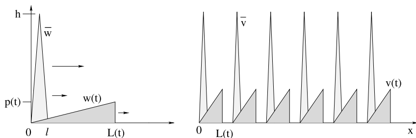
Fig. 2. Left: the elementary solution to Burgers' equation considered at (3.6)–(3.7). Right: the superposition of several shifted copies of the same solution.
