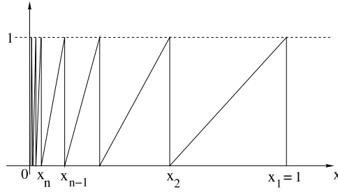
Fig. 1. The initial data considered in Example 3.1.
