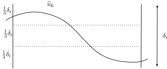
Fig. 6. Illustration of the case i \in \mathcal{J}_1 . At least one third of the variation is due to the regular part \tilde{u}_k .
