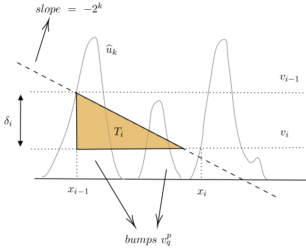
Fig. 5. The configuration considered in the estimate for i \in \mathcal{J} , in step 5 of the proof. (For interpretation of the colors in the figure(s), the reader is referred to the web version of this article.)
