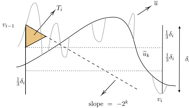
Fig. 7. The estimate for i \in \mathcal{J}_2 . From the fact that the value v_{i-1} survives up to time 2^{-k} , we deduce that the area of the yellow triangle can be controlled by the L^1 norm of all the v_q^p in the interval (x_{i-1}, x_i) .
