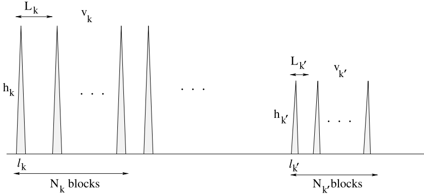
Fig. 3. A family of triangular wave packets.
