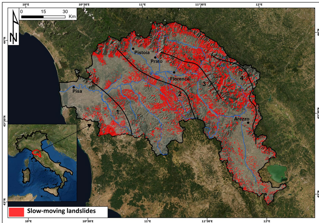
Fig. 2 Location, main drainage, slow-moving landslides and major mountain ridges of the Arno River basin. (1) Mt-Pisano-Montagnola Senese; (2) Mt. Albano-Chianti; (3) Calvana-Mt. Morello-Pratomagno; (4) Falterona-Mandrioli-Alpe di Catenaia
