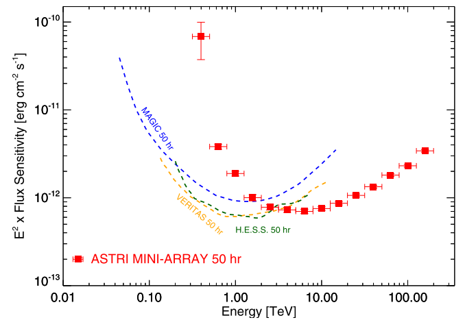
Fig. 9. ASTRI Mini-Array differential sensitivity compared with those of current imaging atmospheric Cherenkov telescope arrays. See text for details.
