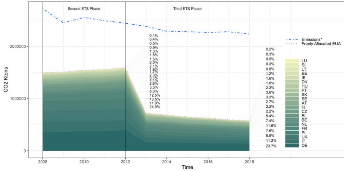
Figure A.5.3: Freely Allocated EUAs by Country
