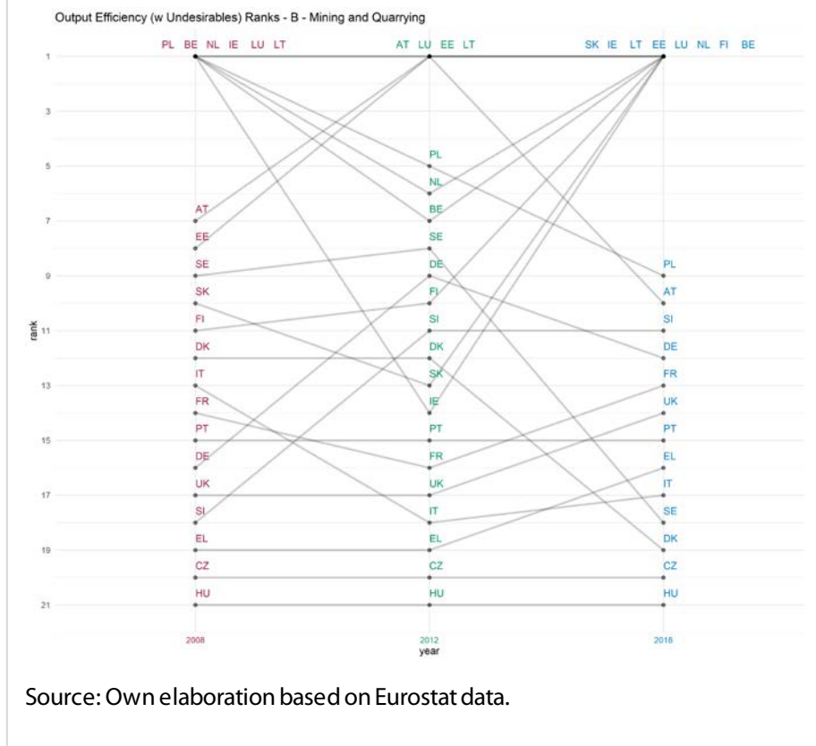
Figure A.5.12: Efficiency Ranking – Mining and Quarrying
