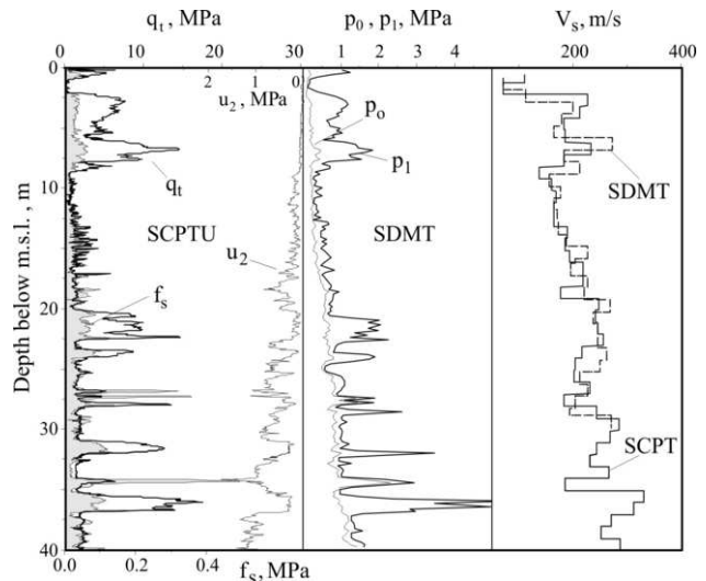
Figure 18. Example of in situ test results at the TTS.
