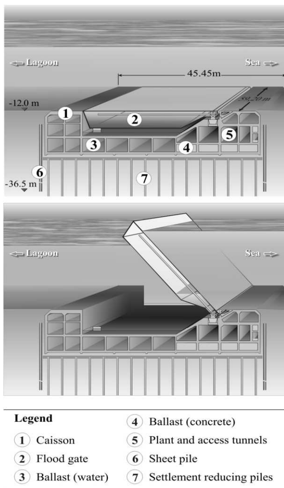
Figure 26. S.Nicolò barrier: flood gates operational scheme.
