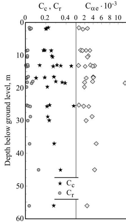
Figure 17. Compressibility parameters from oedometer test at the TTS.
