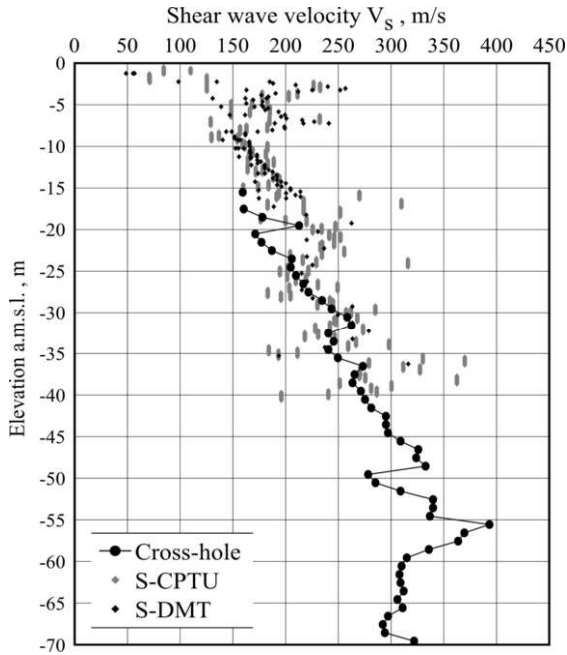
Figure 13. Shear wave velocity of the Lagoon deposits.
