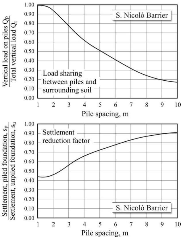
Figure 32. Results of soil-structure interaction analysis carried out by the code NAPRA, Russo (1998).
