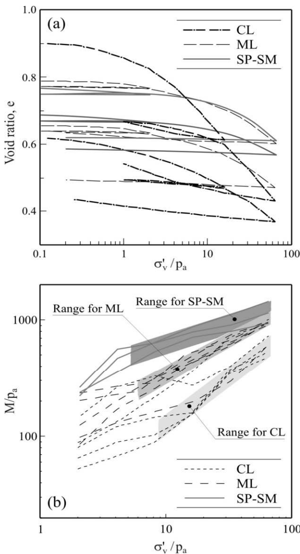
Figure 8. a) Examples of oedometer compression curves. b) Normalized constrained modulus vs. normalized vertical effective stress.
