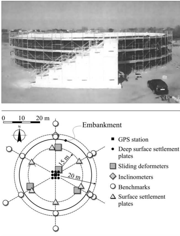
Figure 19a. Lido-Treporti trial embankment and layout of monitoring instrumentation.
