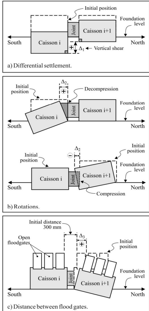
Figure 31. Differential displacements accounted in design.
