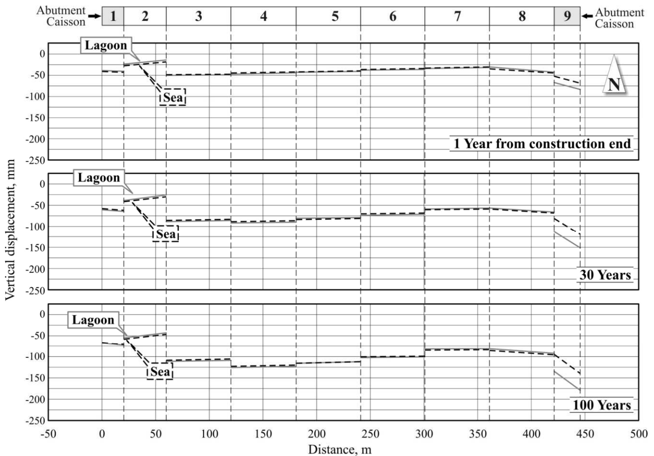
Figure 29. Computed vertical displacements of caissons of the barrier at S.Nicolò inlet.
