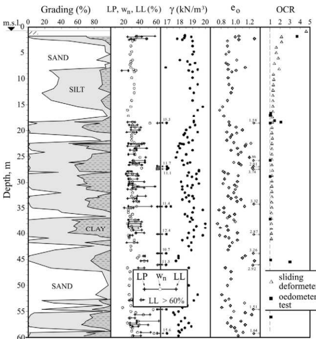
Figure 16. Soil profile and index properties at the TTS.
