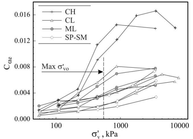
Figure 9. Coefficient of secondary compression vs. vertical effective stress at MTS.
