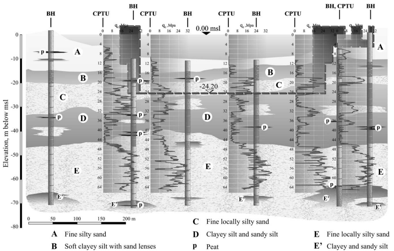
Figure 12c. Soil profile at the inlet of Chioggia.
