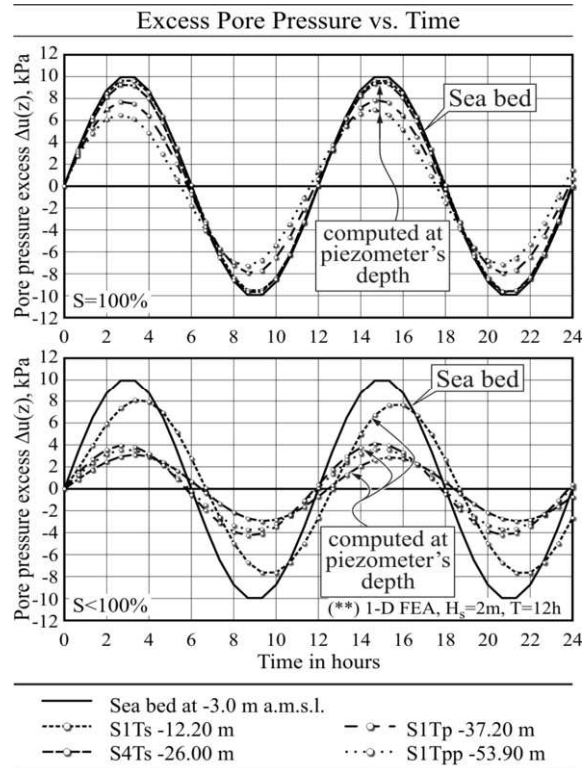
Figure 15b. Deamplification factor at the location of four piezometers.
