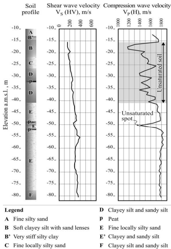
Figure 14. Results of cross-hole test at Malamocco inlet.
