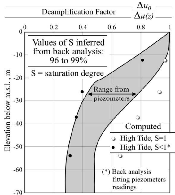
Figure 15a. Deamplification factor – Measured vs. computed.
