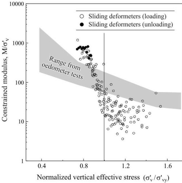
Figure 23. Site and laboratory normalized constrained modulus vs. normalized vertical effective stress.
