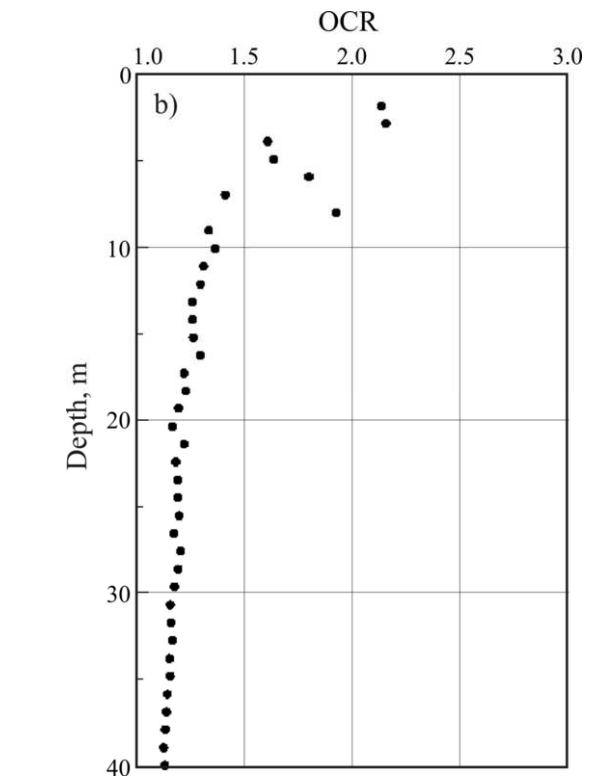
Figure 22. a) Field compression curves from sliding deformer. b) Overconsolidation ratio from field compression curves.
