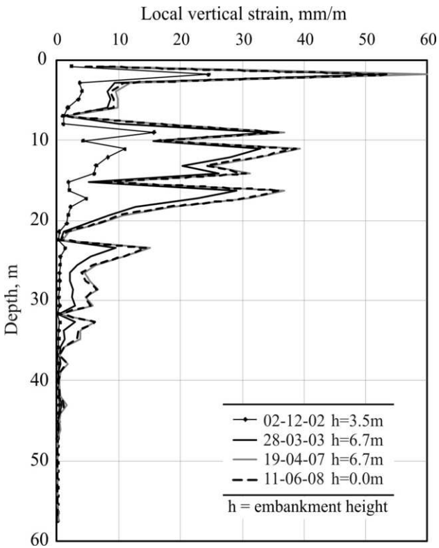
Figure 21b. Local strain under the centre of trial embankment.
