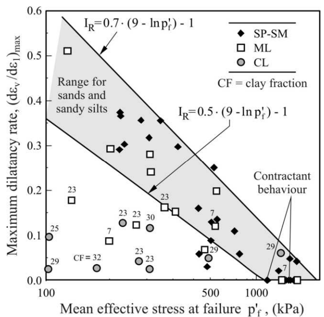
Figure 10. Maximum dilatancy rate vs. mean effective stress at failure.
