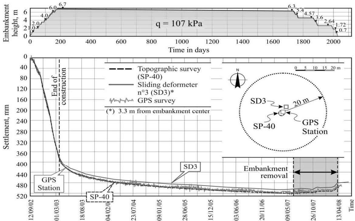
Figure 20. Time-settlement curves at the centre of the trial embankment, measured with different types of instruments.
