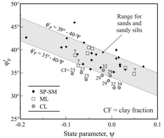
Figure 11. Peak angle of shearing resistance vs. state parameter.
