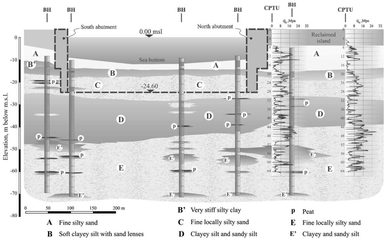
Figure 12a. Soil profile at the inlet of Lido-S.Nicolò.
