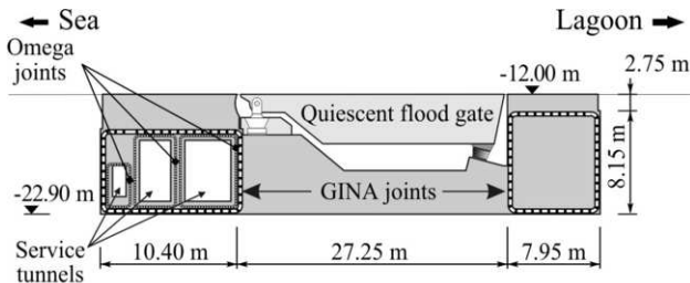
Figure 30. Cross-section of a caisson with the layout of the waterproofing joints.
