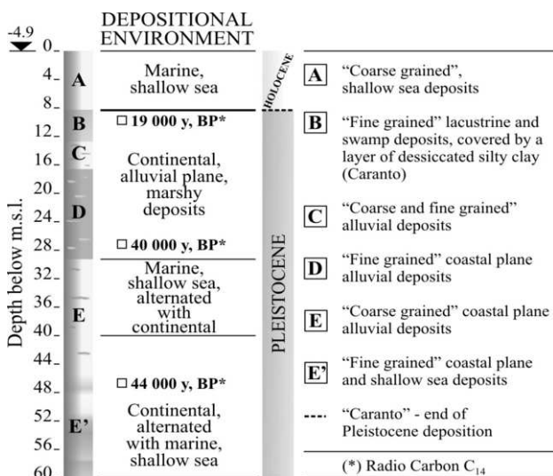
Figure 5. Scheme of depositional history at the Malamocco inlet (After Belloni and Caielli, 1997)
