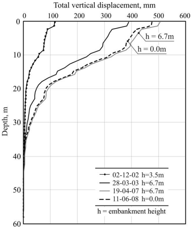
Figure 21a. Vertical displacement under the centre of trial embankment.
