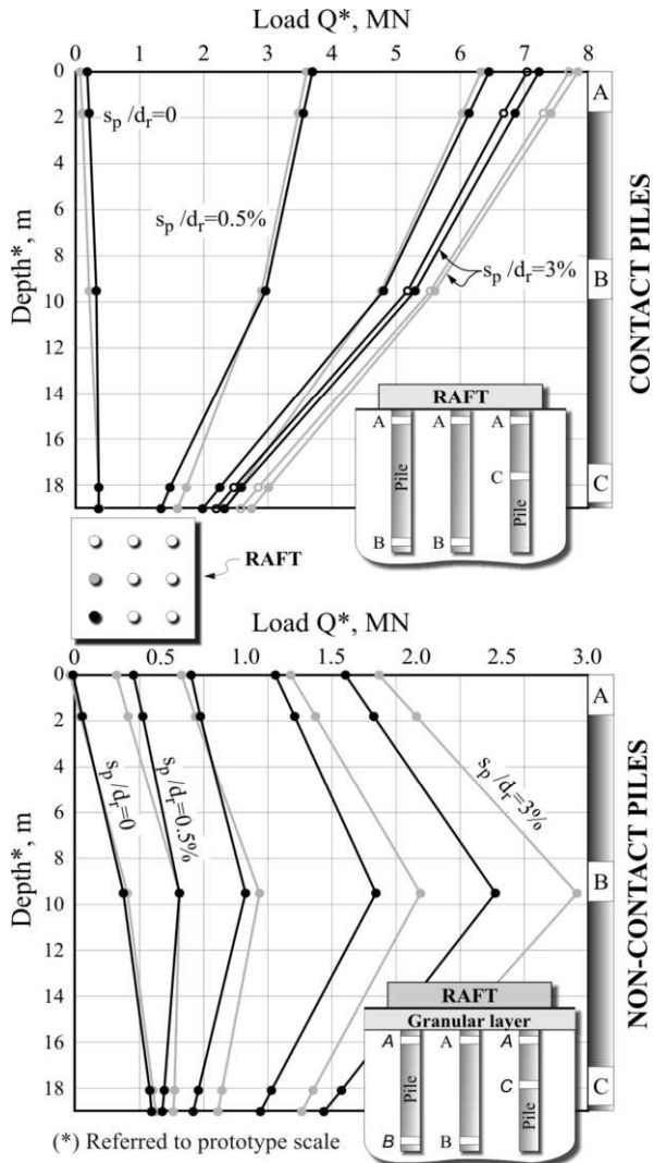
Figure 33. Square raft with nine piles on silty sand: axial load distribution along piles from centrifuge tests. ( d_r = raft diameter) Fioravante et al. (2007).
