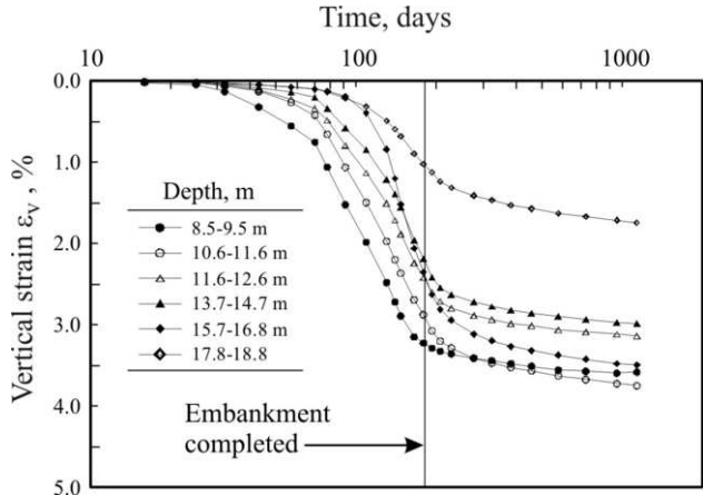
Figure 25. Vertical strain vs. time measured with the sliding deformer.
