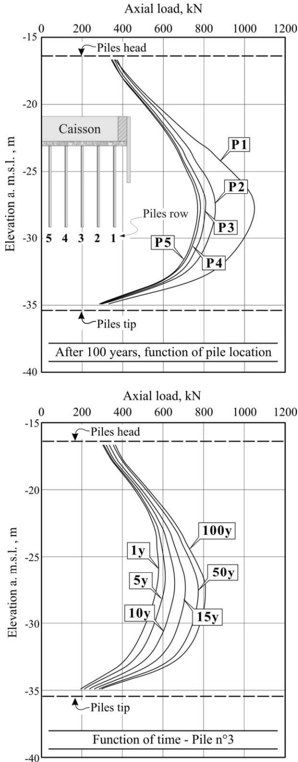
Figure 34. Load distribution along piles from F.E. analysis. Bonizzoni and Daprat (2006).
