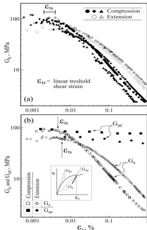
Figure 7. a) Secant shear modulus vs. shear strain b) comparison between secant shear modulus and unload-reload shear modulus.
