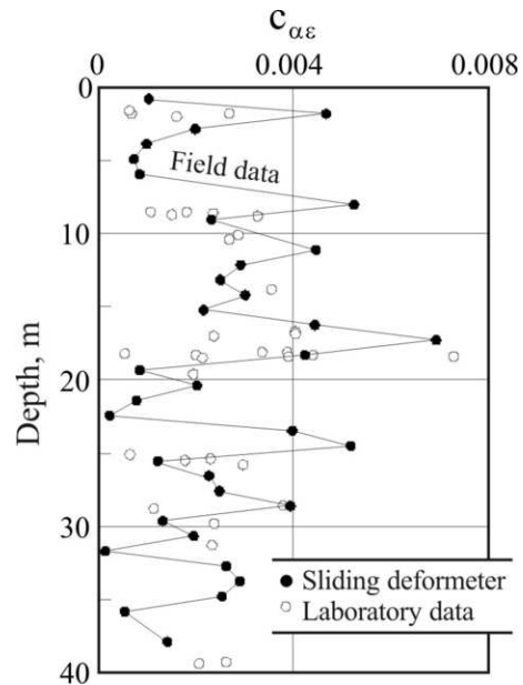
Figure 25. Comparison between field and laboratory secondary compression.
