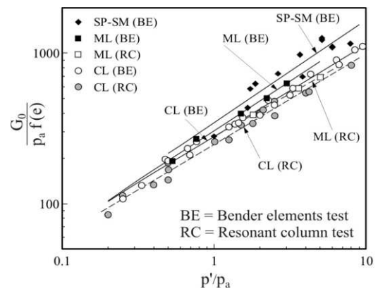
Figure 6. Normalized small strain shear modulus vs. normalized mean effective stress.
