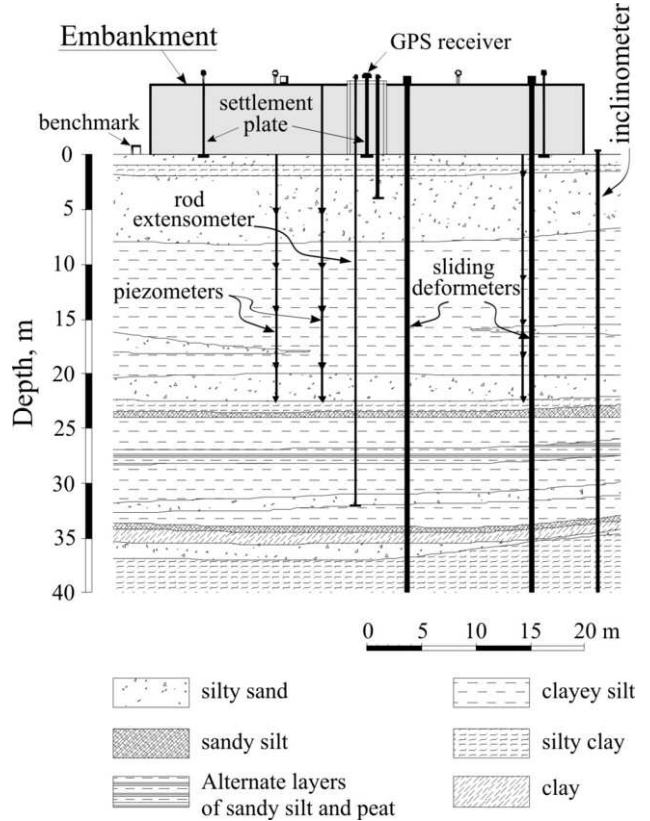
Figure 19b. Cross-section of trial embankment and underlying soil profile.
