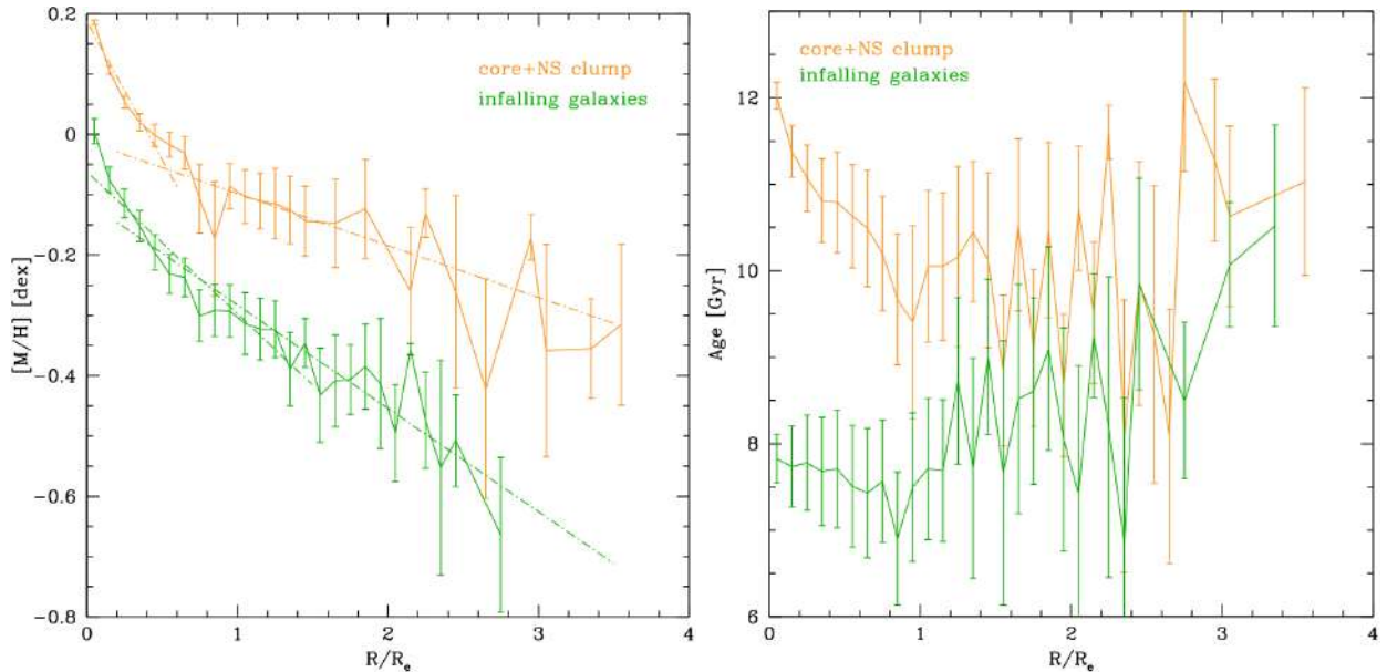
Fig. 4. Running mean as a function of radius of the azimuthally-averaged metallicity (left panel) and age (right panel) for the sample galaxies in the core-NS clump (orange symbols) and for those infalling in the Fornax cluster (green symbols). The dash-dotted lines represent the fits to the metallicity gradients between transition radii. The dash-dotted lines represent the fits to the metallicity gradients in the two regions defined by transition radii R_{tr,1} and R_{tr,2} . The error bars trace the dispersion of the points around the mean trend. The radial profiles of the stellar kinematics and population properties of the three edge-on galaxies, FCC 153, FCC 170, and FCC 177, have been excluded from the mean.
