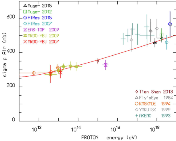
Fig. 16. FLUKA (PEANUT) computed proton-Air “particle production” cross-sections (red line) compared with experimental data [123–132] (symbols) from Cosmic Ray experiments up to 10^{19} eV.
