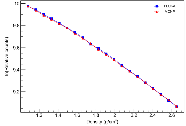
Fig. 71. Relationship between detector log relative counts and formation density in the near detector.
