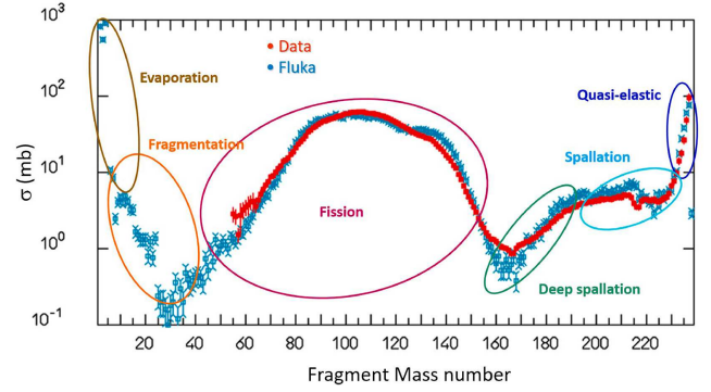
Fig. 11. Fragment mass distribution from 1 GeV protons on ^{238}\text{U} computed with PEANUT (dark cyan symbols) and compared with experimental data (red symbols [35,36]). Experimental data were actually measured at GSI in reverse kinematics.
