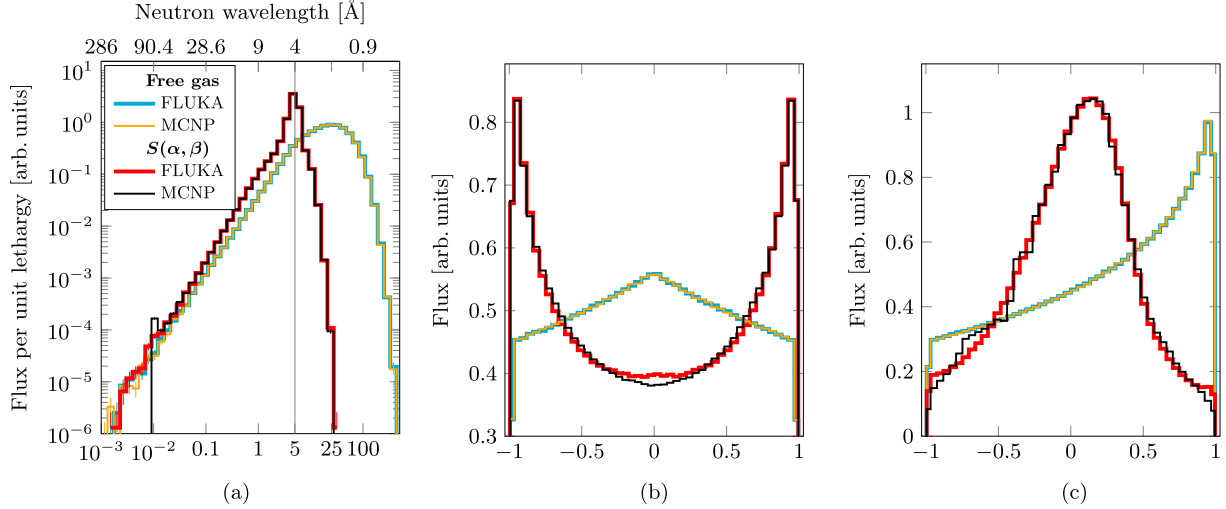
Fig. 52. 5 meV neutrons on para-hydrogen. (a) Neutron energy [meV]. (b) Direction cosine with respect to the axis perpendicular to the incident beam. (c) Direction cosine with respect to the axis collinear to the incident beam.
