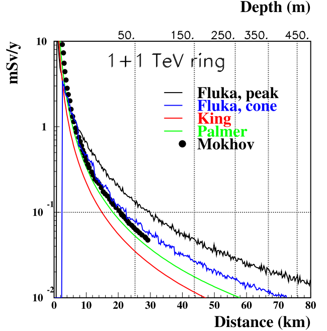
Fig. 64. H^*(10) from neutrino interaction products as a function of distance from the muon collider, or, equivalently, depth of the muon collider (top x -axis). Normalized to 1.2 \times 10^{21} \mu decays per year. The horizontal line draws the limit for population. Muon beams at 1 TeV (2 TeV centre of mass energy), radiation from the ensemble of the ring. FLUKA results labelled “peak” are averaged over 1 m in the vertical direction. FLUKA results labelled “cone” are averaged over 1/\gamma to be compatible with results in [319] (black symbols). The analytical approximations as in [320,321] (red and green lines) are displayed.
