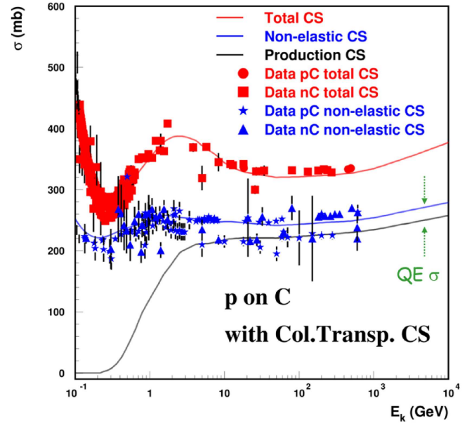
Fig. 17. FLUKA (PEANUT) computed proton on carbon total (red), non-elastic (blue), and particle production (black) cross-sections compared with experimental data [120,121] for proton and neutron interactions (symbols). The difference between the non-elastic and particle production cross-sections is the quasi-elastic contribution.
