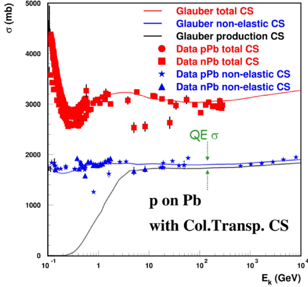
Fig. 15. FLUKA (PEANUT) computed proton on lead total (red), non-elastic (blue), and particle production (black) cross-sections compared with experimental data [120,121] for proton and neutron interactions (symbols). The difference between the non-elastic and particle production cross-sections is the quasi-elastic contribution.
