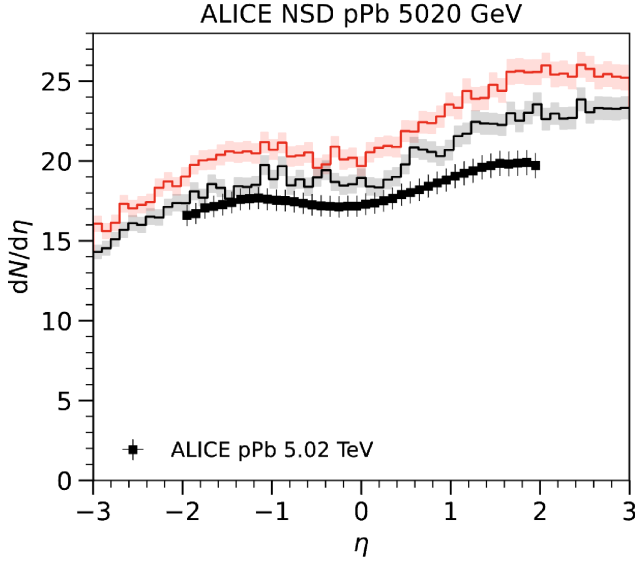
Fig. 29. Pseudorapidity distribution in proton-lead collisions measured by ALICE in non-single-diffractive events [164]. Note that this calculation was made without using pre-tabulated Glauber parameter distributions, which may result in slightly different numbers compared to the FLUKA defaults or distributions published in [164].
