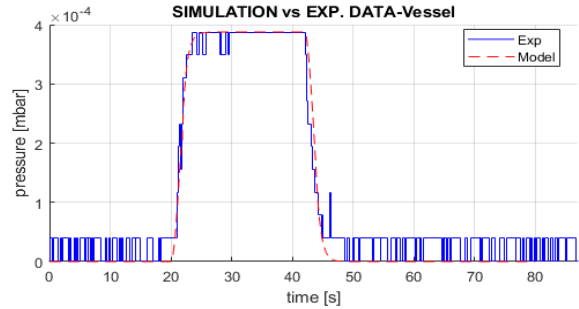
Fig. 5: Calculated and measured vessel pressure.
