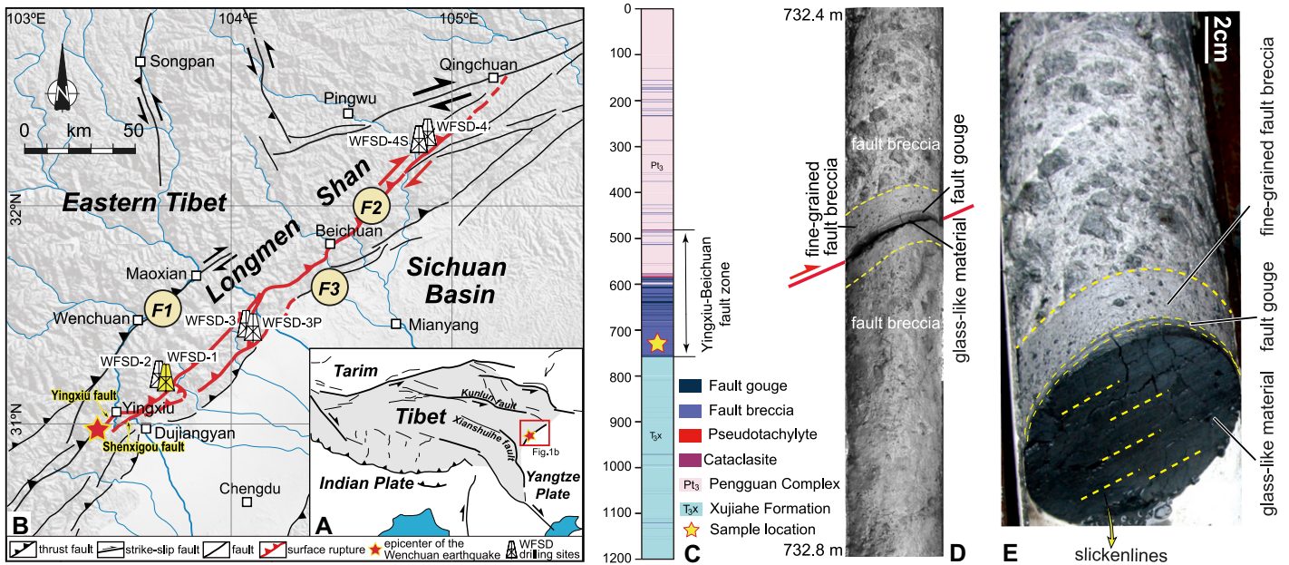
Figure 1. Tectonic setting and fault rocks in the first borehole of the Wenchuan Earthquake Fault Scientific Drilling Project (WFSD-1). (A) Active faults in the Tibetan Plateau. (B) Tectonic sketch of the Longmen Shan area in China and the WFSD drilling sites. F1—Wenchuan-Maoxian fault, F2—Yingxiu-Beichuan fault, F3—Guanxian-Anxian fault. (C) Fault rocks in the WFSD-1 core. (D) The core at 732.4–732.8 m depth, including a black 2-mm-thick layer bounded by (E) a striated, mirror-like principal slip surface.
