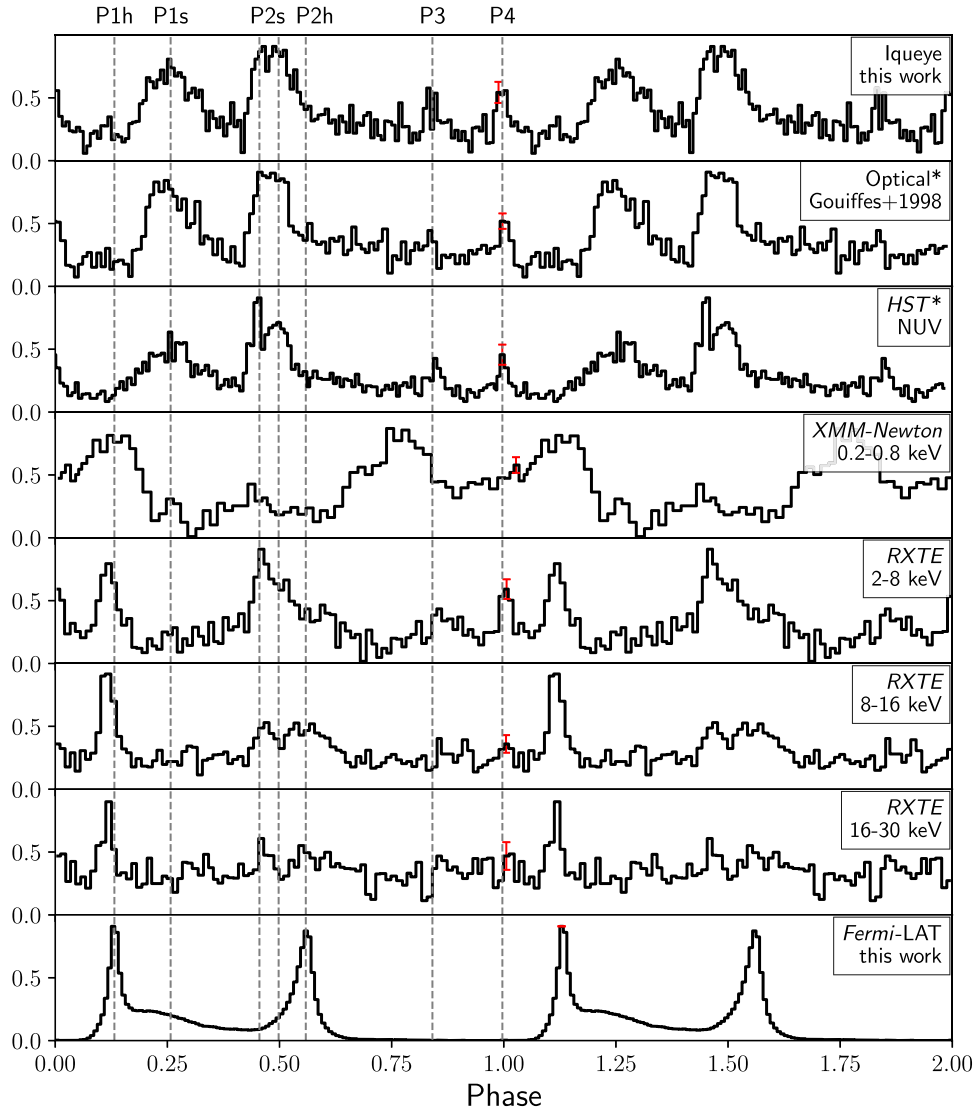
Figure 5. Normalized pulse profiles of the Vela pulsar in different energy bands. Optical, near UV, and X-ray profiles are adopted from Gouiffes (1998), Romani et al. (2005), and Kuiper & Hermsen (2015) and Harding et al. (2002), respectively. Pulse profiles from Gouiffes (1998) and Romani et al. (2005) (marked with asterisks) are shifted so as to align them with the Iqueye profile (see the text for details). Phase 0 corresponds to the radio peak. The vertical dotted lines mark the positions of different peaks. The average 1\sigma error bar for each profile is shown in red.
