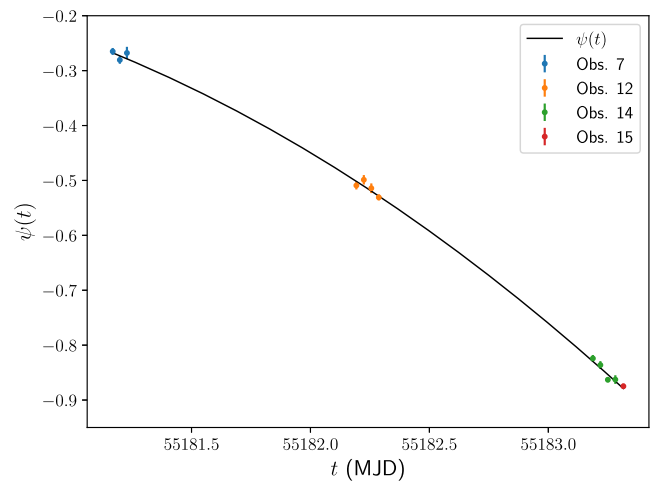
Figure 3. Phase drift of the Vela pulsar \psi(t) with respect to uniform rotation. Time t expressed in MJD.
