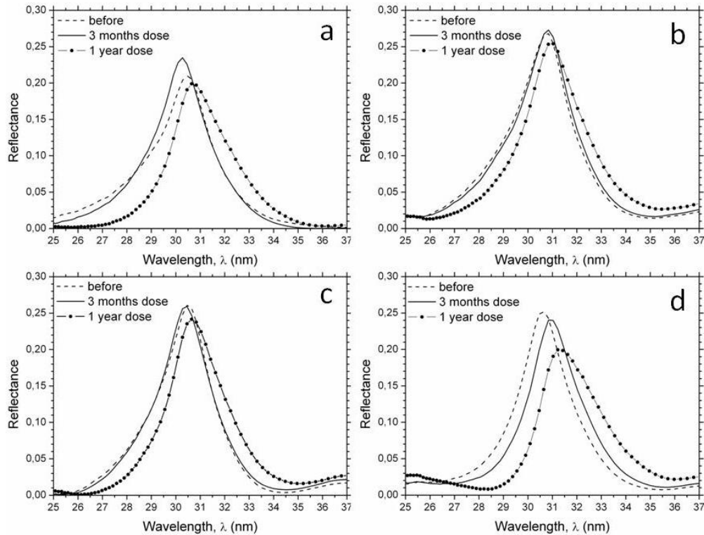
Fig. 2. Reflectance measurements of the structures REF (a), CL1 (b), CL2 (c) and CL3 (d) before and after low energy protons implantation experiment.
