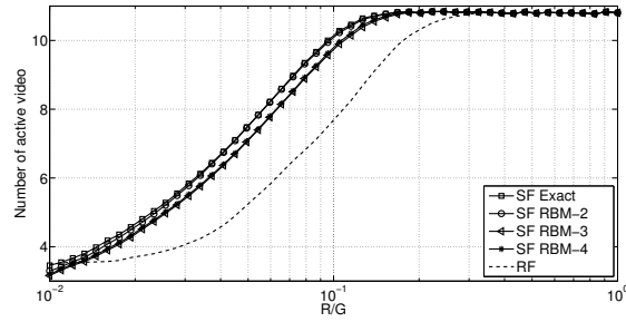
(a) Average number of admitted videos.
