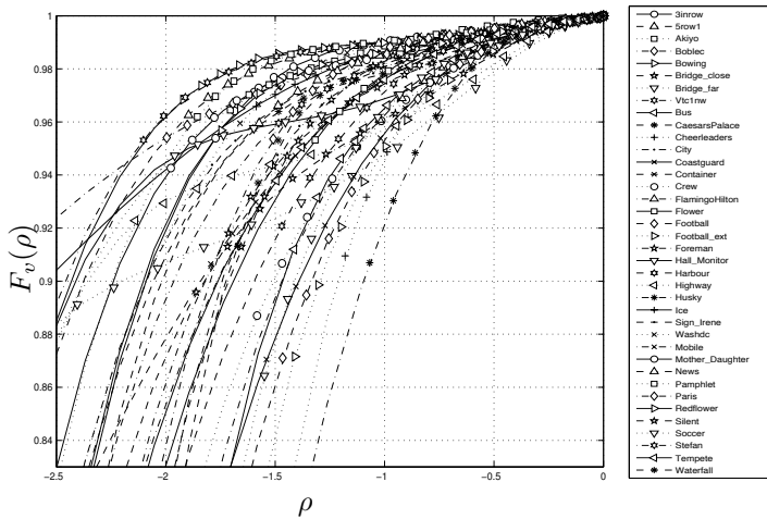
Fig. 2. SSIM of the different video clips when varying the RSF: markers show empirical values, lines are obtained by the 4-degree polynomial approximation F_v^{(4)}(\rho) .
