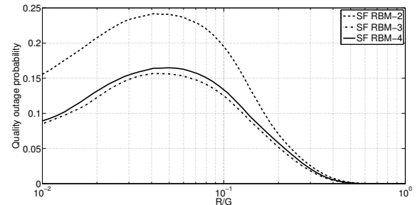
(d) Probability that video quality is under threshold (at least once during the video session).
