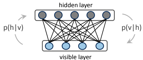
Fig. 3. Graphical representation of a Restricted Boltzmann Machine.
