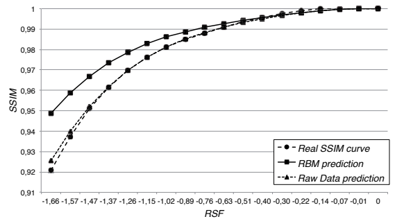
(b) Predicted and real curves for video number 11: raw data prediction shows better precision, but RBM prediction is still acceptable.
