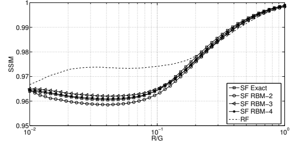
(b) Average SSIM of the admitted videos.
