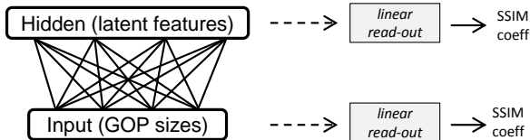
Fig. 4. Scheme of the proposed learning framework, on which unsupervised feature extraction (left) is followed by a supervised linear read-out (right).
