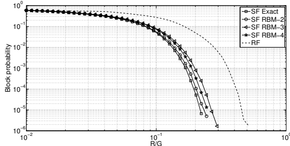
(c) Probability that video request is blocked.
