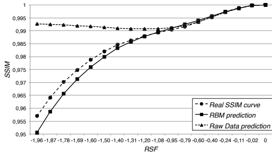
(a) Predicted and real curves for video number 2: RBM prediction shows better precision.
