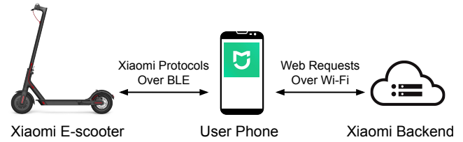
Figure 1: Xiaomi e-scooter ecosystem. Xiaomi e-scooter (left), the user smartphone running the Mi Home app (middle), and the Xiaomi backend (right). The e-scooter and the app are paired and connected over BLE. The app associates the e-scooter with the Xiaomi backend over Wi-Fi. We focus on the BLE traffic between the app and the e-scooter.
