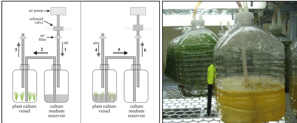
Figure 1. Temporary immersion bioreactor (TIB): The transfer of the medium to the plant culture vessel occurs by a positive pressure of the air pump and the explants are temporarily immersed, after this, the air pump starts and the medium returns to the culture medium reservoir (A) scheme, (B) picture.
