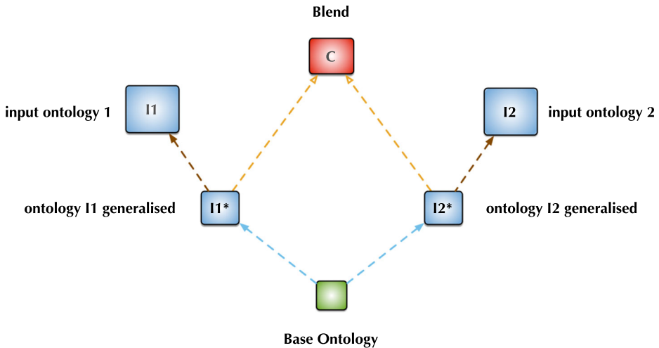
Fig. 2 The core model of computational conceptual blending
