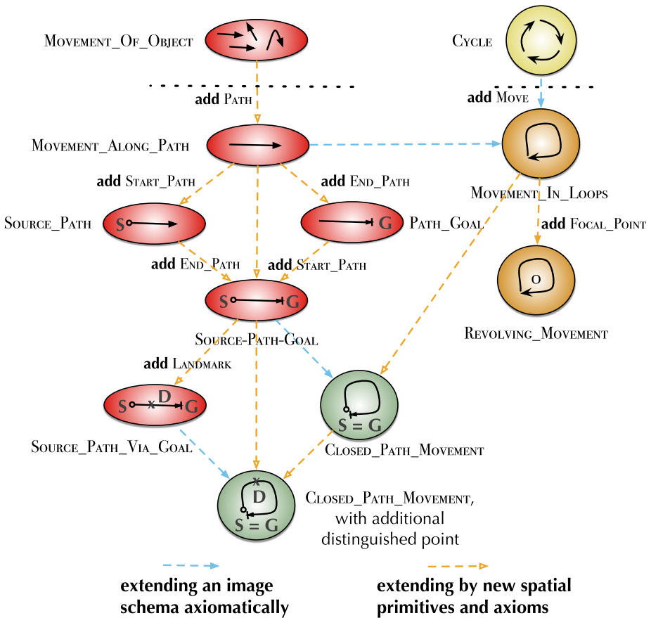
Fig. 6 Selected image schemas of path and cyclic movement as a graph. The coloured arrows described as “extending an image schema axiomatically” respectively “extending by new spatial primitives and axioms” illustrate by which means the PATH family is formally extended
