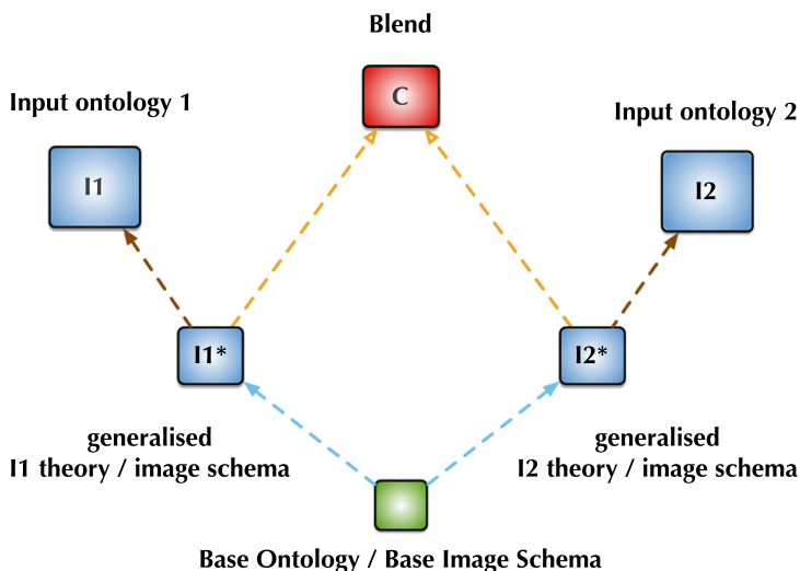
Fig. 8 Blending using common image schemas through theory generalisation
