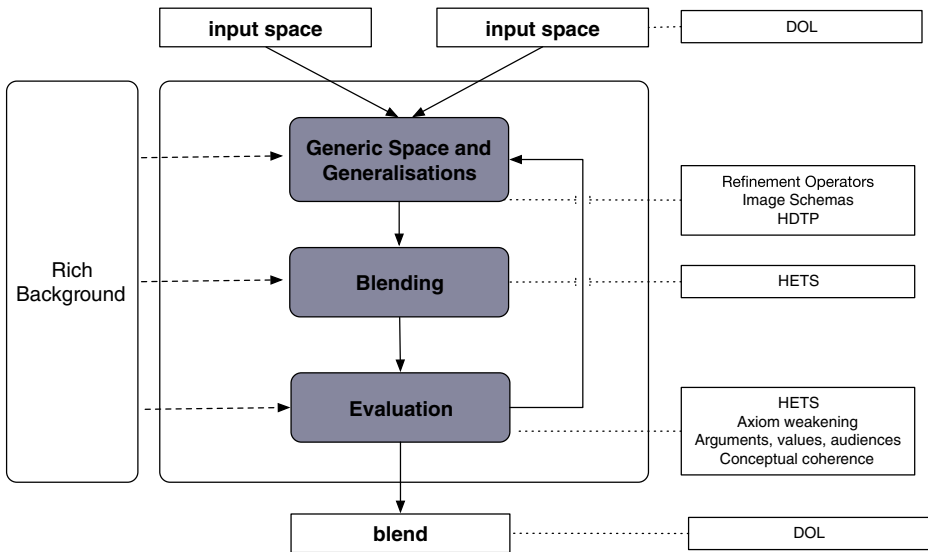
Fig. 3 Concept-invention workflow and enabling techniques
