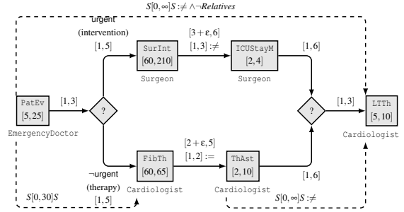
Figure 1: Official STEMI guidelines (excerpt). We model TSoD as [1, 3] \neq , TBoD as [1, 2] = . Ranges [x, y] and [x + \epsilon, y] model all durations t s.t. x \leq t \leq y and x < t \leq y , respectively.
