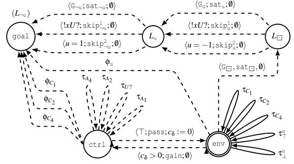
Figure 3: TGA equivalent to the CSTNU in Fig. 2.
