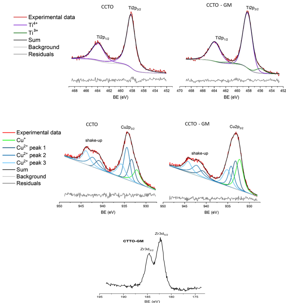
Fig. 4 XPS of CCTO and CCTO-GM. Top row; Ti 2p region for CCTO (left) and CCTO-GM (right) with associated data fitting. Second row; Cu 2p 3/2 region for CCTO (left) and CCTO-GM (right) and fittings. Bottom row; Zr 3d region for CCTO-GM.
