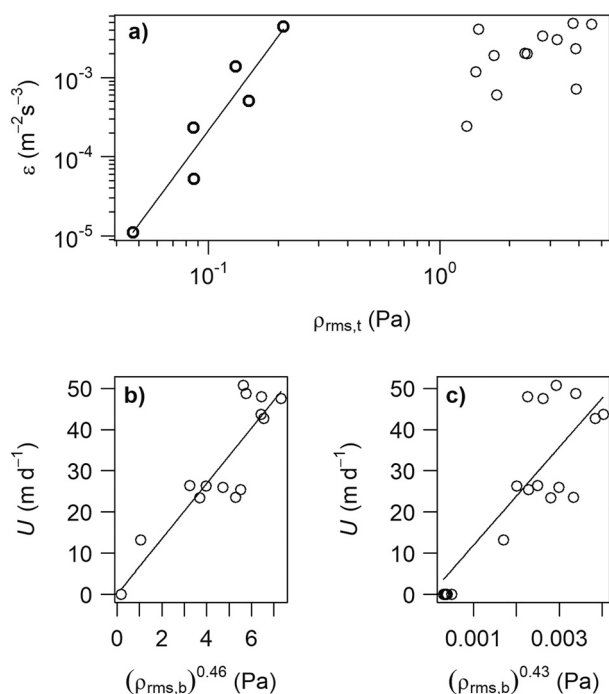
Figure 7. Relationship between indicators of underwater sound, turbulence and bubble flux. (a) root-mean-square sound pressure at 10–100 Hz ( \rho_{rms,t} ) versus turbulent kinetic energy dissipation rate ( \epsilon ), (b) root-mean-square sound pressure at 5–10 kHz measured underwater ( \rho_{rms,b} ) versus superficial gas velocity ( U ), (c) as in (b) but for sound measured above the water surface. Lines show best fits of regression models: (a) \log_{10}(\epsilon) = 3.83 \log_{10}(\rho_{rms,t}) + 0.46 (fitted to data without bubbles only; circles with thick outline), (b) U = 6.73 \rho_{rms,b}^{0.46} ; (c) U = 1.19 \cdot 10^4 \rho_{rms,b}^{0.43} . For model details, see Table S2 in Supporting Information S1.
