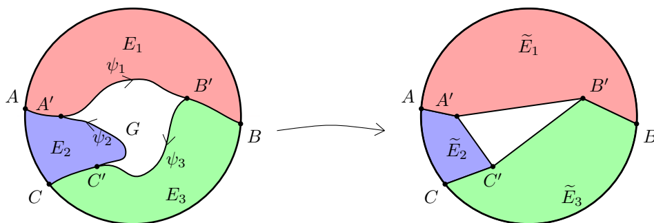
FIGURE 10. The paths \psi_1 , \psi_2 and \psi_3 and the points A , B , C , A' , B' , C' in Lemma 2.15.
