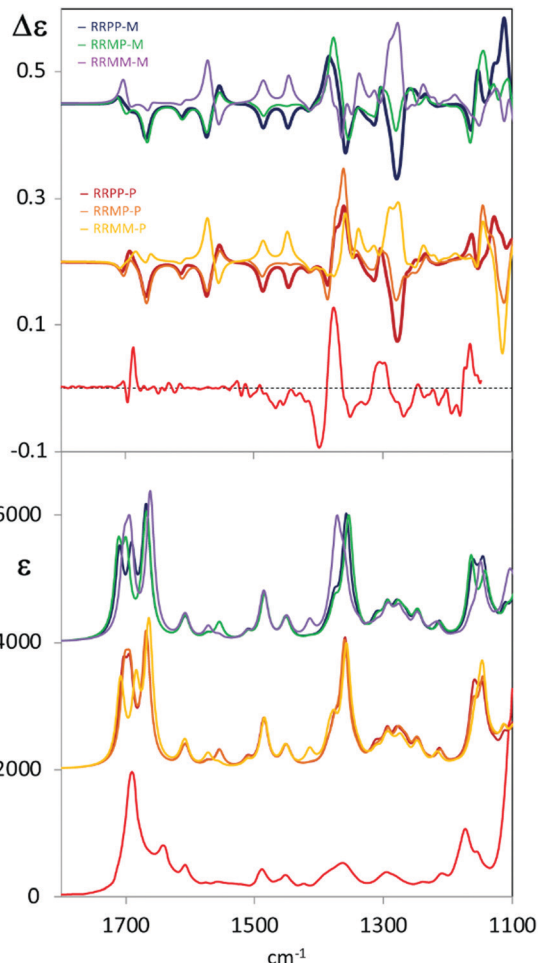
Fig. 3 Comparison of experimental VCD spectra of C_6F@ (R,R)-1 (top) and IR absorption spectra of C_6F@ (R,R)-1 with calculated VCD and IR spectra of C_6F@ (R,R)-1 with the two head groups and fluorinated chains in all possible configurations ( PP-M , PP-P , MM-M , MM-P , MP-M , MP-P ). Experimental data in red.
