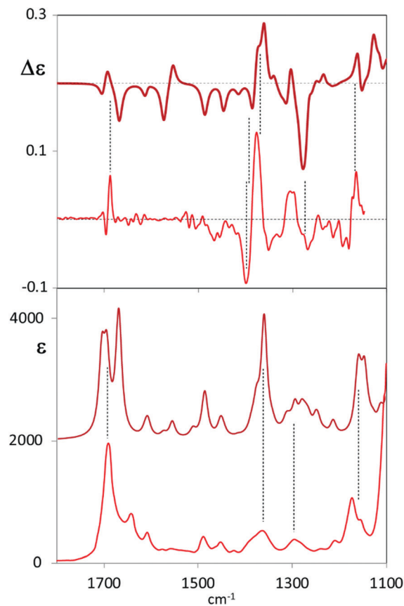
Fig. 1 Comparison of experimental (lower traces) VCD spectra of C_6F@ (R,R)-1 (top square) and IR absorption spectra (lower square) of (R,R)-C_6F@ 2 (see Scheme 1) with calculated (upper traces) VCD and IR spectra of C_6F@ (R,R)-1 with the two head groups in P,P configuration and with the P configuration of the fluorinated chain. Experimental data are displayed with weaker lines in the lower part of each panel; main correspondences are evidenced with vertical lines.
