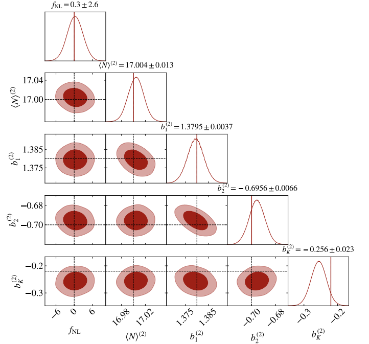
Fig. B.5. Corner plot for f_{\text{NL}} and bias parameters, for Run #4, catalogue 2. Similar to Fig. B.4, there are little to no degeneracies between f_{\text{NL}} and the bias parameters.
