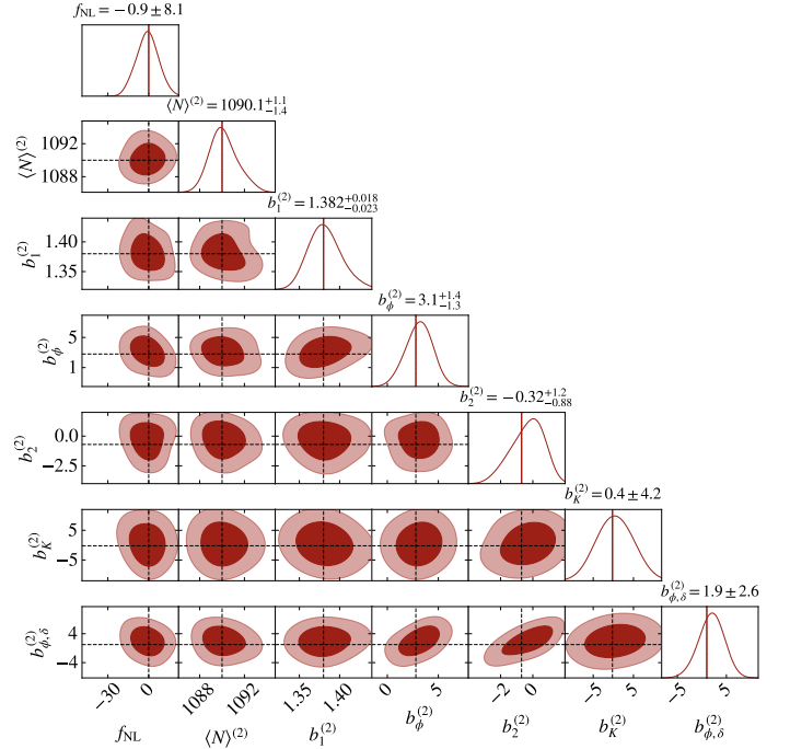
Fig. B.9. Corner plot for f_{\text{NL}} and bias parameters, for Run #7, catalogue 2. Similar to Fig. B.4, there are little to no degeneracies between f_{\text{NL}} and the bias parameters.
