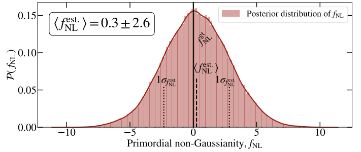
Fig. 6. Field-level results for inferring f_{\text{NL}} for a high-resolution run (Run #4). The figure illustrates that the method can find a unimodal marginalised distribution of f_{\text{NL}} that best explains the data, with the ground truth value f_{\text{NL}}^{\text{gt}} (solid line) within the 68.3% CI of the estimated value. The value in the box is the maximum of the distribution in the range of 68.3%. We point out that these results are based on the universal mass function, which means that the scale-dependent bias parameters are fixed to the expressions in Eqs. (5) and (6).
