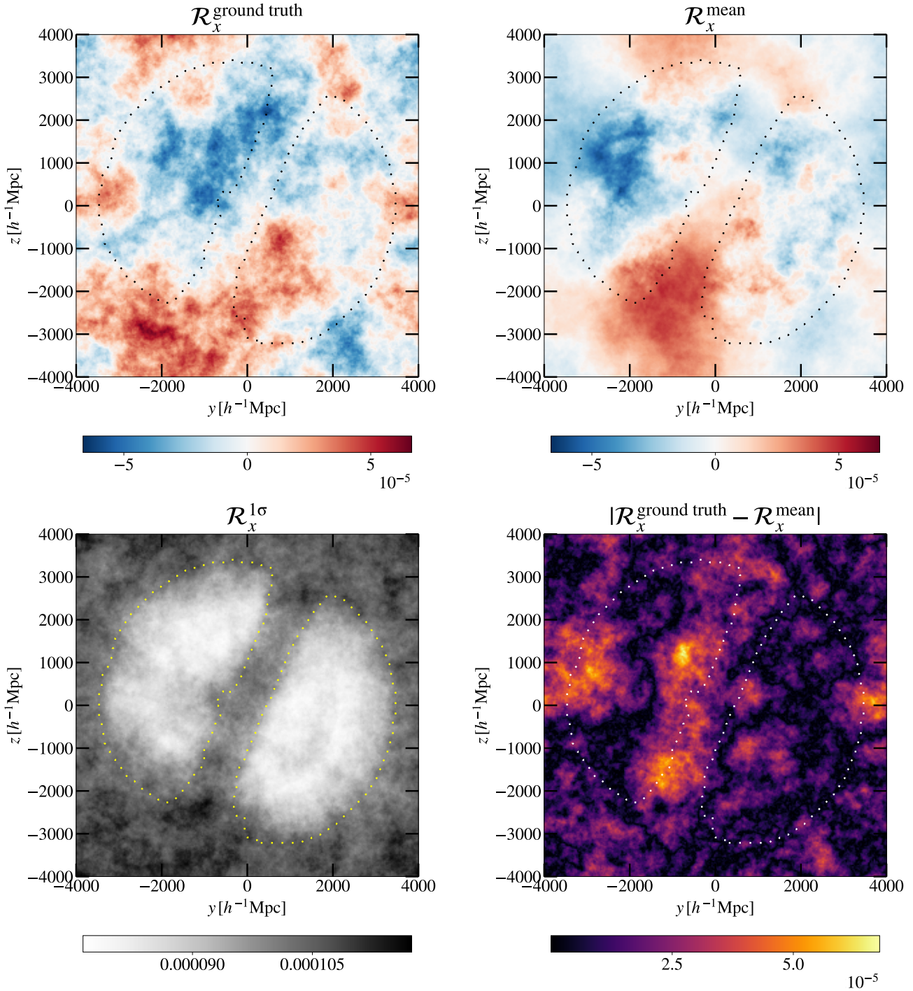
Fig. 9. Illustrations of the inferred adiabatic curvature fluctuations. For each saved sample, we have a set of initial conditions \epsilon that produce a plausible set of model predictions, constrained by the data. Each set of initial conditions corresponds to a field of adiabatic curvature fluctuations (Eqs. (2) and (7)), which are the input to the structure formation model. By computing these fluctuations for a subset of the chain, the method can provide an expected estimate of the fluctuation of the adiabatic curvature along with uncertainty. We highlight the edge of the survey window with the dotted lines, meaning that voxels outside of the inner regions in the final observed field contain no observations. In the top-left plot, we have included the ground truth field of adiabatic curvature fluctuations used to generate the mock data, averaged over the x direction. In the top-right plot, we have the expectation value of the adiabatic curvature fluctuations averaged over the x direction. In the bottom-left plot, we have the corresponding uncertainty averaged over the x direction. Lastly, in the bottom-right plot, we include the absolute difference between the mean inferred field and the ground truth field.
