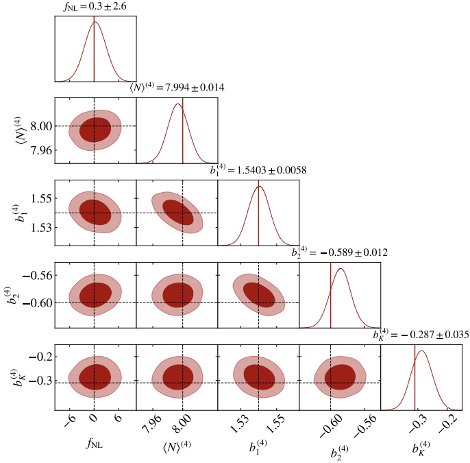
Fig. B.7. Corner plot for f_{\text{NL}} and bias parameters, for Run #4, catalogue 4. Similar to Fig. B.4, there are few to no degeneracies between f_{\text{NL}} and the bias parameters.
