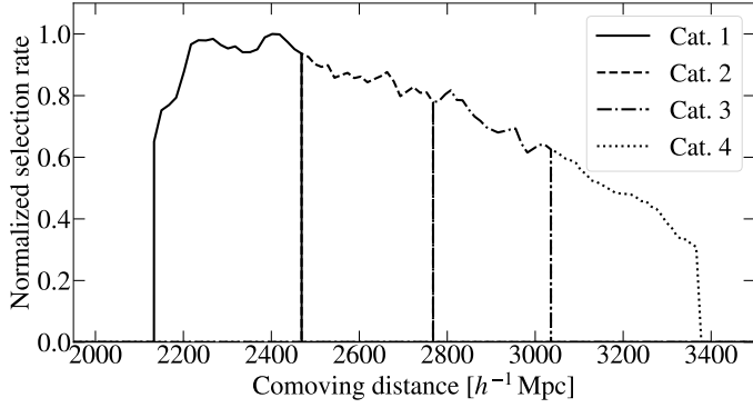
Fig. 5. Euclid radial selection function. This plot displays the normalised radial selection, dN(z)/(d\Omega dz) , for the four galaxy catalogues in this project. Notice how the tracer catalogues do not overlap but rather cover separate regions in the mock universe.
