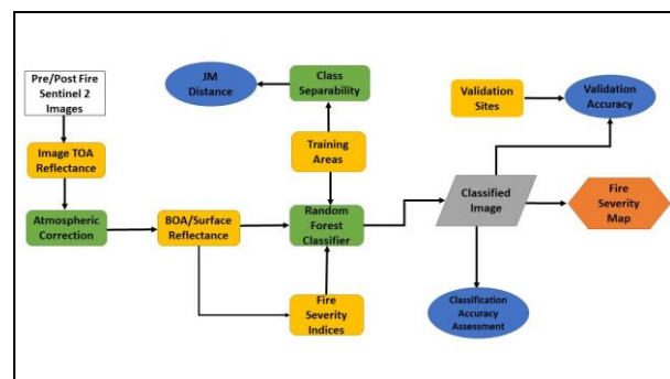
Figure 3. Flowchart of the methodology used in the study To further strengthen the separability between the classes and the accuracy of the classification, following Gibson et al. (2020), the following vegetation indices relevant to burned sites were computed using both the pre-and post-fire images:
