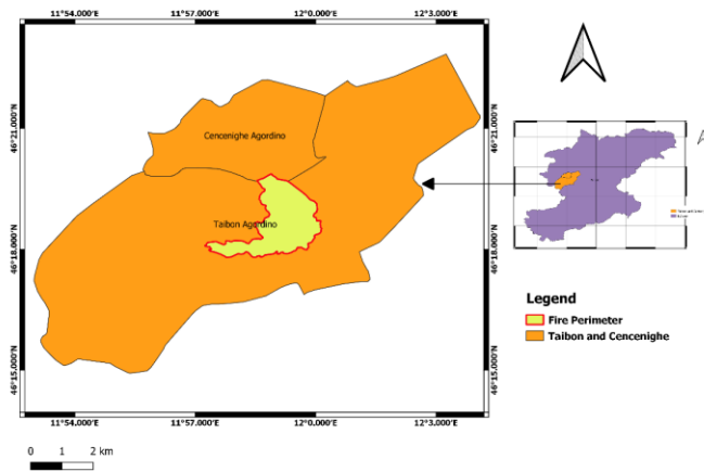
Figure 1. Location of the study area in Taibon Agordino, Belluno Province, Italy
