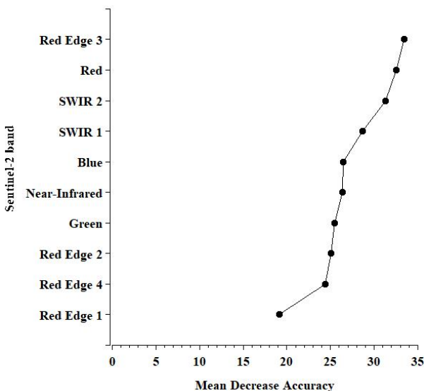
Figure 5. Variable importance plot produced by applying the Random Forest to all the original band reflectance of the postfire Sentinel-2 image
