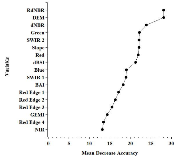
Figure 6. Variable Importance Plot produced by applying the Random Forest classifier to the postfire Sentinel-2 original band reflectance, associated vegetation indices, the DEM, and slope.
