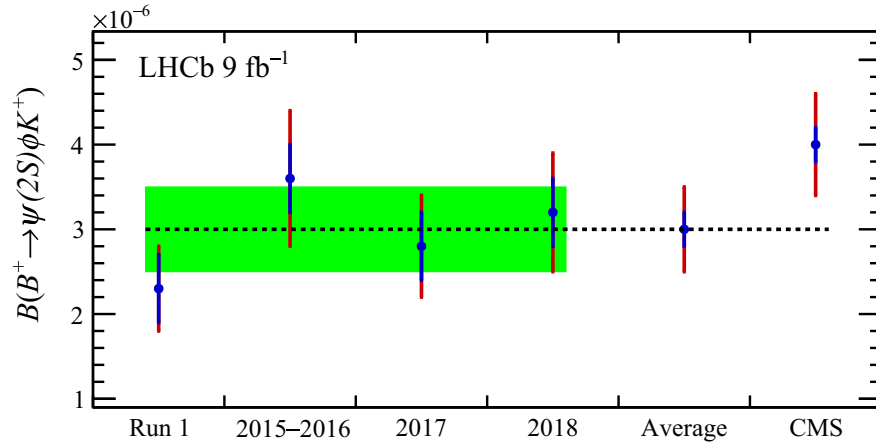
FIG. 5. Branching fraction of the decay B^+ \rightarrow \psi(2S)\phi K^+ for each data-taking period and the confidence level region at one standard deviation for the combined result in green. The inner error bars (in blue) and the outer error bars (in red) delimit the statistical and total (statistical plus systematic, added in quadrature) uncertainties, respectively. The CMS result [7] is included for comparison.
