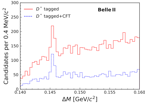
Figure 10: Distribution of the difference between D^{*+} and D^0 masses for wrong-sign D^{*+} \rightarrow D^0(\rightarrow K^+ \pi^- \pi^0) \pi^+ decays reconstructed in data and selected with and without the requirement q_{\pi_s} q > 0 .
