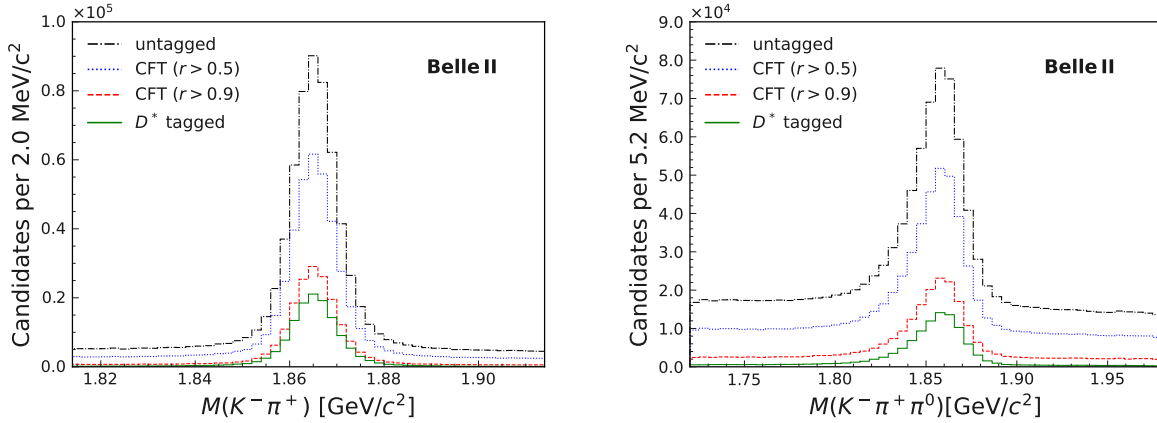
Figure 9: Mass distributions for (left) D^0 \rightarrow K^- \pi^+ decays and (right) D^0 \rightarrow K^- \pi^+ \pi^0 decays reconstructed in data with different requirements on the predicted (uncalibrated) dilution in comparison with D^{*+} -tagged decays. For the selections shown the D^0 \rightarrow K^- \pi^+ signal purities are 0.94 ( D^{*+} -tagged), 0.84 (CFT, r > 0.9 ), 0.73 (CFT, r > 0.5 ), and 0.67 (untagged). For D^0 \rightarrow K^- \pi^+ \pi^0 decays the signal purities are 0.80 ( D^{*+} -tagged), 0.53 (CFT, r > 0.9 ), 0.38 (CFT, r > 0.5 ), and 0.34 (untagged).
