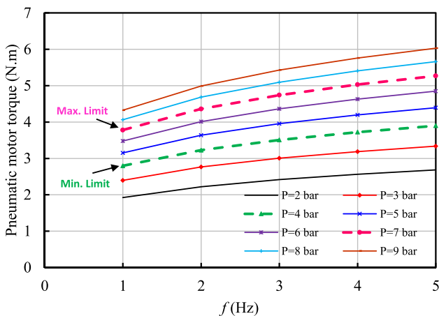
Fig. 15 Effect of pulsating air frequency on the motor torque at different main source pressures
