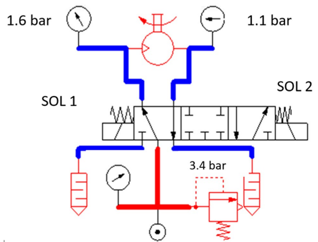
Fig. 2 Pneumatic circuit diagram for a fixed-displacement unidirectional pneumatic motor
