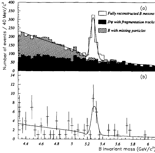
Fig. 6. (a) simulation of Z \rightarrow J/\psi(\psi') X : sum of B invariant-mass distribution for all selected exclusive decay channels with the two relevant components of the background. The curve shows a fit with a Gaussian for the B decays plus background. (b) Same distribution for 1991 and 1992 real data. The curve shows the fit to the data with the slopes of the backgrounds and the width of the signal fixed to the simulated data above.
