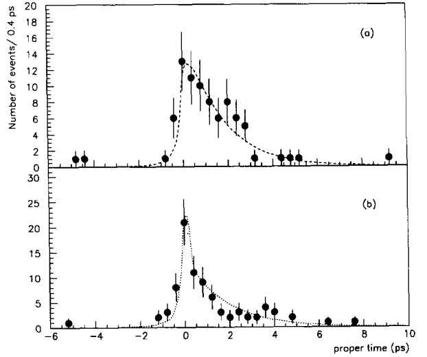
Fig. 5. Proper time distribution for the J/\psi candidates (muon data only). The curve shows the result of the unbinned maximum likelihood fit to determine the lifetime: a) signal events; b) sideband events. The “lifetime” of the background is due to semileptonic decays of heavy flavours.
