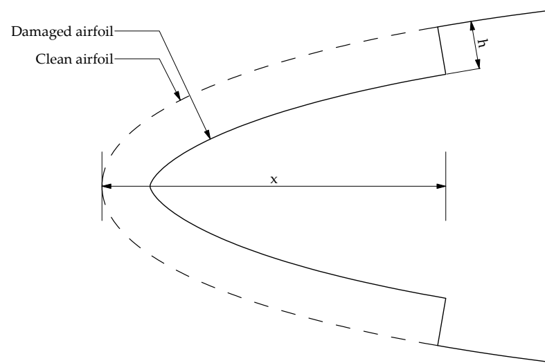
Figure 5. Geometrical representation of the LEE configuration. The chordwise delamination extent is denoted with the letter x and the delamination depth is denoted with the letter h .
