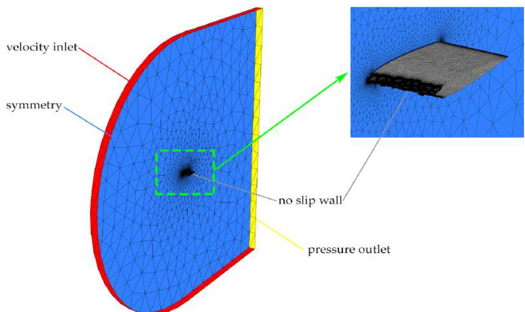
Figure 4. Boundary conditions overview: the red surface is the velocity-inlet while the pressure-outlet is highlighted in yellow. To enhance clarity only one side boundary, with symmetry condition imposed, is shown in light blue.
