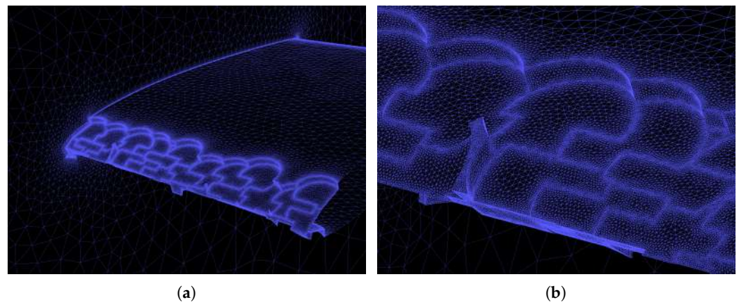
Figure 3. Mesh overview (a) and detail (b) of the three-dimensional geometry. The figures refer to the fine grid of 5 million elements.
