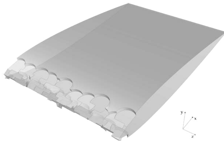
Figure 2. Geometrical representation of the three-dimensional blade with LEE.
