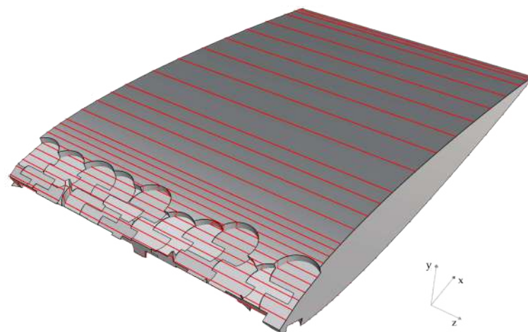
Figure 17. Geometrical representation of the lines where friction and pressure coefficient are evaluated.
