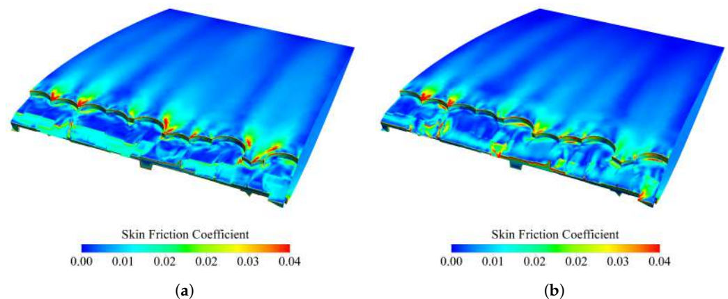
Figure 12. Comparison between contour plots of the friction coefficient on the damaged blade at 0^\circ incidence and 4^\circ incidence. (a) C_f contour at \alpha = 0^\circ ; (b) C_f contour at \alpha = 4^\circ .
