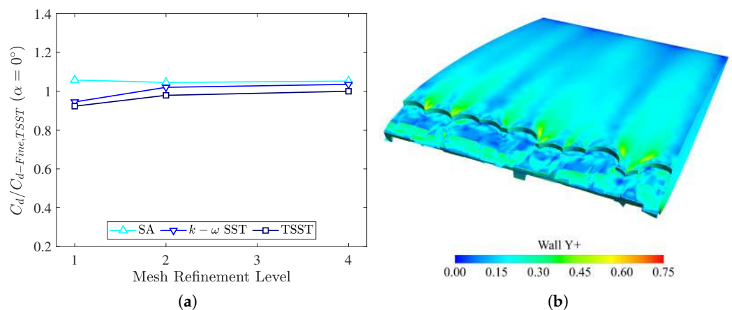
Figure 10. Three-dimensional model validation. (a) CFD-computed drag coefficient of the damaged blade as a function of the turbulence model and the mesh refinement level; (b) Wall y^+ contour obtained with the finest grid and the TSST model at 0^\circ incidence.
