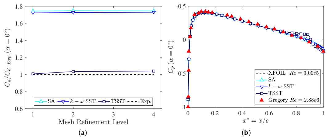
Figure 7. Two-dimensional model validation. (a) Comparison between the experimental and the CFD-computed drag coefficient of the undamaged NACA 0012 airfoil as a function of the turbulence model and the mesh refinement level; (b) Pressure coefficient distribution as a function of the turbulence model obtained using the finest grid. Red triangles denote the pressure coefficient experimentally acquired by Gregory and O'Reilly [57]. Single curve reported being the flow symmetric.
