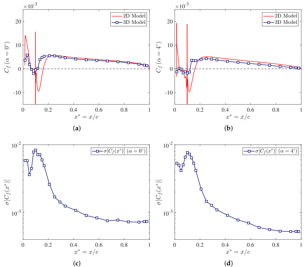
Figure 19. Friction coefficients comparison between the 2D damaged airfoil and the 3D eroded blade. Dark blue squares denote the \overline{C_f}(x^*) value over the three-dimensional blade. (a) C_f distribution at 0^\circ incidence; (b) C_f distribution at 4^\circ incidence; (c) Friction coefficient standard deviation on the blade at 0^\circ incidence; (d) Friction coefficient standard deviation on the blade at 4^\circ incidence.
