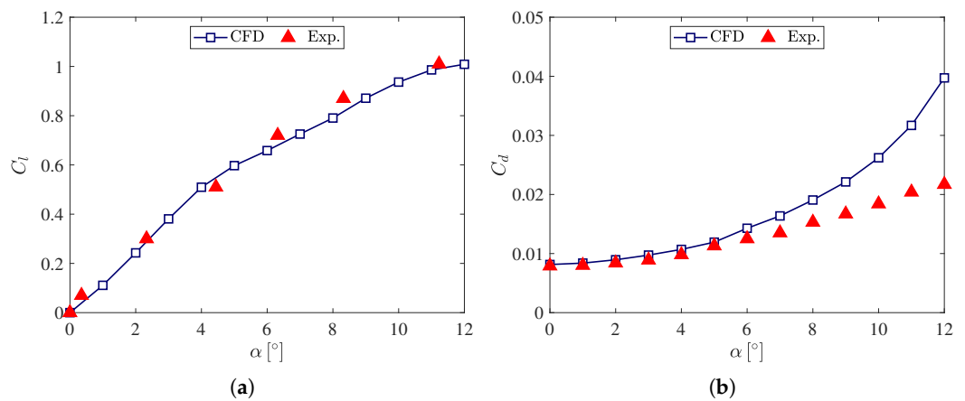
Figure 9. Comparison between lift and drag polar diagrams obtained with the finest grid (using the TSST turbulence model) and the experimental data for NACA 0012 airfoil. (a) C_l as a function of the incidence; (b) C_d as a function of the incidence.
