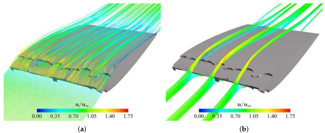
Figure 11. Streamlines around the damaged blade at 4^\circ incidence. (a) Streamlines on the suction side of the blade; (b) Streamlines in three xy planes passing through 1/4 , 1/2 , and 3/4 of the span.
