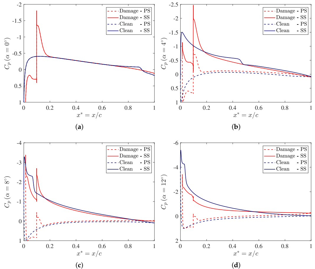
Figure 14. Pressure coefficients comparison between the clean airfoil and the damaged airfoil: the distribution on the Pressure Side (PS) is denoted with the dashed line, while the continuous line is used for the Suction Side (SS) trends. (a) C_p distribution at 0^\circ incidence; (b) C_p distribution at 4^\circ incidence; (c) C_p distribution at 8^\circ incidence; (d) C_p distribution at 12^\circ incidence.
