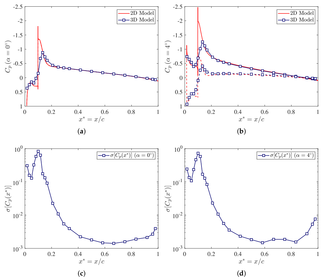
Figure 18. Pressure coefficients comparison between the 2D damaged airfoil and the 3D eroded blade. Distributions on the pressure side are denoted with the dashed line while solid lines are used for suction side trends. Dark blue squares denote the \overline{C_p}(x^*) value over the three-dimensional blade. (a) Pressure coefficients comparison at 0^\circ incidence; (b) Pressure coefficients comparison at 4^\circ incidence; (c) Pressure coefficient standard deviation on the blade at 0^\circ incidence; (d) Pressure coefficient standard deviation on the blade at 4^\circ incidence.
