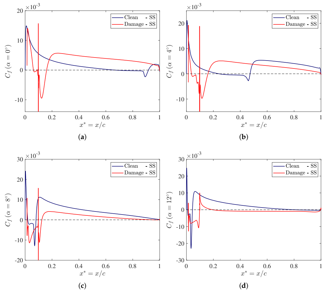
Figure 15. Friction coefficients comparison between the clean airfoil and the damaged airfoil. C_f distribution at (a) 0^\circ incidence; (b) 4^\circ incidence; (c) 8^\circ incidence; (d) 12^\circ incidence.
