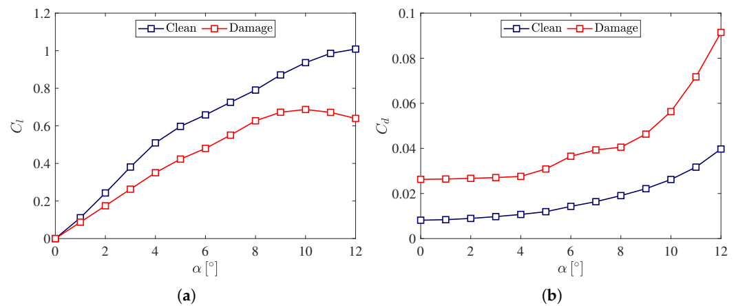
Figure 16. Comparison between polar diagrams of the clean airfoil and the damaged airfoil. (a) C_l polar plot comparison; (b) C_d polar plot comparison.
