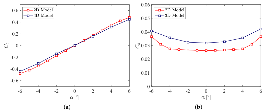
Figure 20. Comparison between polar diagrams of the 2D damaged airfoil and the 3D eroded blade. (a) Comparison of the lift coefficient distribution as a function of the angle of attack; (b) Comparison of the drag coefficient distribution as a function of the angle of attack.
