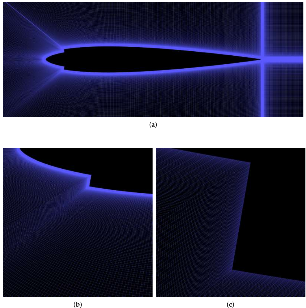
Figure 6. Mesh overview (a) and details (b,c). The figures refer to the fine grid of 500 k elements.
