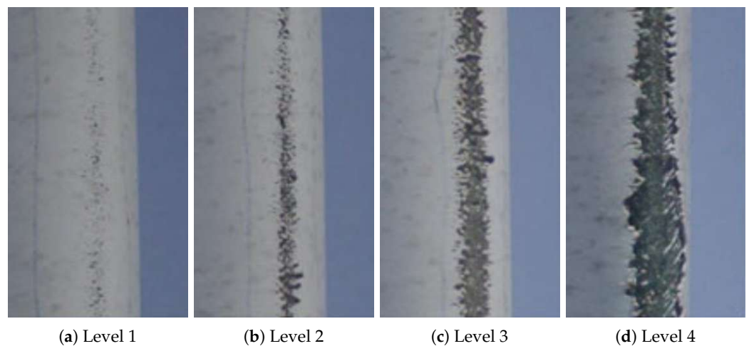
Figure 1. Various levels of erosion from lighter (left) to heavier (right), adapted from [44].
