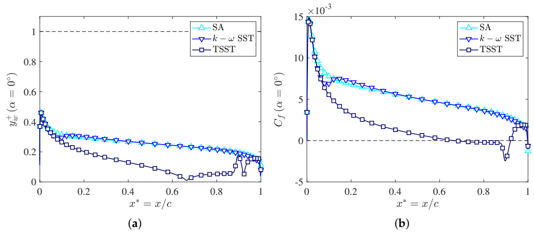
Figure 8. Wall y_w^+ and friction coefficient trends as a function of the turbulence model obtained with the finest grid. (a) y_w^+ distribution on the airfoil surface; (b) C_f distribution on the airfoil surface.
