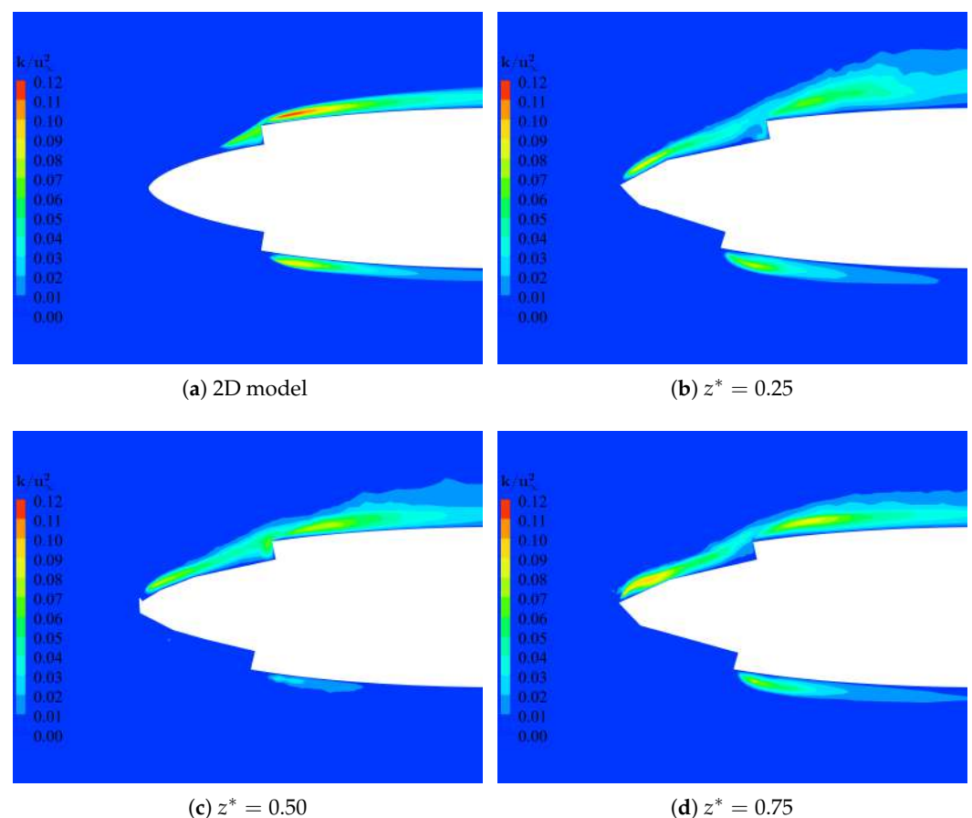
Figure 13. Comparison between contour plots of the non-dimensional turbulent kinetic energy around the 2D airfoil (a) and the 3D blade (b–d) at 4^\circ incidence. (a) Turbulent kinetic energy contour around the two-dimensional airfoil; (b–d) turbulent kinetic energy contour around the three-dimensional blade on a xy plane passing through 1/4 , 1/2 , and 3/4 of the span, respectively.
