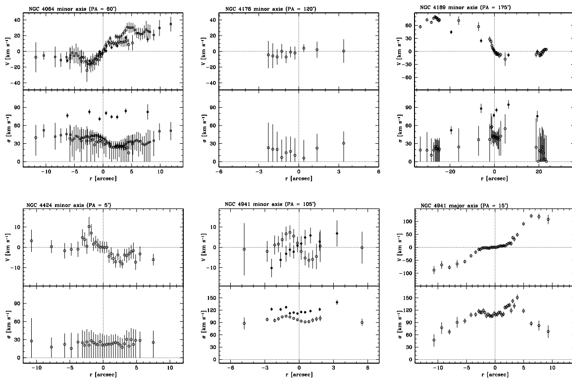
Fig. 1. Ionized-gas ( open symbols ) and stellar ( filled circles ) kinematics measured along the optical minor axis of NGC 4064, NGC 4178, NGC 4189, NGC 4424, and NGC 4941, and the optical major axis of NGC 4941. For NGC 4064, the open circles and open squares refer to gas kinematics obtained in runs 1 and 3, respectively.
