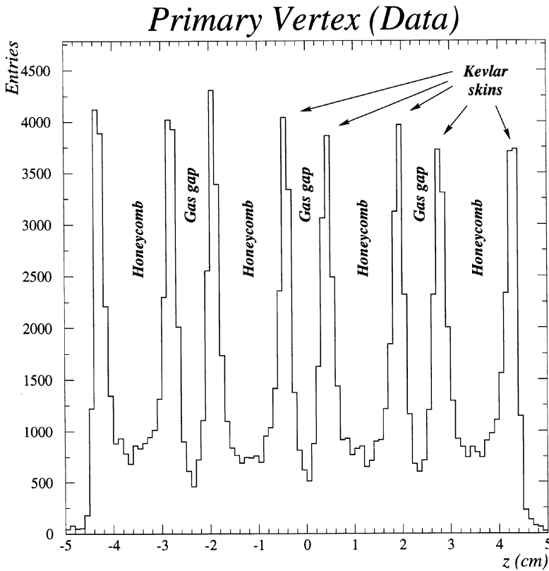
Fig. 11. The positions of reconstructed neutrino interaction vertices as measured along the beam direction; see text.
