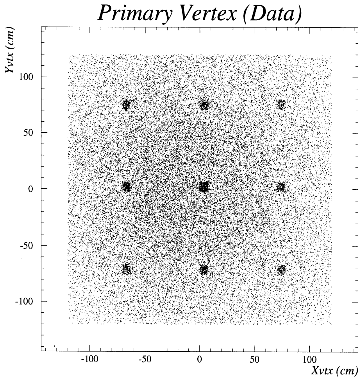
Fig. 10. The positions of reconstructed neutrino interaction vertices in the plane perpendicular to the beam; see text.
