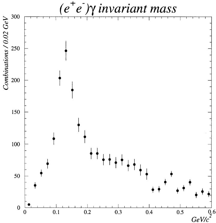
Fig. 29. The \gamma\gamma invariant mass where one \gamma converts in the DC and a second one is measured in ECAL.
