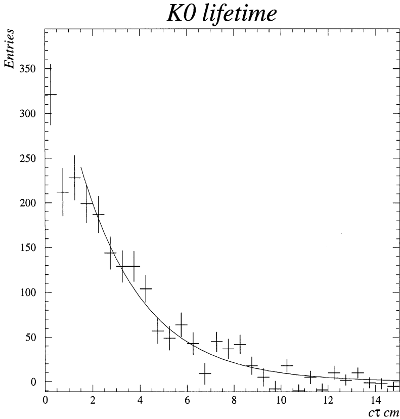
Fig. 27. The product c\tau of K_S^0 mesons observed in NOMAD.
