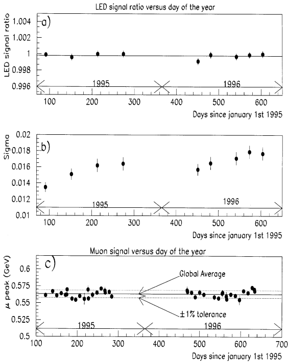
Fig. 16. The signal in ECAL from LED and muon monitoring: (a) LED stability in time over two years of data collection, (b) spread of the ratio of the LED signals to a reference measurement, (c) \mu peak position vs. time over two years of data collection.
