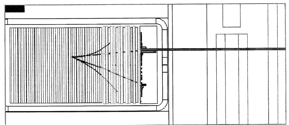
Fig. 25. A candidate \nu_e CC event; see text for details.
