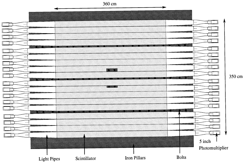
Fig. 18. A front view of the HCAL; see the text for details.
