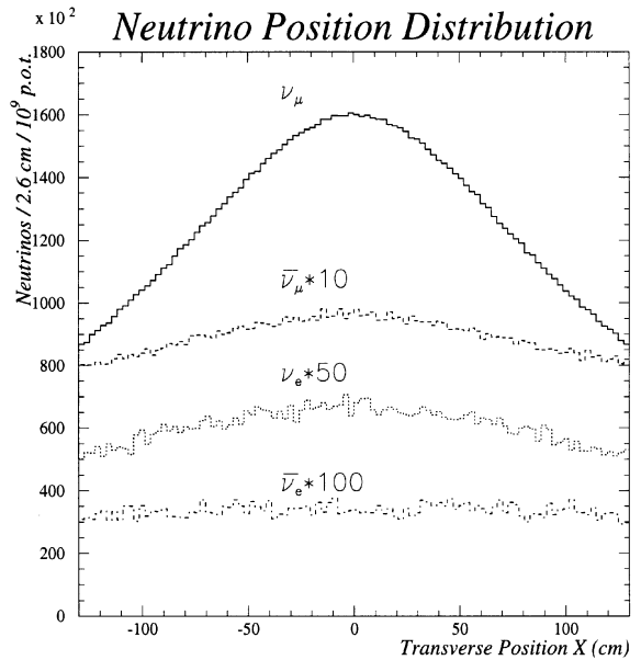
Fig. 5. The predicted transverse position distribution of neutrinos at NOMAD in the horizontal direction. (Due to the beam line symmetry similar spectra are obtained in the other transverse direction.)
