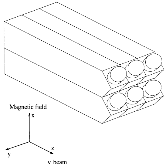
Fig. 15. Schematic view of some lead-glass counters with phototetodes.
