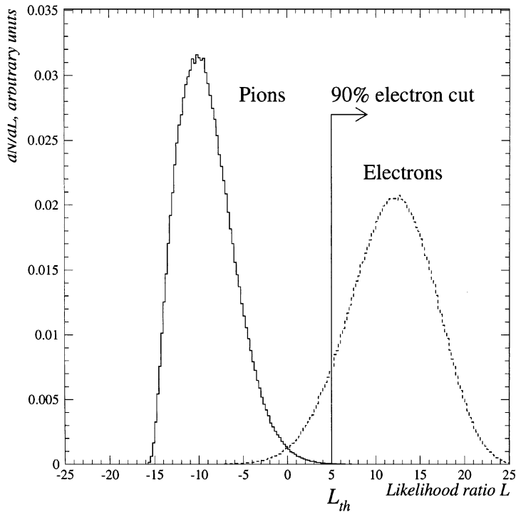
Fig. 31. The likelihood ratio distributions for pions and electrons with track momenta 10 GeV/c crossing nine TRD modules (Monte-Carlo simulation). Pion rejection is better than 1000:1 at 90% electron efficiency.
