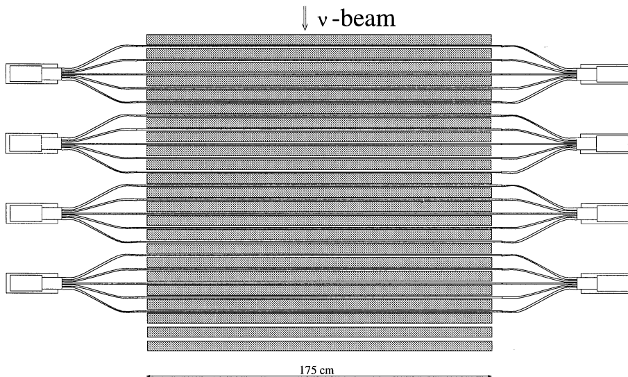
Fig. 6. Top view of the FCAL.
