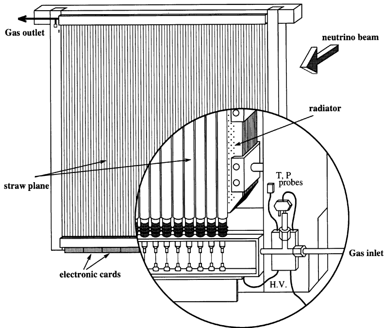
Fig. 12. Schematic view of a TRD module, as seen from the straw plane side.
