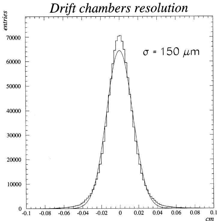
Fig. 8. Residuals for a sample of straight tracks at normal incidence on the drift chambers.
