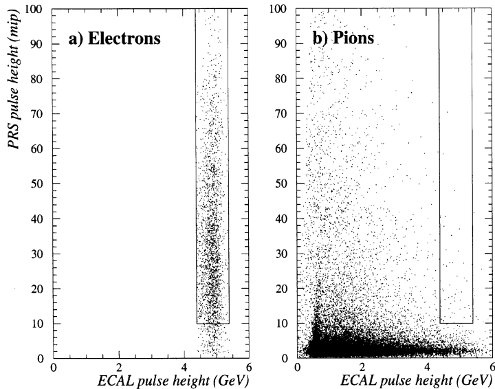
Fig. 32. Scatter plots of the PRS vs ECAL signals for 5 GeV/ c incident electrons (a) and pions (b).
