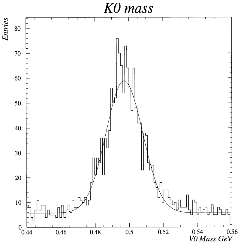
Fig. 26. The invariant mass distribution of (\pi^+\pi^-) pairs from secondary vertices.
