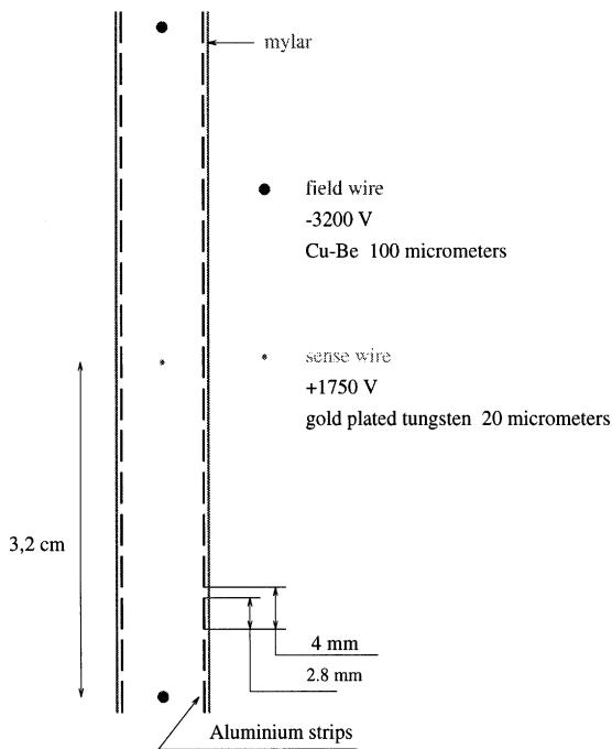
Fig. 7. An overview of the drift chamber layout.
