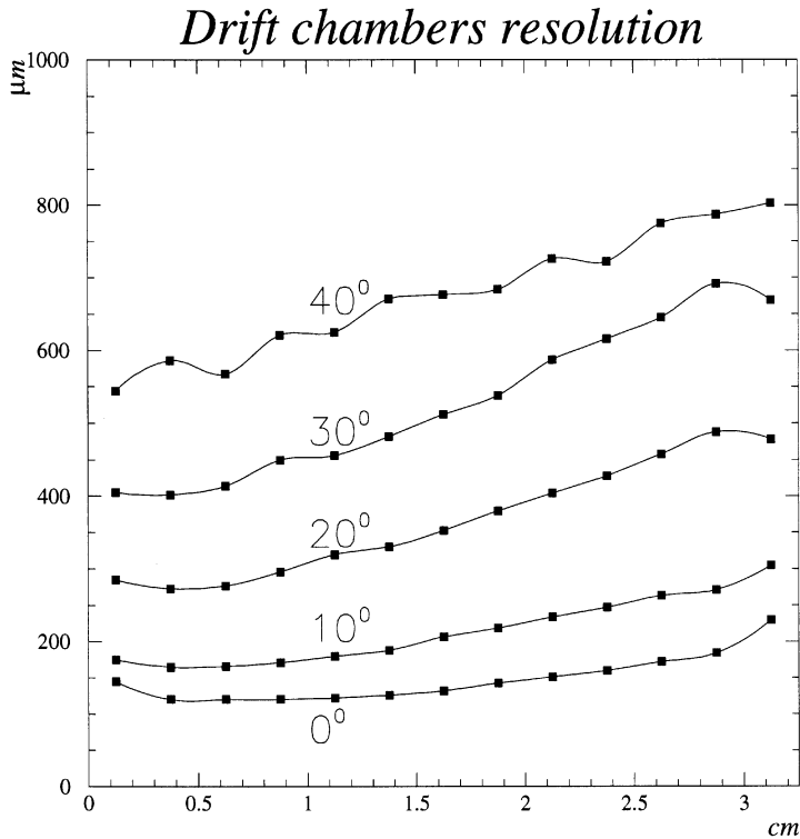
Fig. 9. The dependence of the track residuals on drift distance and angle.
