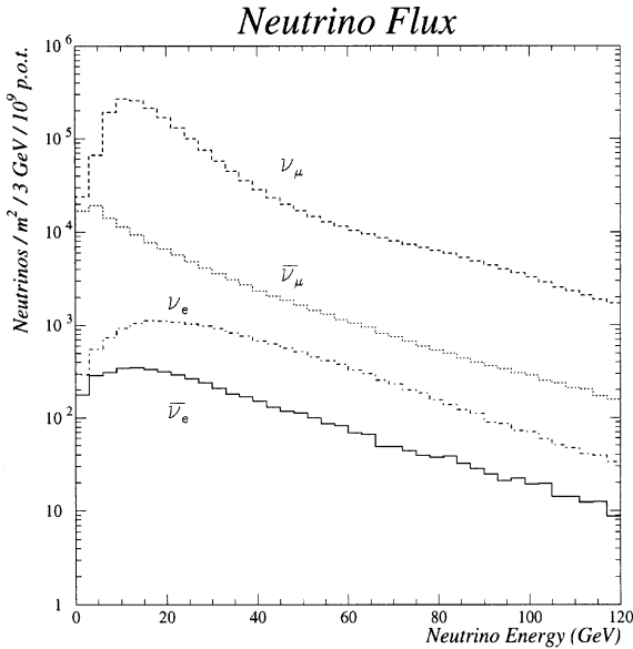
Fig. 4. The predicted energy spectra of neutrinos at NOMAD.
