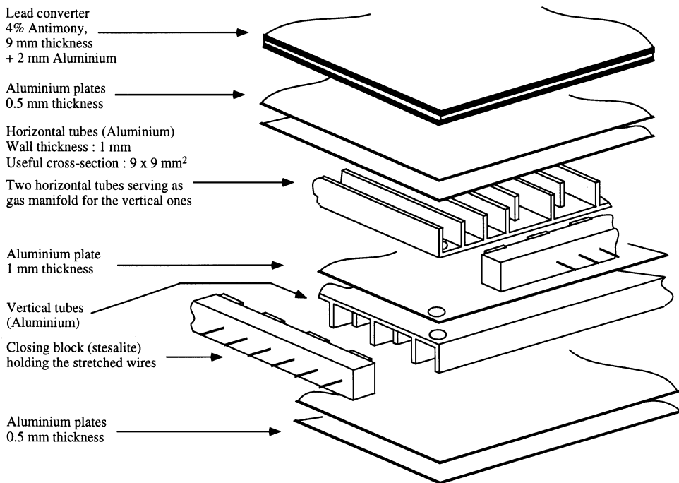
Fig. 14. An exploded view of the preshower.
