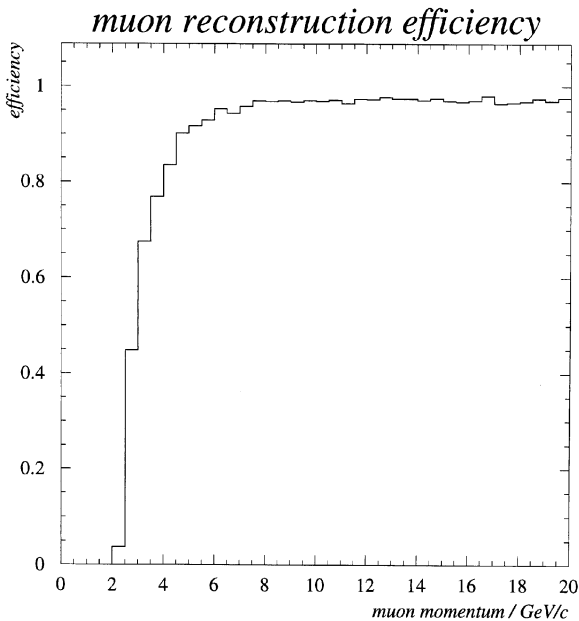
Fig. 30. Typical muon reconstruction efficiency as a function of muon momentum for \nu_\mu CC events. This includes tracking, vertex association, the probability for a muon to emerge from the iron absorbers, the geometrical efficiency and the matching efficiency (multiple scattering).
