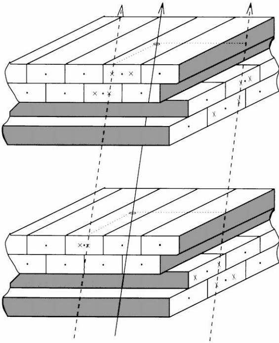
Fig. 21. A cut through a muon chamber module illustrating the drift tube arrangement, and the typical hit pattern left by a throughgoing muon (continuous arrow) and the track segment reconstructed in projection (dashed arrows).
