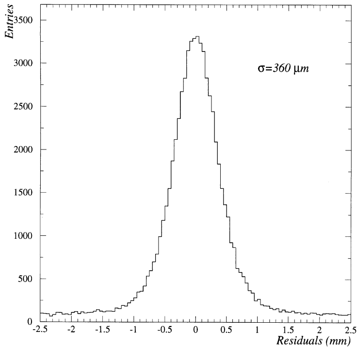
Fig. 22. Residuals for 4-point tracks in the muon chambers for a typical run.
