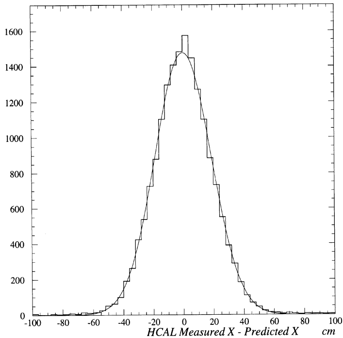
Fig. 20. Horizontal position resolution for muons passing through a single hadron calorimeter module.
