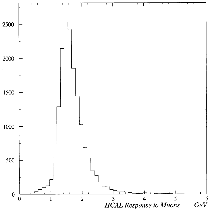
Fig. 19. Minimum ionizing peak for muons passing through the hadron calorimeter.
