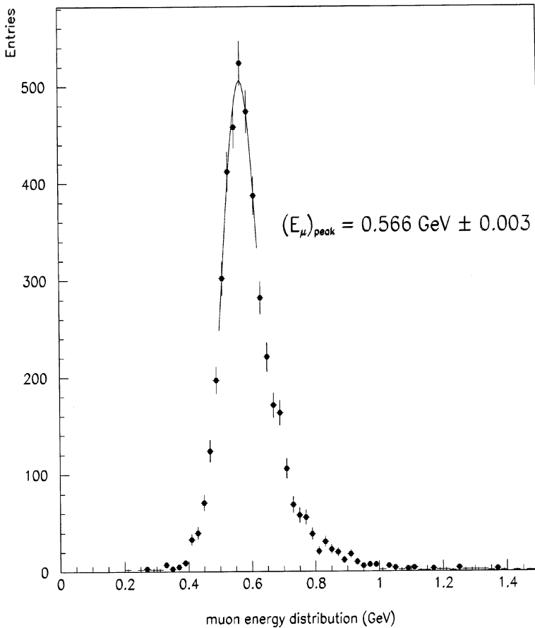
Fig. 17. The signal in ECAL from muons crossing the detector during normal data taking. A correction has been applied to account for the differences in impact angle of the muons on the detector.
