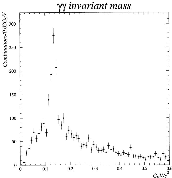
Fig. 28. The \gamma\gamma invariant mass where both \gamma energies are measured in ECAL.
