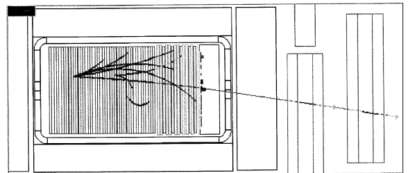
Fig. 24. A candidate \nu_\mu CC event see text for details.
