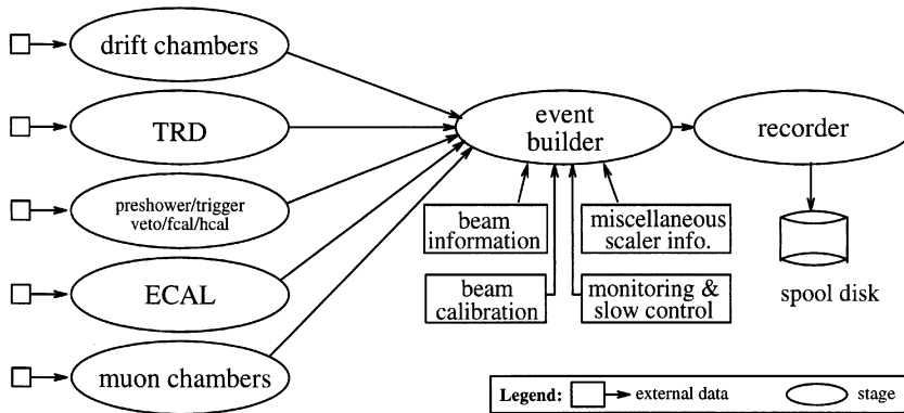
Fig. 23. Data-acquisition software configuration.
