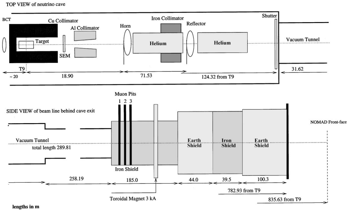
Fig. 3. Schematic layout of the WANF beam line pointing out its main elements. Not drawn to scale. See the text for further explanation.
