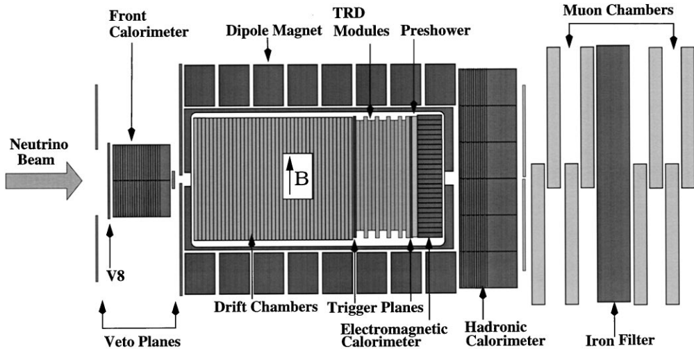
Fig. 2. A topview of the NOMAD detector.
