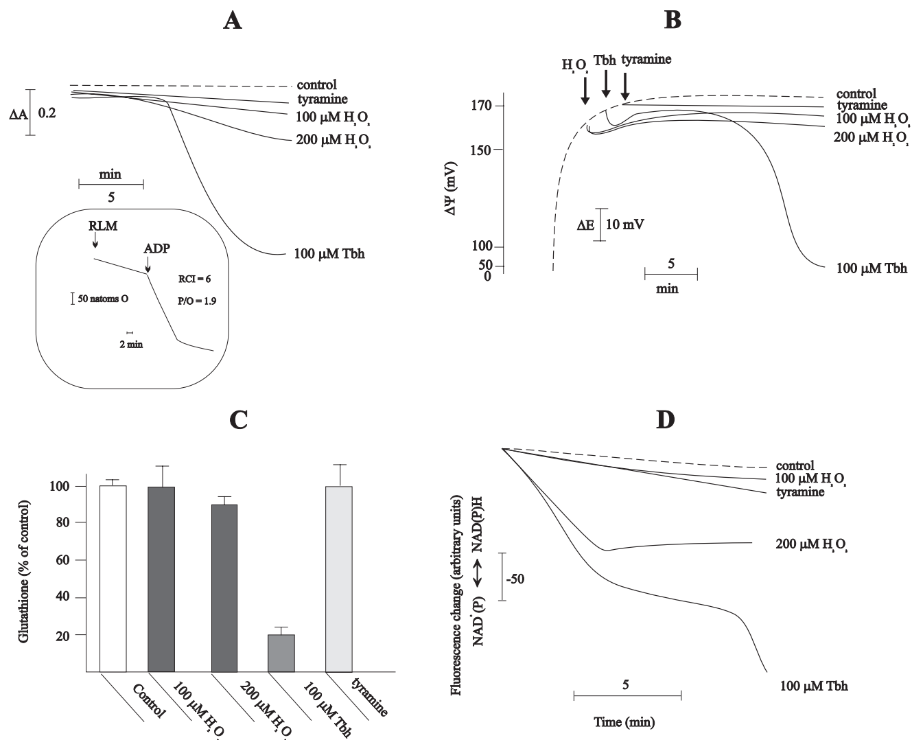
FIGURE 1. Comparisons of effects of Tbh, H 2 O 2 , and tyramine in inducing membrane permeabilization (panels A and B) and oxidative stress (panels C and D) associated with MPT induction. RLM were incubated in standard medium supplemented with 50 \mu\text{M} Ca 2+ in conditions indicated under "Experimental Procedures." Tbh, H 2 O 2 , and tyramine were added at concentrations indicated. A , mitochondrial swelling. Downward deflection indicates mitochondrial swelling. B , membrane potential. \Delta E = electrode potential. C , mitochondrial glutathione content. Glutathione content was measured after 15 min of incubation. D , pyridine nucleotide oxidation. Downward deflection indicates pyridine nucleotide oxidation. Inset , calculation of the respiratory control index and ADP/O. RLM were incubated in standard medium with 1 mM phosphate. Addition of 0.3 mM ADP. Assays in panels A , B , and D were performed four times with comparable results. Panel C , mean values \pm S.D. of four experiments.
