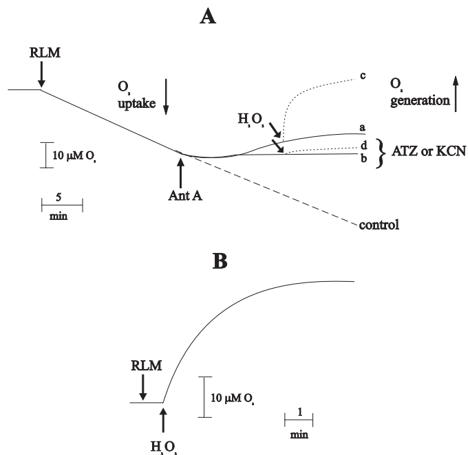
FIGURE 2. Oxygen generation from endogenous or added H 2 O 2 in isolated RLM. Panel A, effect of treatment with antimycin A and ATZ or KCN (both in presence of antimycin A). RLM were incubated in standard medium, as described under "Experimental Procedures." When present in medium, ATZ and KCN were 10 μM and 200 μM, respectively. 1 μM antimycin A (Ant. A) and 50 μM H 2 O 2 were added (see arrows). Trace a, antimycin A; trace b, ATZ or KCN plus antimycin A; trace c, antimycin A plus H 2 O 2 ; trace d, ATZ or KCN plus antimycin A plus H 2 O 2 . Assays were performed three times with comparable results. Panel B, effect of exogenous H 2 O 2 . RLM were incubated in standard medium, deprived of succinate, in same conditions as in panel A. 50 μM H 2 O 2 were added where indicated.
