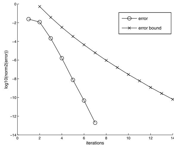
FIG. 5.5. Error and error bound for the rational Arnoldi method applied to (5.2) with \alpha = 0.5 , t = 1 , h = 0.4 .
