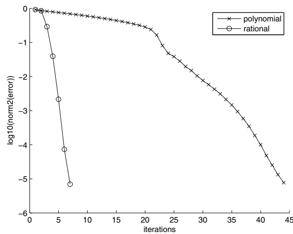
FIG. 5.3. Approximation of (5.3) at t = 0.1 with \alpha = 0.5 .
