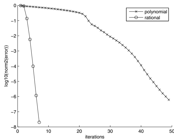
FIG. 5.4. Approximation of (5.3) at t = 1 with \alpha = 0.5 .
