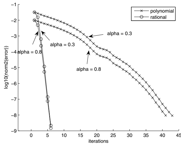
FIG. 5.2. Approximation of (5.2) at t = 1 .
