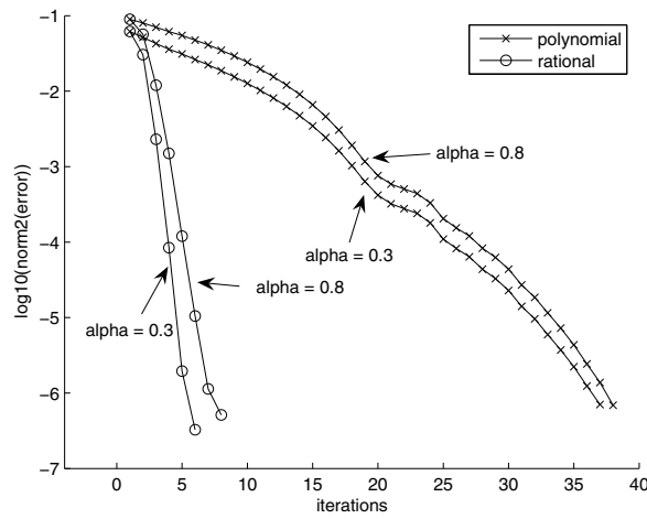
FIG. 5.1. Approximation of (5.2) at t = 0.1 .
