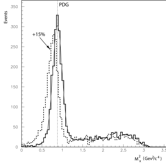
Figure 2. Missing mass in 3 GeV/c pp scattering. The result (solid line) is centered very close to the PDG value of the squared proton mass. An artificial shift of 15% of the momentum measured was applied to obtain the dashed histogram. Such a shift is clearly excluded by the data (see the text).
