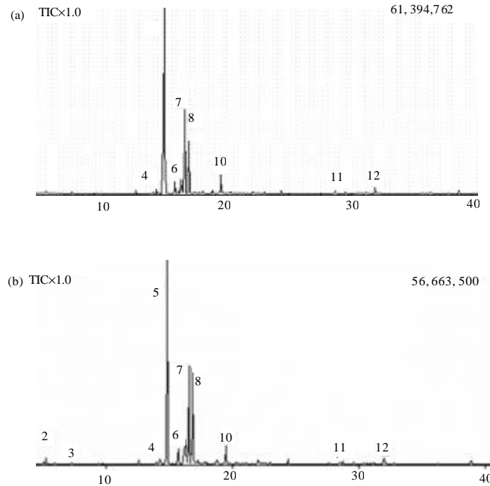
Fig. 1 (a-b): Chromatogram of total ions in essential oil of jambu ( Spilanthes oleracea cv. Jambuarana) inflorescence, cultivated under (a) Mineral manuring and (b) Organic, Peaks 5, 7, 8 and 10 are trans-caryophyllene, germacrene-D, 1-dodecene and spathulenol, respectively
