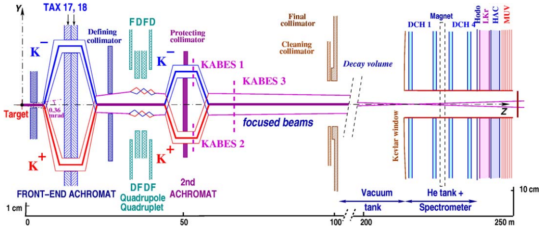
Fig. 1. Schematic lateral view of the NA48/2 experiment. Region 1 (from target to decay volume): beam line (TAX17, 18: motorized beam dump/collimators used to select the momentum of the K^+ and K^- beams; DFDF: focusing quadrupoles; KABES1-3: beam spectrometer stations). Region 2: decay volume and detector (DCH1-4: drift chambers; Hodo: hodoscope; LKr: electromagnetic calorimeter; HAC: hadron calorimeter; MUV: muon veto). The vertical scales for the two regions are different.
