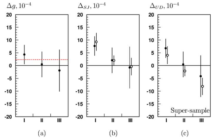
Fig. 5. (a) Slope difference \Delta g for each super-sample. The horizontal dashed line represents the weighted average of the three results, (b) Left–right instrumental asymmetry and (c) up–down instrumental asymmetry for experimental data (full circles) and Monte Carlo events (open circles) (these instrumental asymmetries cancel in the quadrupole ratio (6)).
