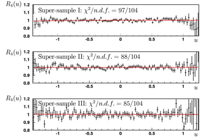
Fig. 4. Fits of the normalized quadrupole ratios for each super-sample.
