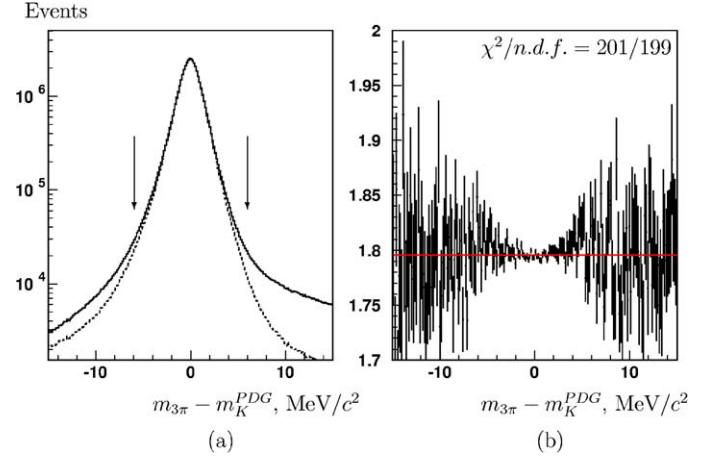
Fig. 2. (a) Difference between the invariant \pi^\pm \pi^0 \pi^0 mass and the PDG kaon mass [11]. The selected interval is indicated by the arrows. The dashed histogram shows the same distribution for events with no hit in the muon detector. (b) Ratio of invariant mass distributions for \pi^+ \pi^0 \pi^0 and \pi^- \pi^0 \pi^0 fitted with a constant function.
