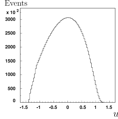
Fig. 3. u -spectrum for the selected events.
