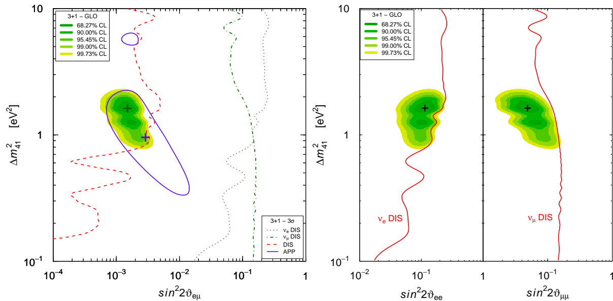
Figure 1. Allowed regions in the \sin^2 2\theta_{e\mu}-\Delta m_{41}^2 , \sin^2 2\theta_{ee}-\Delta m_{41}^2 and \sin^2 2\theta_{\mu\mu}-\Delta m_{41}^2 planes obtained in the global (GLO) 3+1-HIG fit [65] of short-baseline neutrino oscillation data compared with the 3\sigma allowed regions obtained from \bar{\nu}_{\mu} \rightarrow \bar{\nu}_e short-baseline appearance data (APP) and the 3\sigma constraints obtained from \bar{\nu}_e short-baseline disappearance data ( \nu_e DIS), \bar{\nu}_{\mu} short-baseline disappearance data ( \nu_{\mu} DIS) and the combined short-baseline disappearance data (DIS). The best-fit points of the GLO and APP fits are indicated by crosses.
