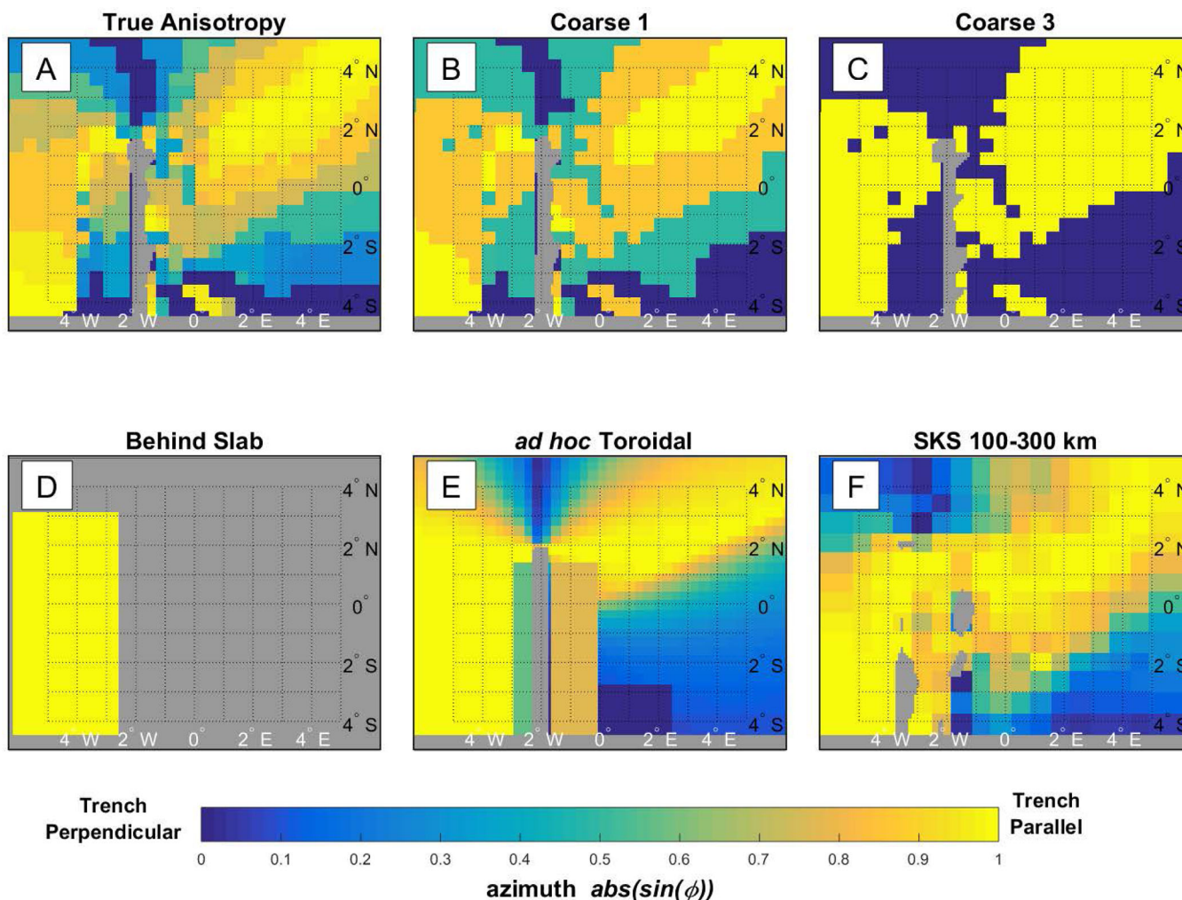
Figure 9. Azimuth distribution for six different anisotropy models used as a priori constraints on the tomographic inversions. Model names are indicated above each plot. All plots represent depth slices at 195 km depth.
