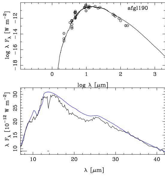
Fig. B.1. Fits to the SED and mid-IR spectrum of Galactic extreme C stars.
