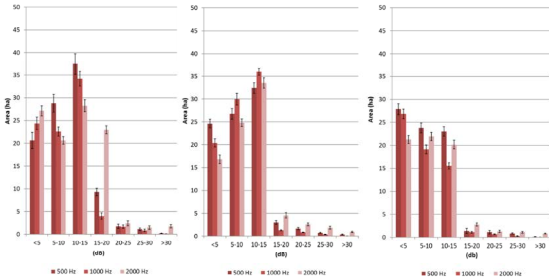
Fig. 3. Excess noise exposed area for (a) Felling, (b) Skidding and (c) Cable yarder scenarios.
