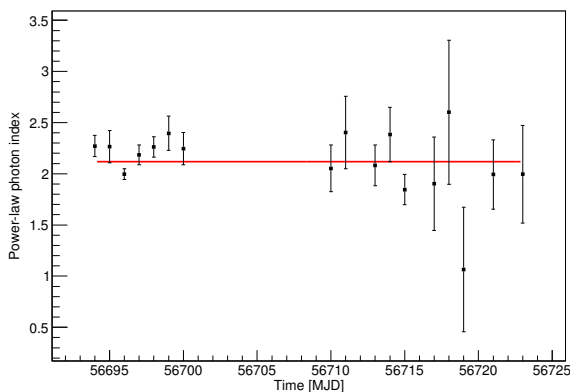
Fig. 3. Evolution of the photon index from power-law fits to the de-absorbed night-wise spectra of 1ES 1011+496 between February 6 and March 7 2014. The error bars are the parameter uncertainties from the fits. The red line represents the fit to a constant value, for which the probability is 10%.
