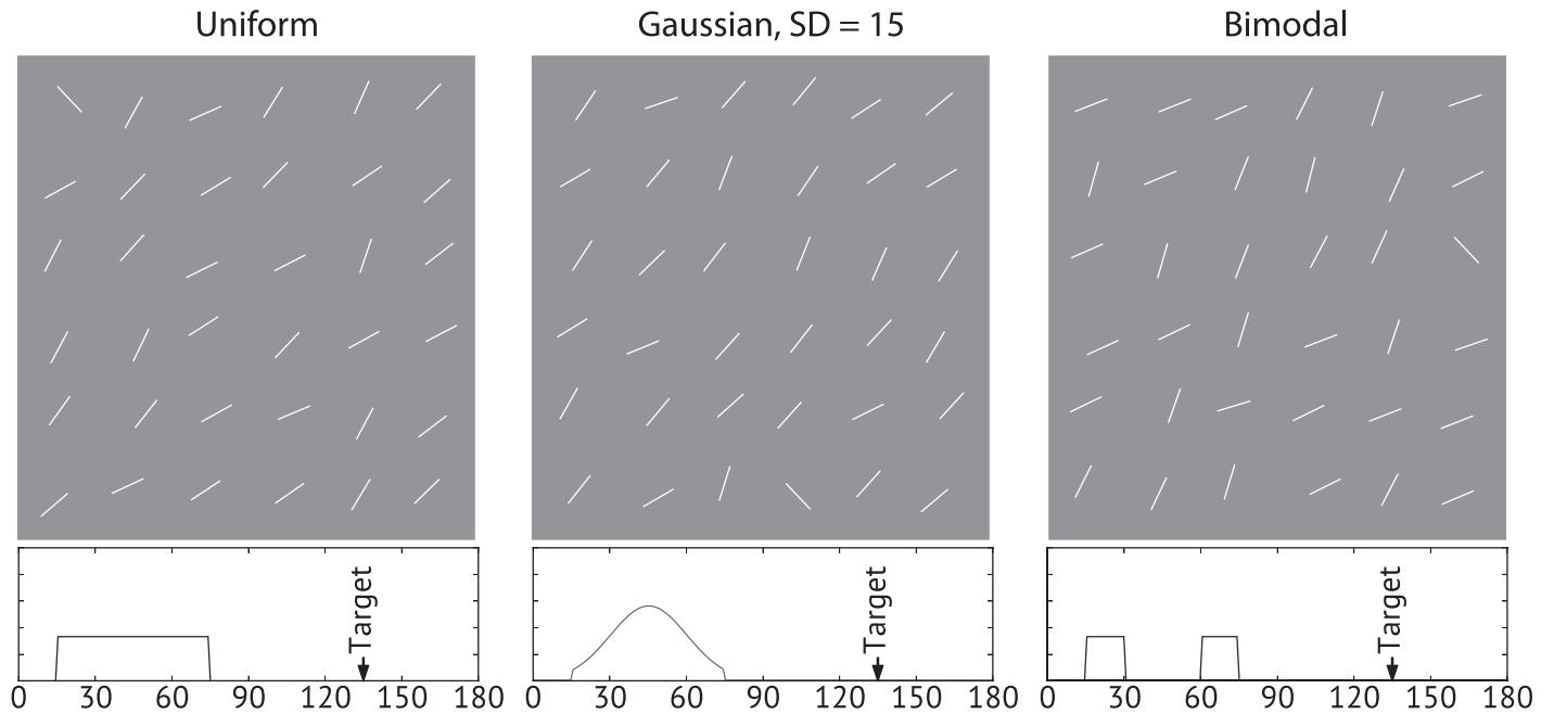
Figure 2. Example prime distributions in Experiments 1, 2, and 3. The top row shows example stimuli, and the bottom row shows corresponding probability density functions of distractor distributions and target position in feature space.
