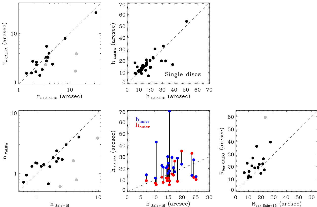
Fig. 13. Comparison of our r -band best-fit parameters with those from the multi-component photometric decompositions of the 3.6\mu\text{m} images of the \text{S}^4\text{G} galaxies (Salo et al. 2015). There are 65 galaxies in common between our sample and \text{S}^4\text{G} . Left panels correspond to elliptical/bulge parameters: effective radius ( top ) and Sérsic index ( bottom ). Controversial bulges (see text) are plotted as grey dots. Middle panels compare the disc scale lengths for single discs ( top ) and truncated discs as classified by this work ( bottom ). Salo et al. (2015) only include single discs in their decompositions. Inner and outer disc scale lengths are distinguished in the case of breaks as blue and red dots, respectively. For the sake of clarity, the 1:1 axis proportion in the bottom panel has not been kept. The right panel shows the comparison of the bar lengths for the 19 galaxies classified as barred by both works. The use of two different disc components (an exponential and Ferrers) in the \text{S}^4\text{G} fit explain the difference for NGC 5957 (grey dot).
