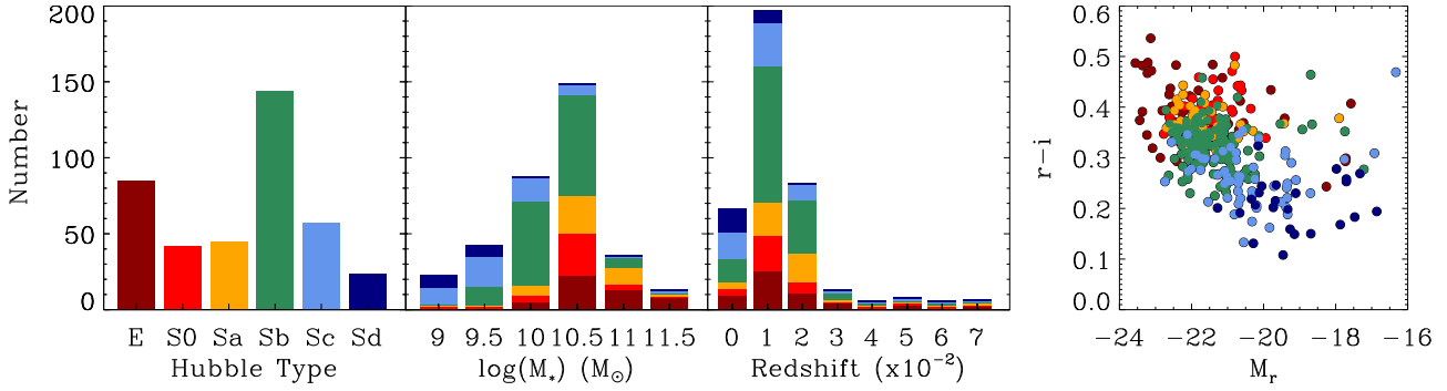
Fig. 1. (From left to right) Distribution of our galaxy sample in Hubble type, stellar mass, redshift, and on the r - i vs. r -band colour magnitude relation. Colours in all panels represent the different galaxy Hubble types. The parameters for each galaxy were obtained from Walcher et al. (2014).
