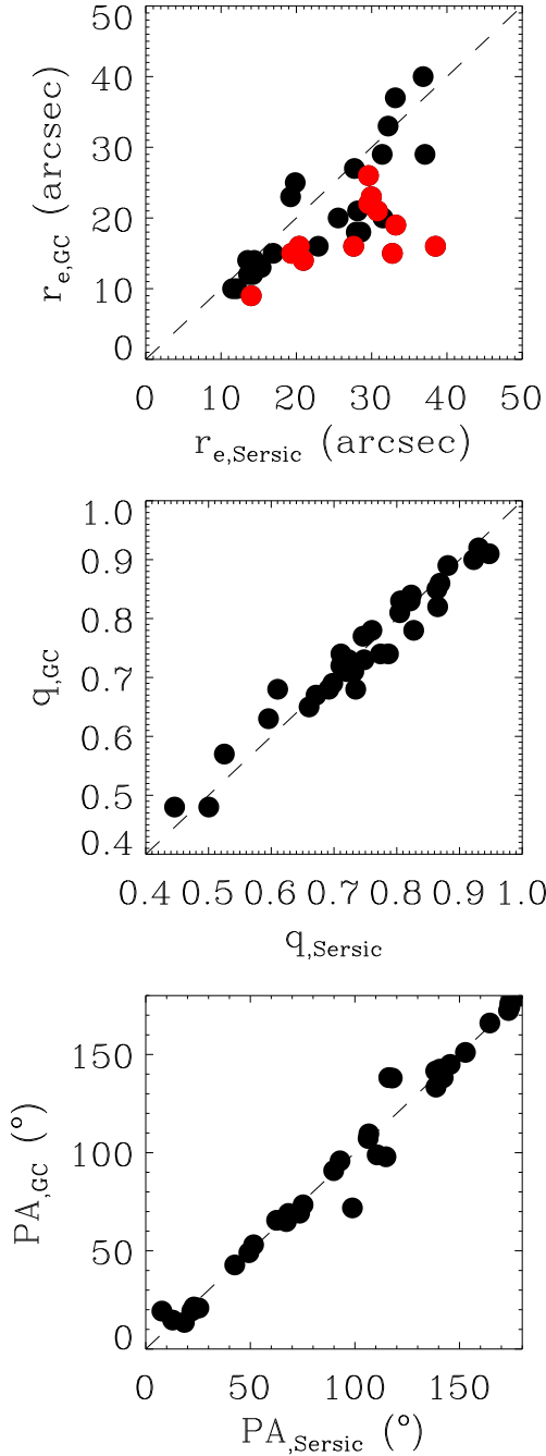
Fig. 11. Comparison of our photometric decomposition r -band estimated parameters (labelled as Sérsic) with those obtained from the growth curves (labelled as GC) in Walcher et al. (2014). Only those galaxies fitted with a single Sérsic profile have been used in this comparison. From top to bottom, panels show the galaxy effective radius, axis ratio, and position angle, respectively. Red points in the upper panel represent galaxies fitted with a single Sérsic with n > 5.5 .
