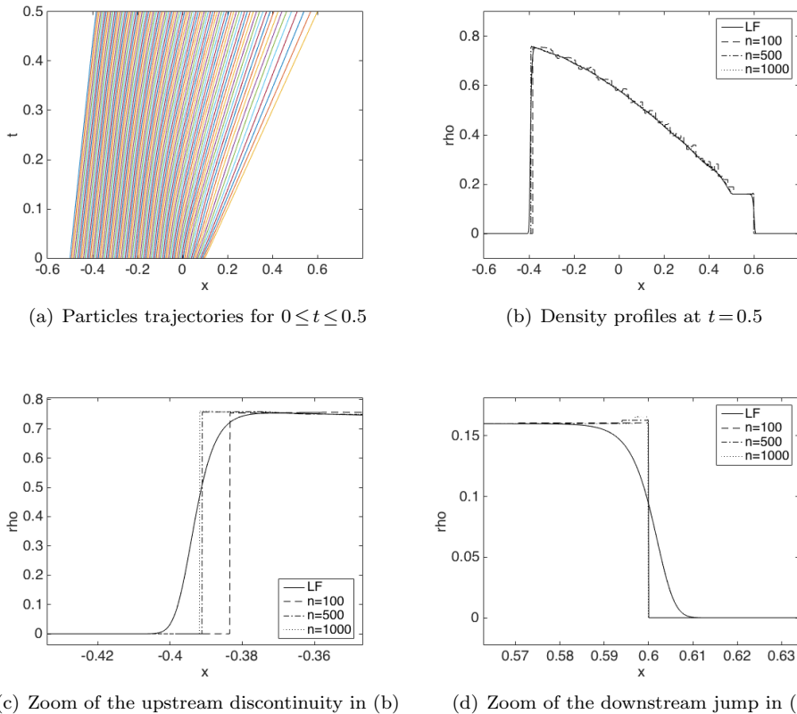
FIG. 4.1. Approximate solutions \hat{\rho}_n to (1.1), (4.19) with kernel w_\eta(x) = 1/\eta obtained by the particle method with n = 100, 500 and 1000 particles, and the corresponding Lax-Friedrichs approximation for \Delta x = 0.0002 .
