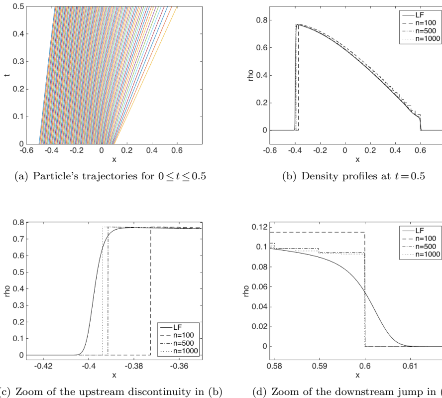
FIG. 4.2. Approximate solutions \hat{\rho}_n to (1.1), (4.19) with kernel w = 2(\eta - x)/\eta^2 obtained by the particle method with n = 100, 500 and 1000 particles, and the corresponding Lax-Friedrichs approximation for \Delta x = 0.0002 .
