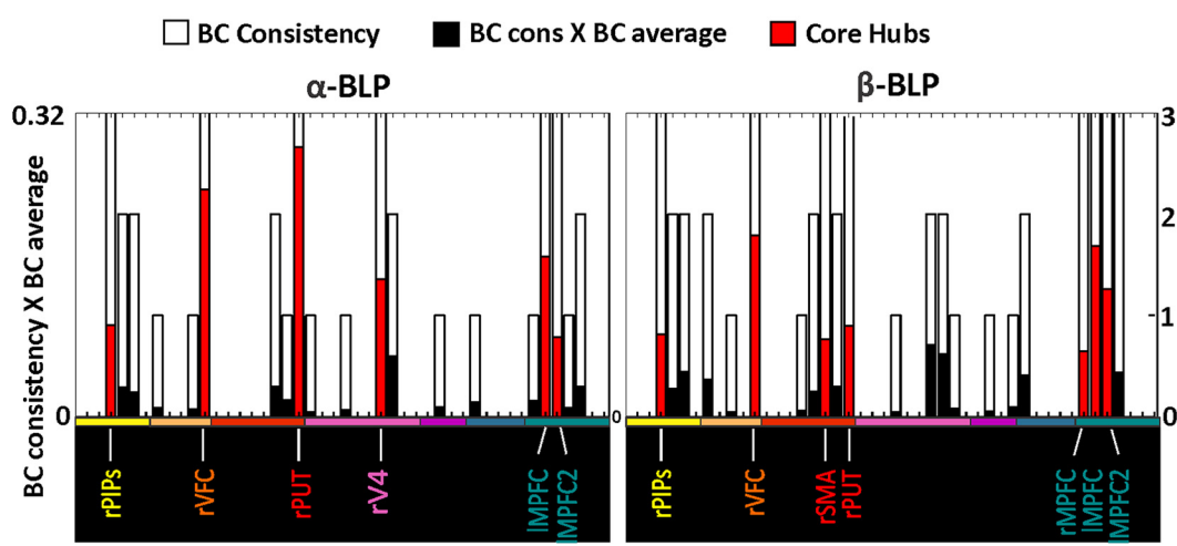
Figure 5. Measures of BC during rest and movie viewing. A , BC values in \alpha -BLP and \beta -BLP for fixation (cyan), movie (magenta), and scrambled (green). These values are compared with the averaged BC obtained from a set of equivalent random graphs (solid lines). The patterns of node centrality vary between the \alpha and \beta band. B , BC consistency (right y-axis, white bars) in each band defined as the number of times across the three experimental conditions in which the BC in each node exceeds the random graph BC threshold. The product BC consistency \times BC values averaged across the three conditions (left y-axis, black bars) provides a core network for each band, defined as a group of nodes with consistently high centrality (red bars). C , For each band, the spatial location of the hubs form the core network.
