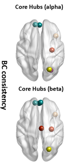
Figure 5. Measures of BC during rest and movie viewing. A , BC values in \alpha -BLP and \beta -BLP for fixation (cyan), movie (magenta), and scrambled (green). These values are compared with the averaged BC obtained from a set of equivalent random graphs (solid lines). The patterns of node centrality vary between the \alpha and \beta band. B , BC consistency (right y-axis, white bars) in each band defined as the number of times across the three experimental conditions in which the BC in each node exceeds the random graph BC threshold. The product BC consistency \times BC values averaged across the three conditions (left y-axis, black bars) provides a core network for each band, defined as a group of nodes with consistently high centrality (red bars). C , For each band, the spatial location of the hubs form the core network.
