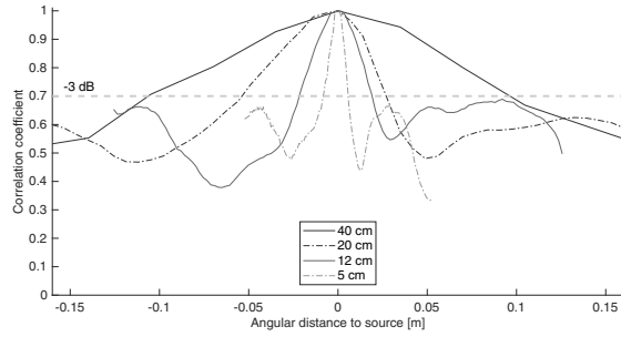
Figure 3: Normalized focusing functions along the curvilinear abscissa for sources in front of the center of the skull ( \varphi = 0^\circ ) and at different distances to the skull. The distance of the measurement points to the skull decreases from 40 cm, down to 20 cm, 12 cm and 5 cm (different curves). There is a clear trend of increasing resolution (decreasing -3 dB width of the curves) with decreasing distance.
