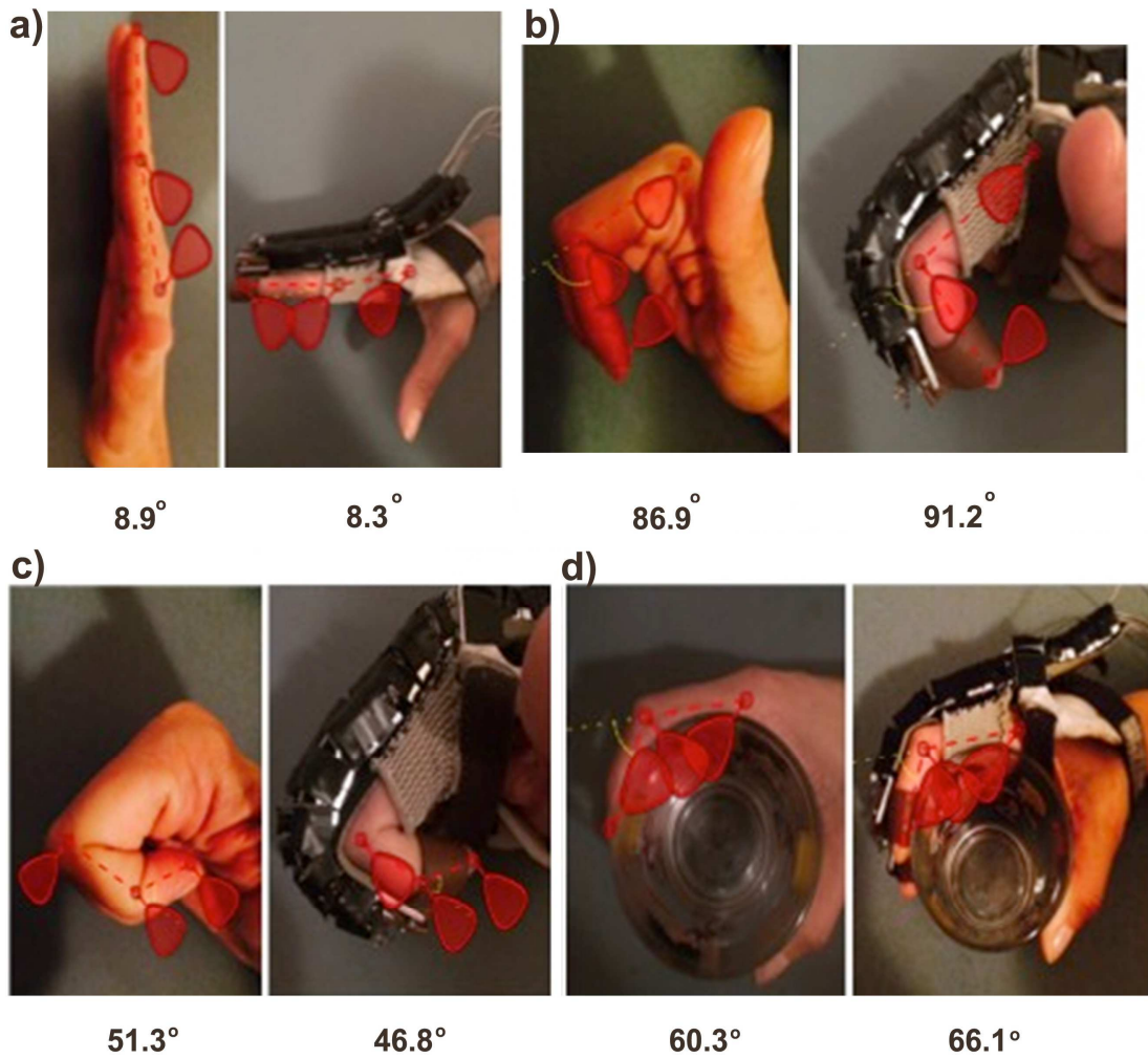
Fig.8 - Range of motions for bare fingers in comparison to fingers equipped with FEX device: a) straight fingers configuration, b) proximal interphalangeal maximum configuration angle, c) distal interphalangeal maximum configuration angle, d) exemplary power grasp.
