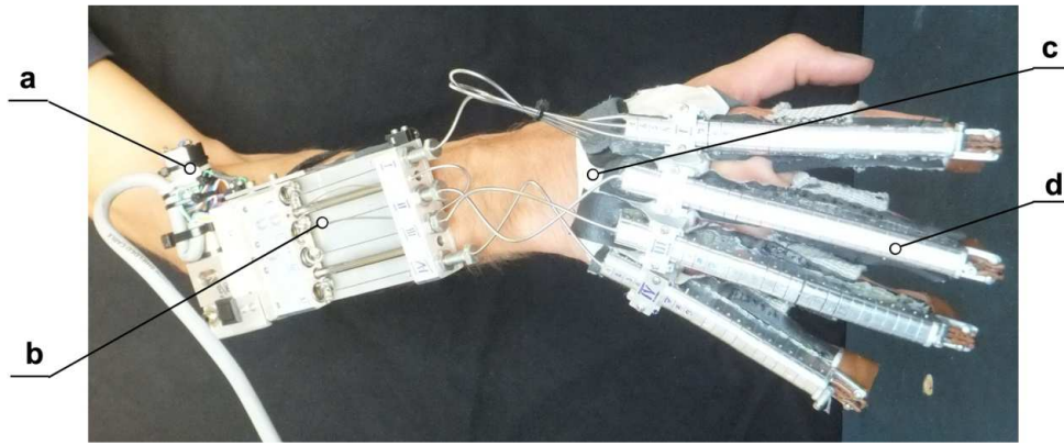
Fig.7 FEX device - a) motor, b) wires tensioning unit, c) palm mounting plate, d) pulling chains
