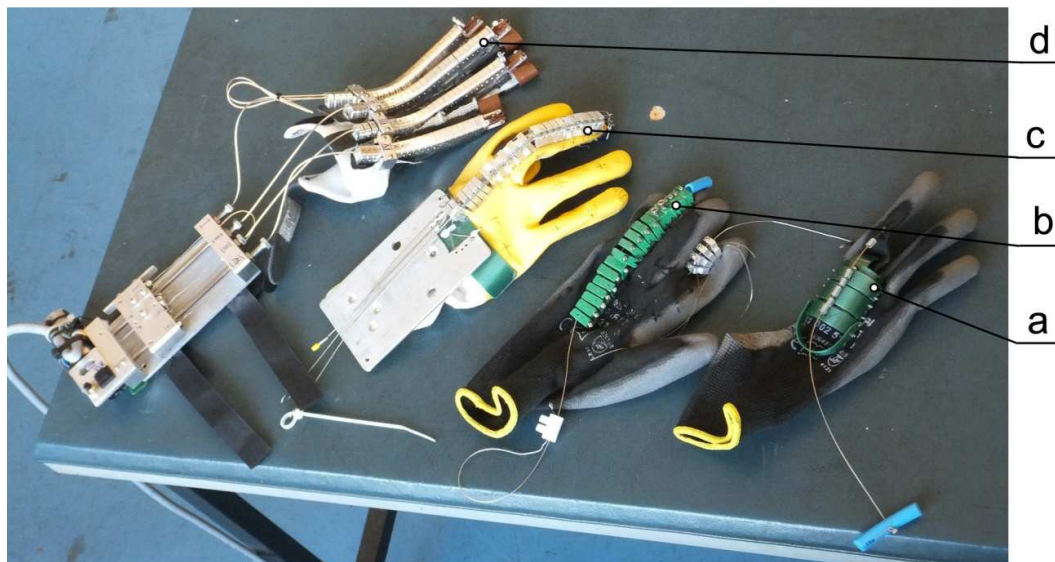
Fig.2 Consecutive FEX device designs - a) first prototype, b) and c) intermediate prototypes, d) latest design
