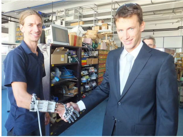
Fig.9 - FEX device tested for being possible to wear even during very complex tasks like handshake and to be able to force open semi-closed fingers (left), FEX device with markers glued onto (right).
