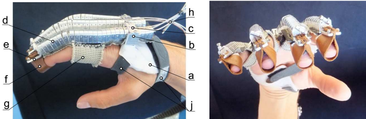
Fig.5 FEX worn on a hand - side view (left), front view (right)
