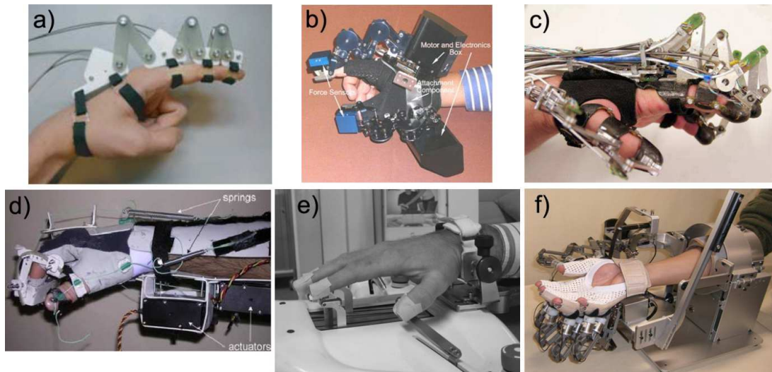
Fig.1 Various hand rehabilitation devices: a) The University of Tokyo Hand [11], b) Percro Hand [12], c) Berlin University Hand [13], d) Milan University Hand [14], e) Amadeo [15], f) Gifu University Hand [16]
