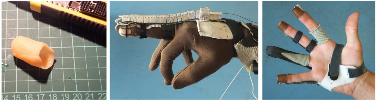
Fig.4 Finger tip cast (left), semi-rigid finger-tip mounting (center), various finger attachment schemes (right)
