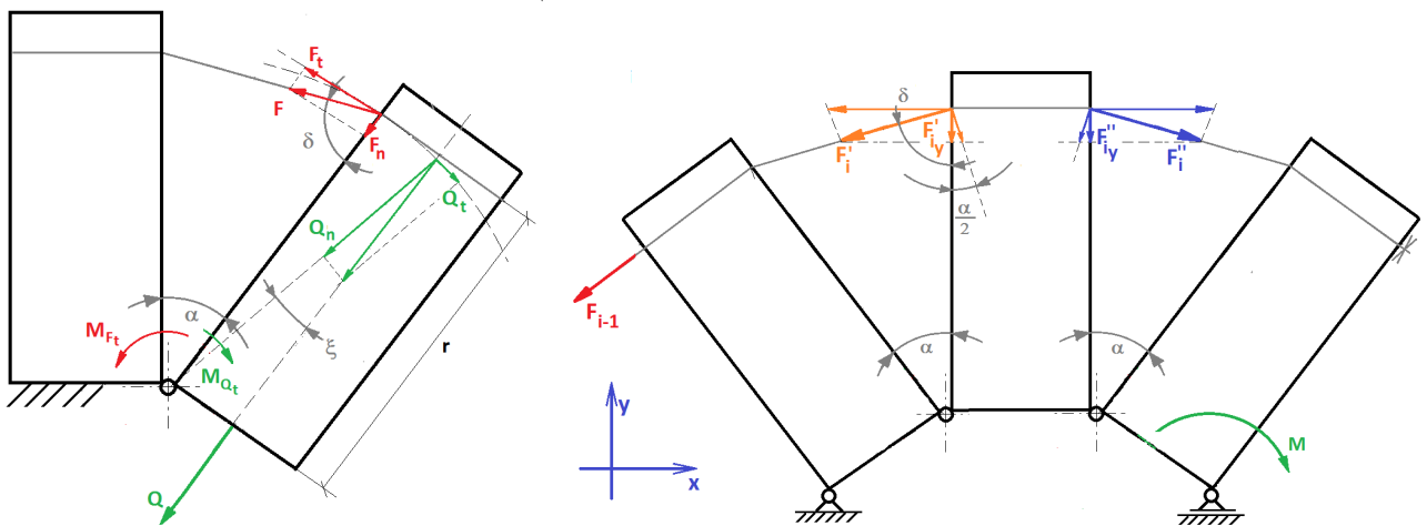
Fig.6 FEX structure working principles - last block case (left) and the amid block case (right)
