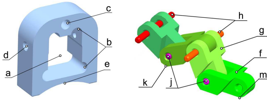
Fig.3 Subcomponents of the FEX - cuboid block (left) and the Fingerspine structure (right)
