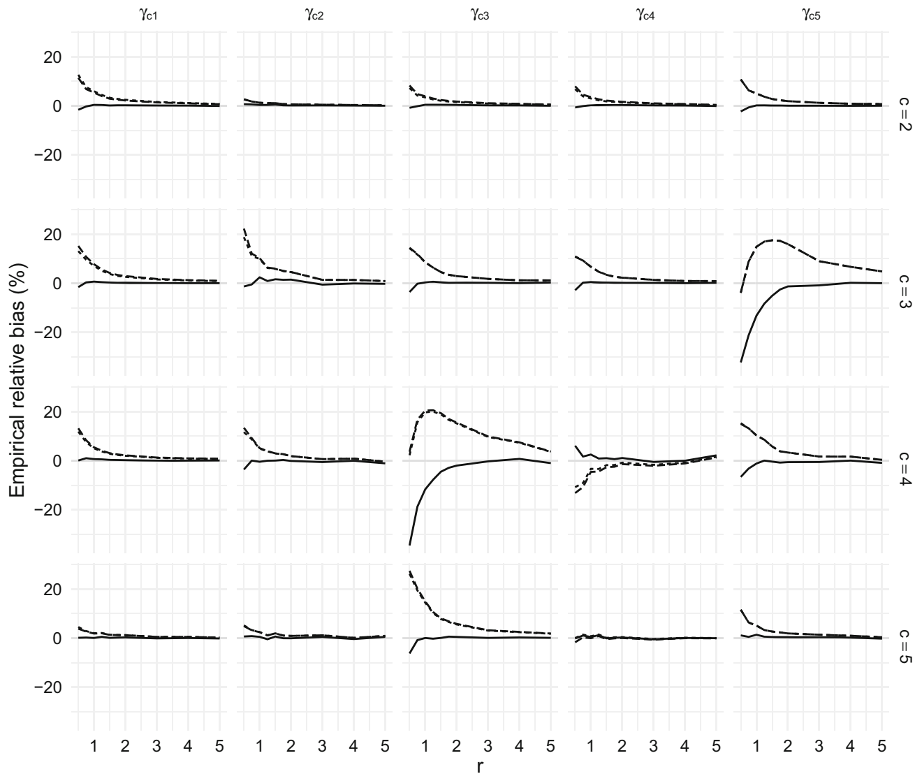
Fig. 3 Empirical relative bias based on 10,000 simulated samples from the ML fit of model (15) given in Table 10, for each r \in \{0.5, 0.75, 1, 1.25, 1.5, 1.75, 2, 3, 4, 5\} . The curves correspond to the
