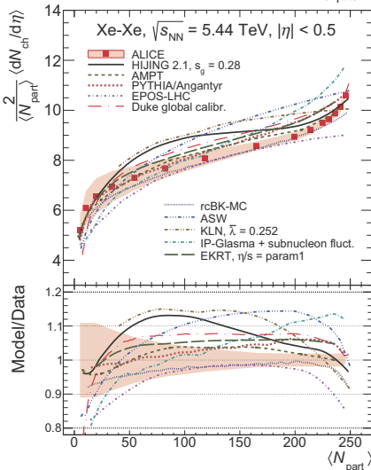
(c) The \frac{2}{\langle N_{part} \rangle} \langle dN_{ch}/d\eta \rangle vs \langle N_{part} \rangle in Xe–Xe collisions [13]
